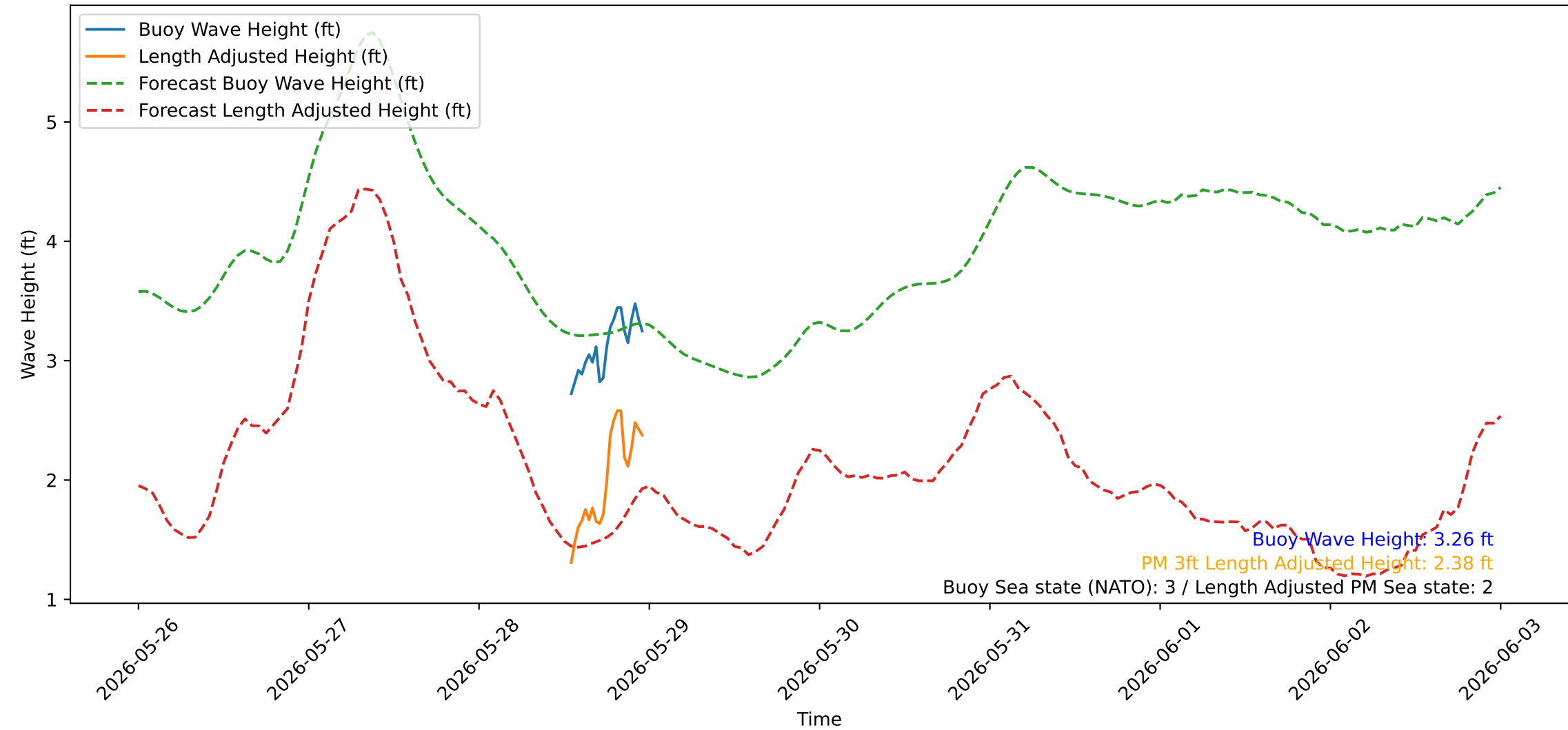
Wave Heights over Time for Oceanside Harbor at 2026-05-28 23:50:21
