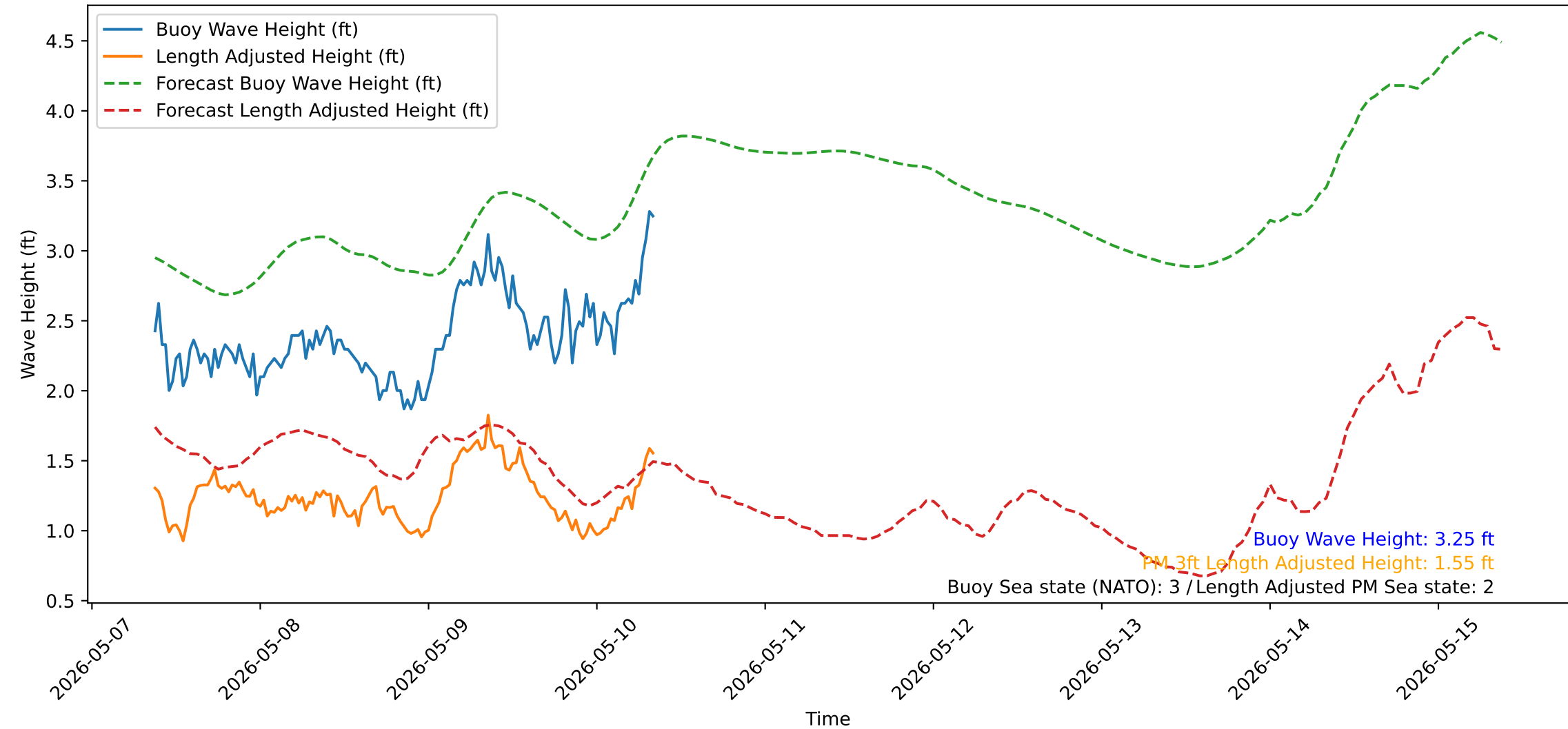
Wave Heights over Time for Oceanside Harbor at 2026-05-10 08:50:31
