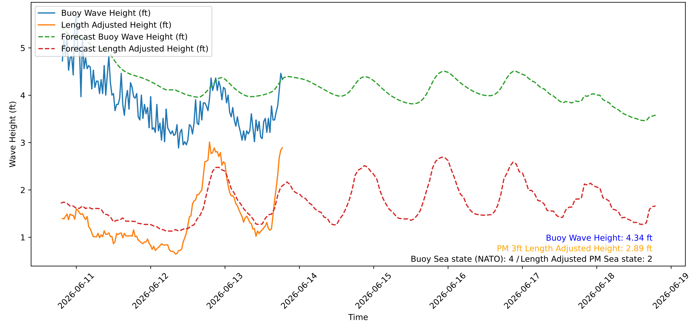
Wave Heights over Time for Green Beach at 2026-06-13 19:21:10
