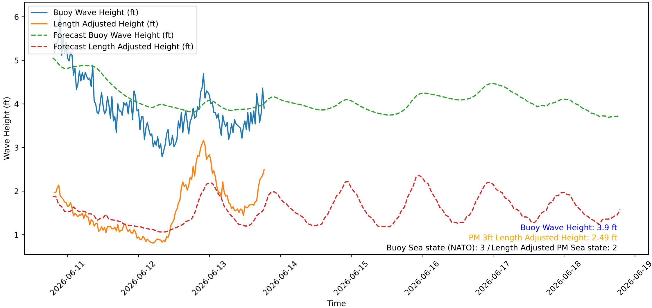
Wave Heights over Time for Oceanside Harbor at 2026-06-13 19:20:26
