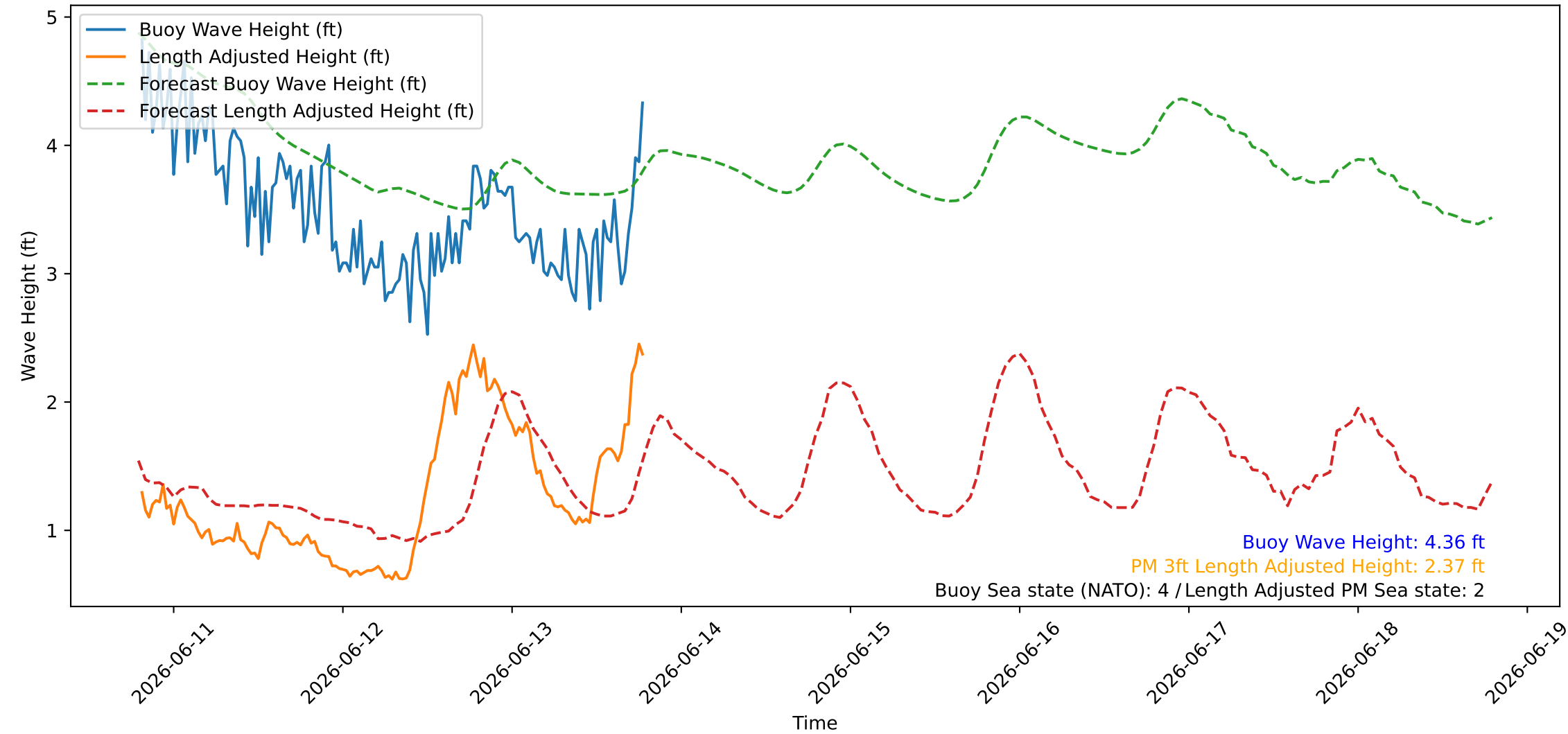
Wave Heights over Time for Red Beach at 2026-06-13 19:20:47
