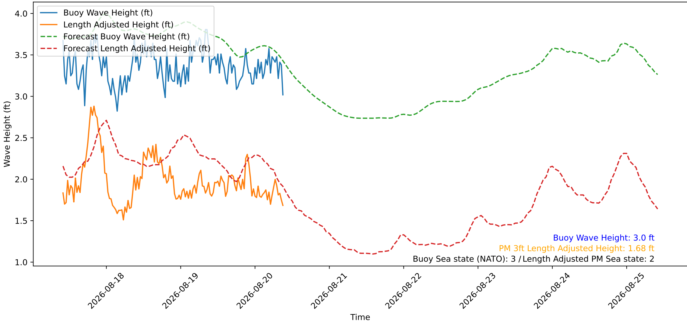
Wave Heights over Time for Oceanside Harbor at 2026-08-20 10:00:26
