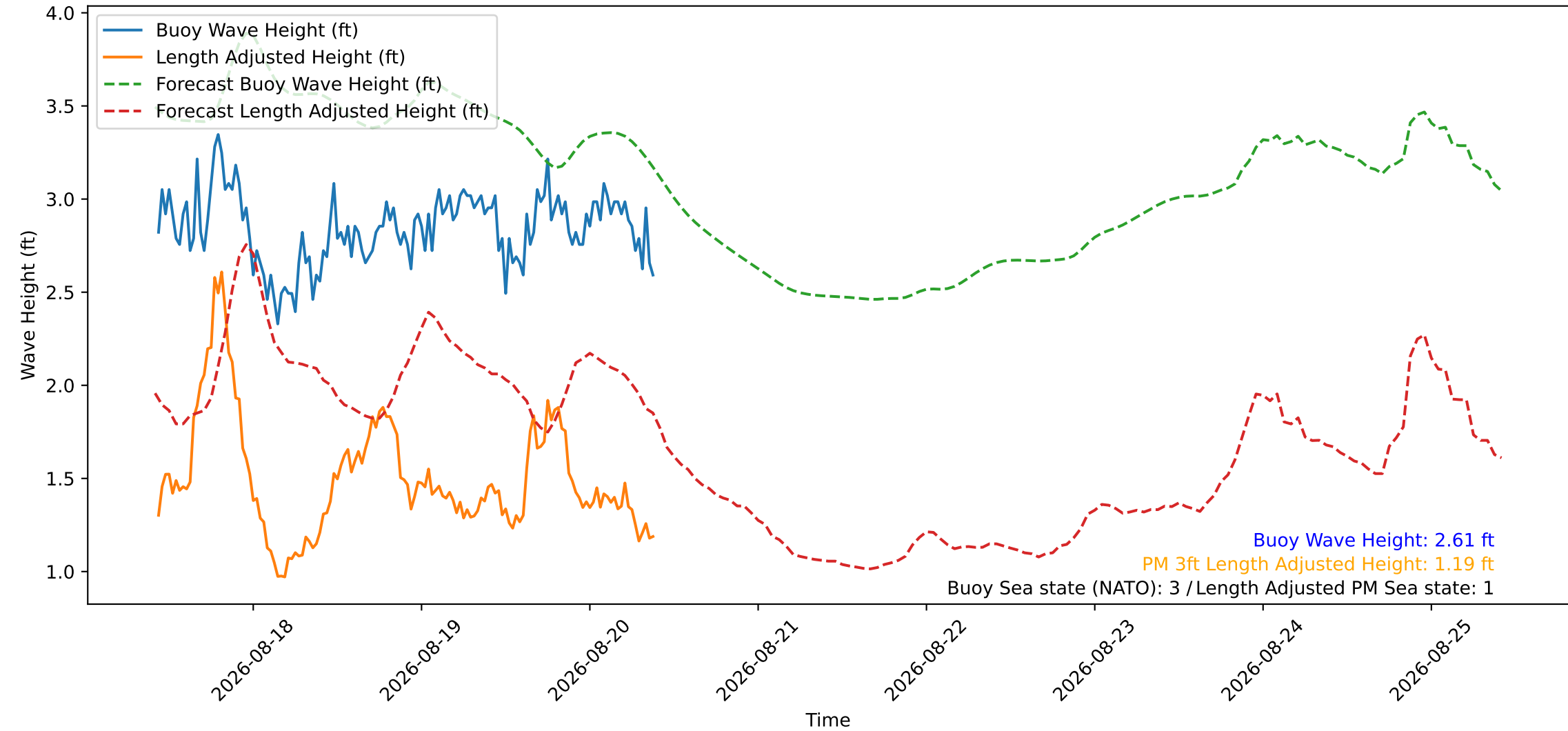
Wave Heights over Time for Red Beach at 2026-08-20 10:00:46
