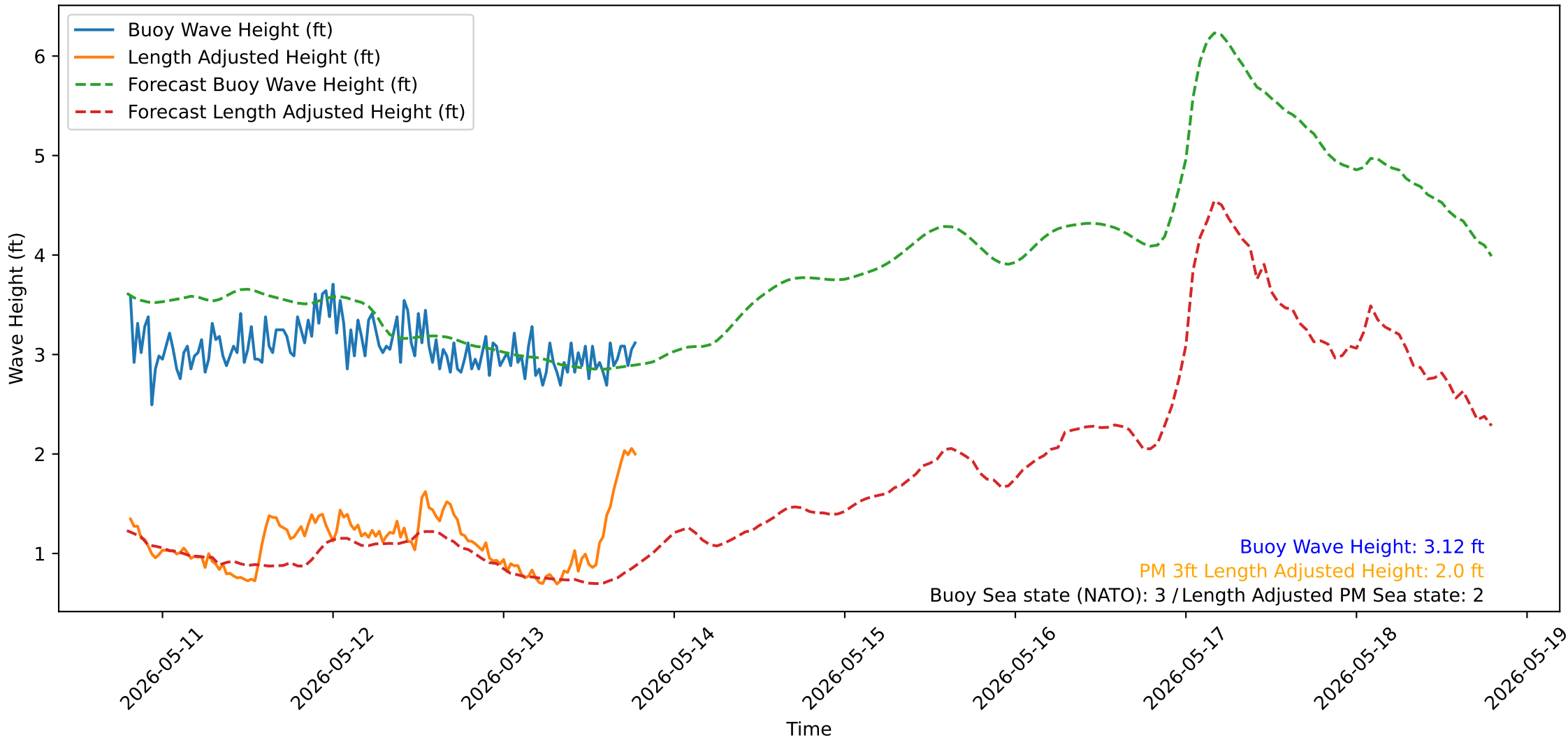
Wave Heights over Time for Oceanside Harbor at 2026-05-13 19:20:31
