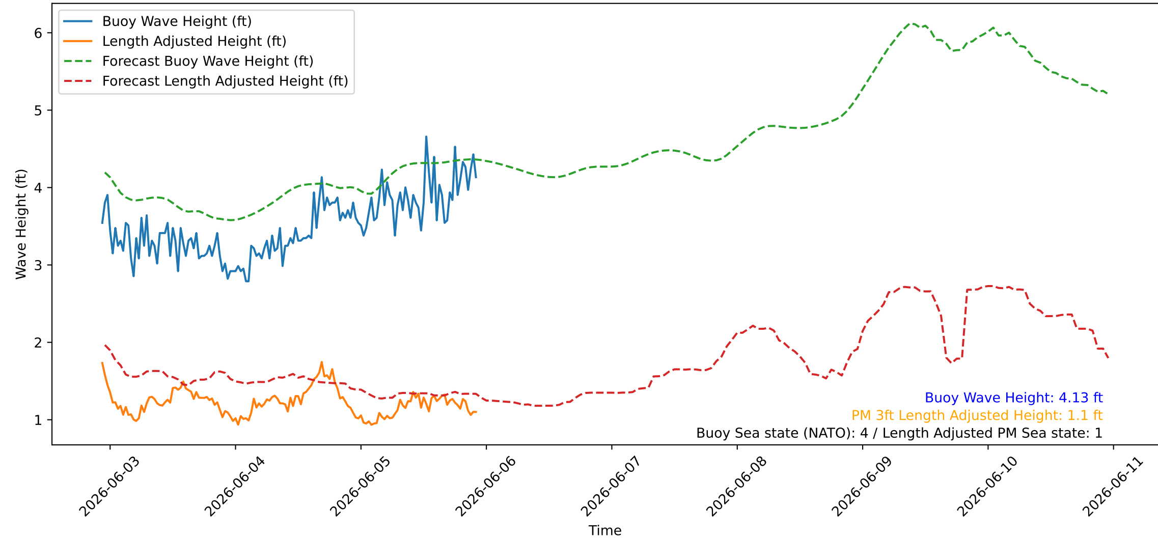
Wave Heights over Time for Green Beach at 2026-06-05 22:41:09
