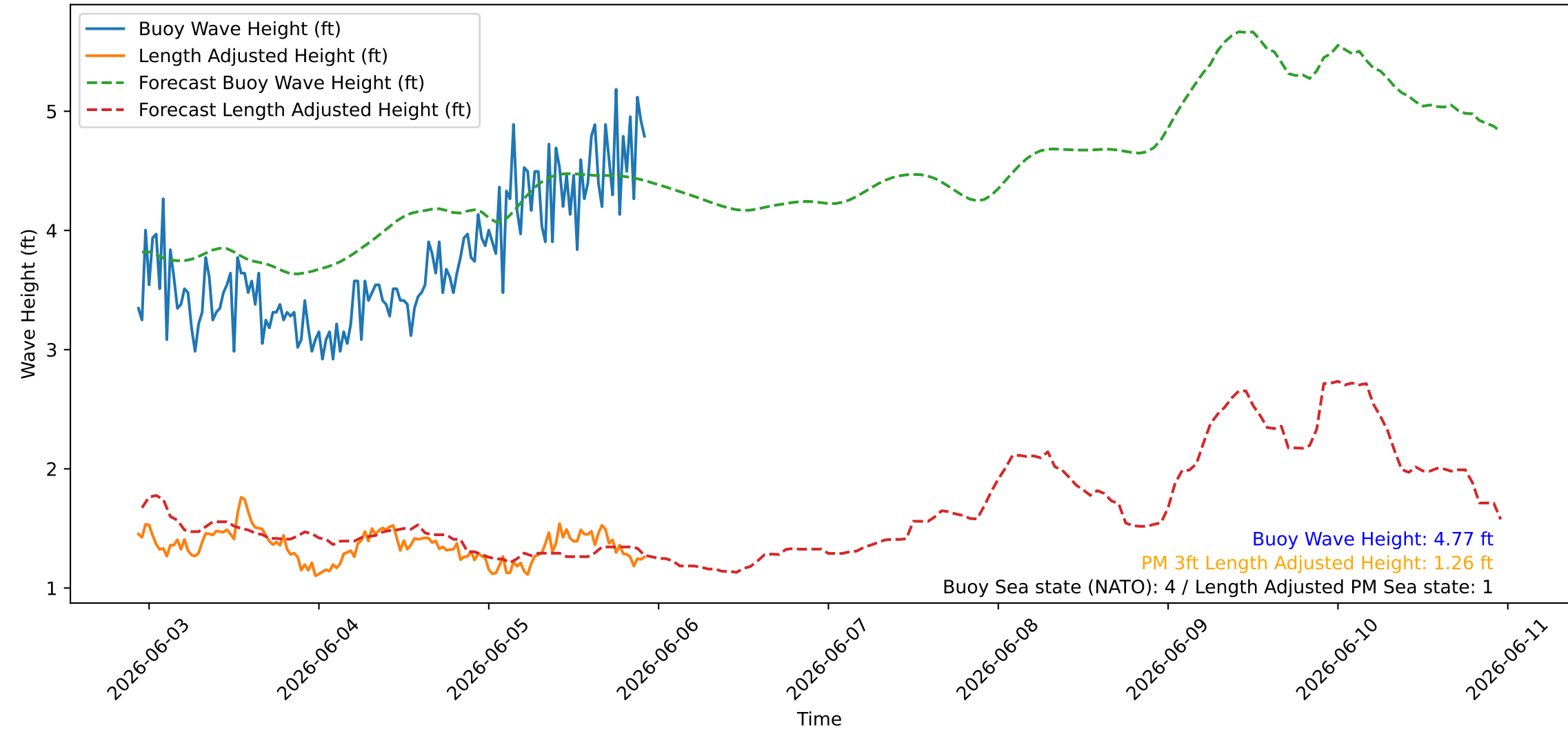
Wave Heights over Time for Oceanside Harbor at 2026-06-05 22:40:26
