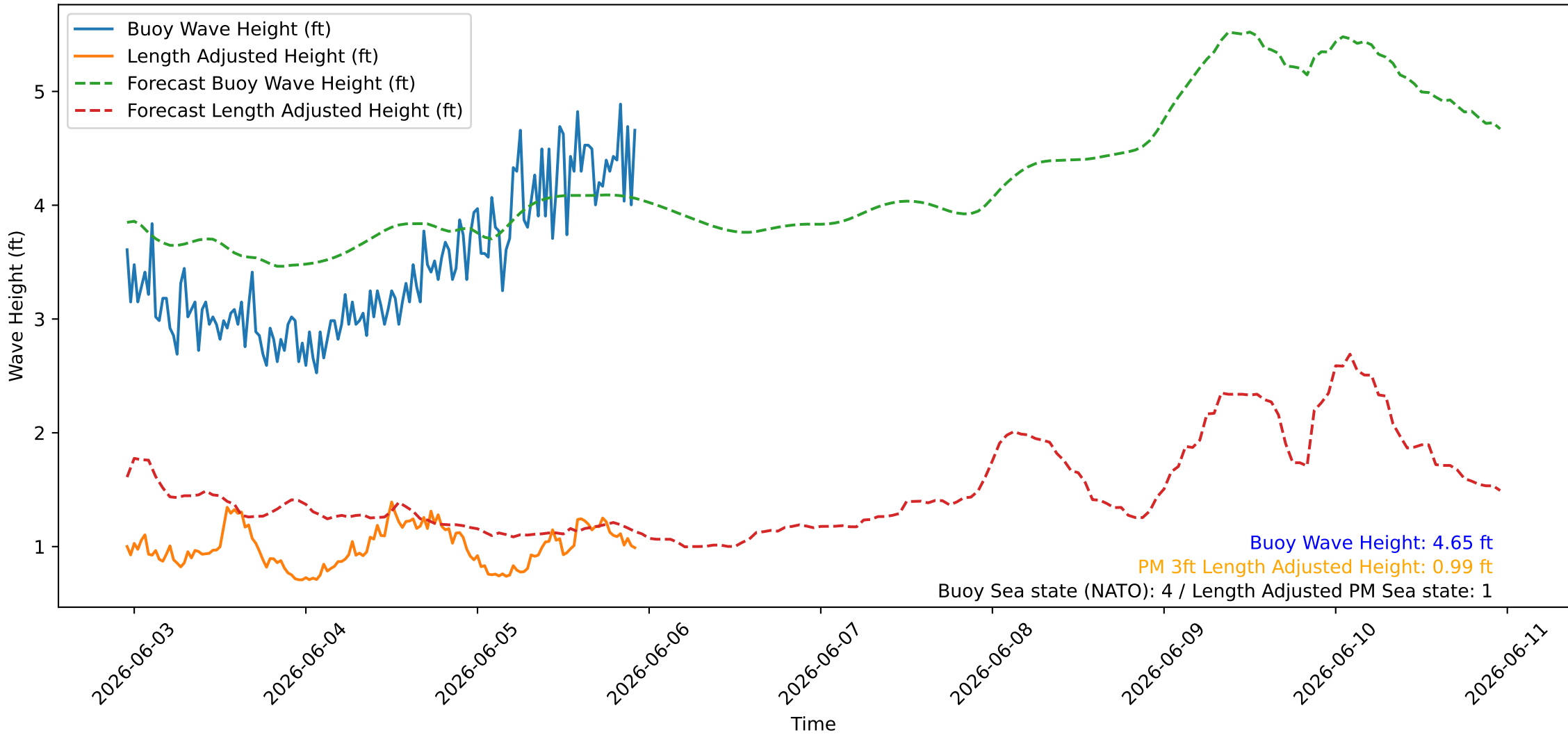
Wave Heights over Time for Red Beach at 2026-06-05 22:40:46
