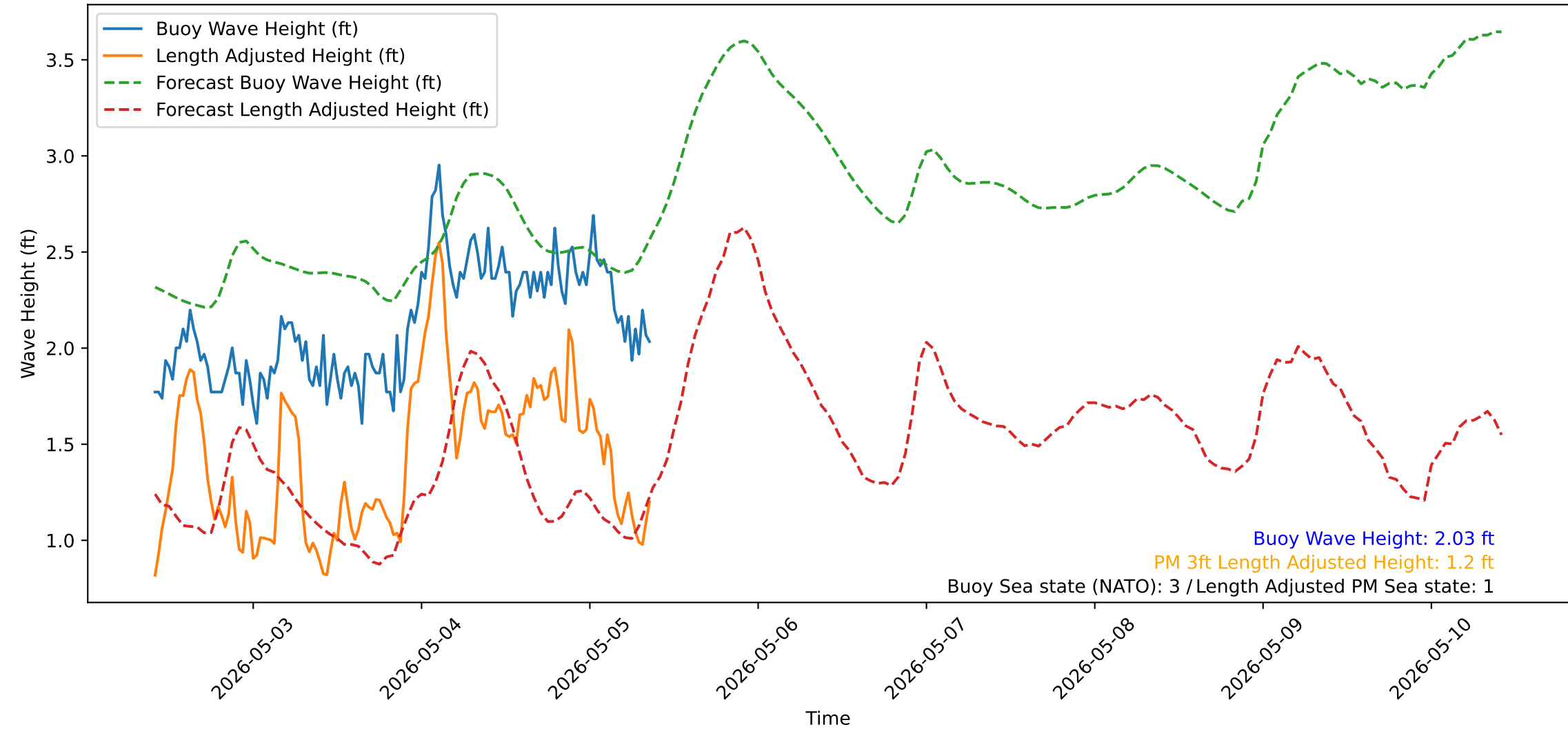
Wave Heights over Time for Red Beach at 2026-05-05 09:30:51
