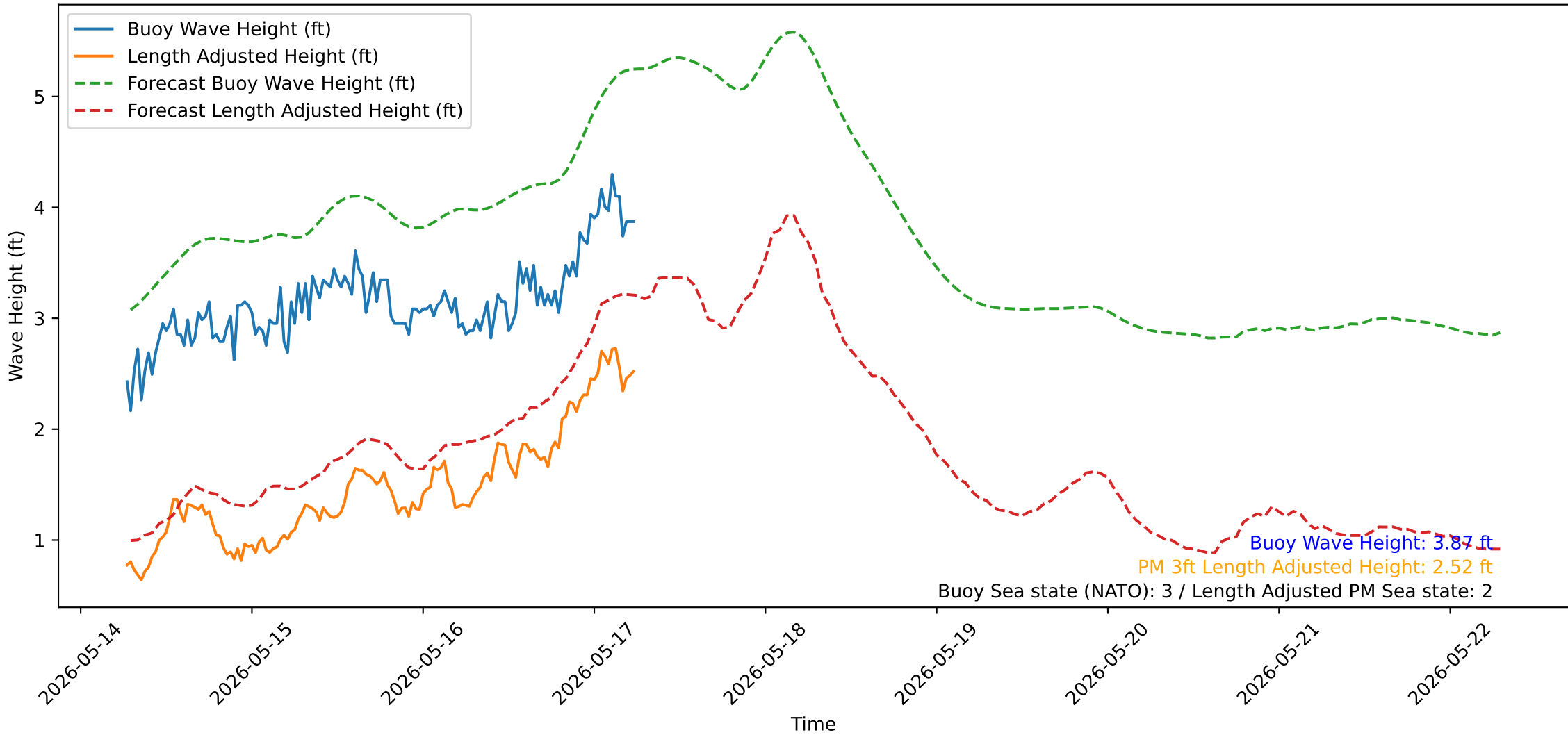
Wave Heights over Time for Oceanside Harbor at 2026-05-17 06:30:31
