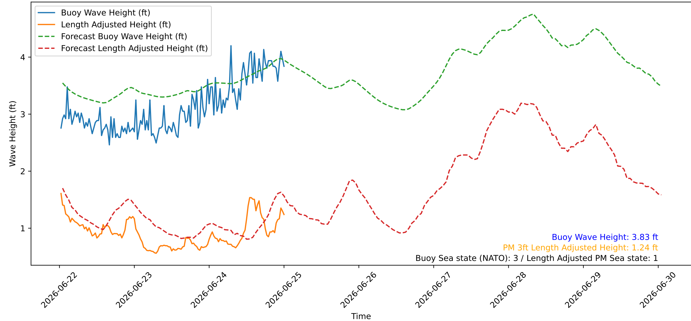
Wave Heights over Time for Green Beach at 2026-06-25 00:41:08
