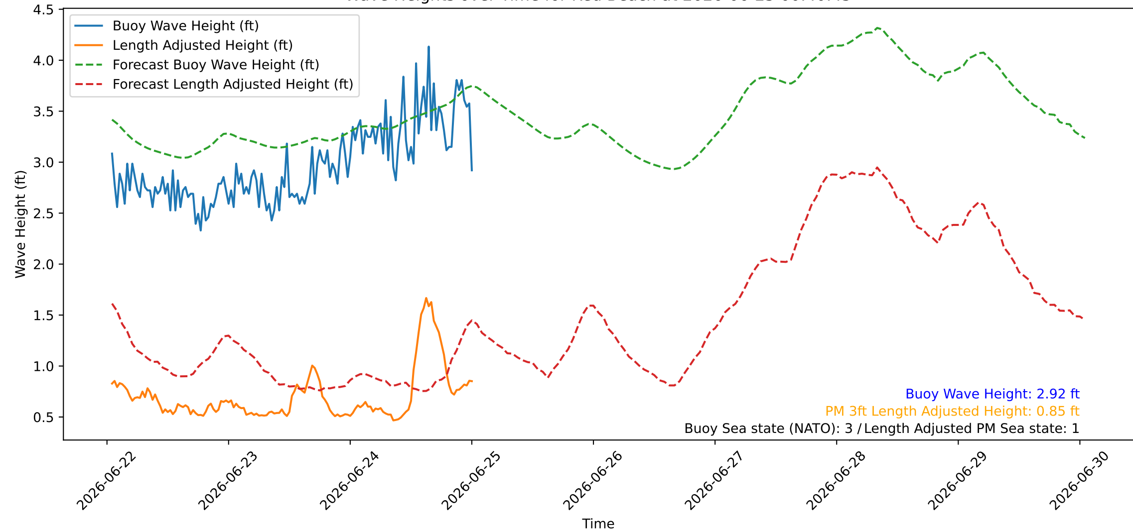
Wave Heights over Time for Red Beach at 2026-06-25 00:40:45
