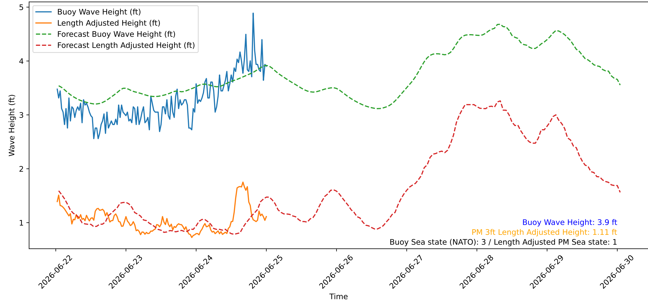
Wave Heights over Time for Oceanside Harbor at 2026-06-25 00:40:26
