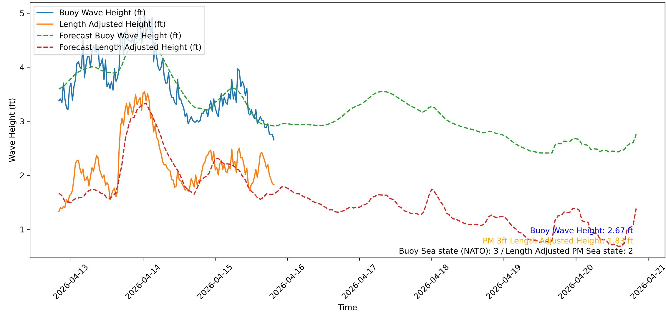
Wave Heights over Time for Green Beach at 2026-04-15 20:11:14
