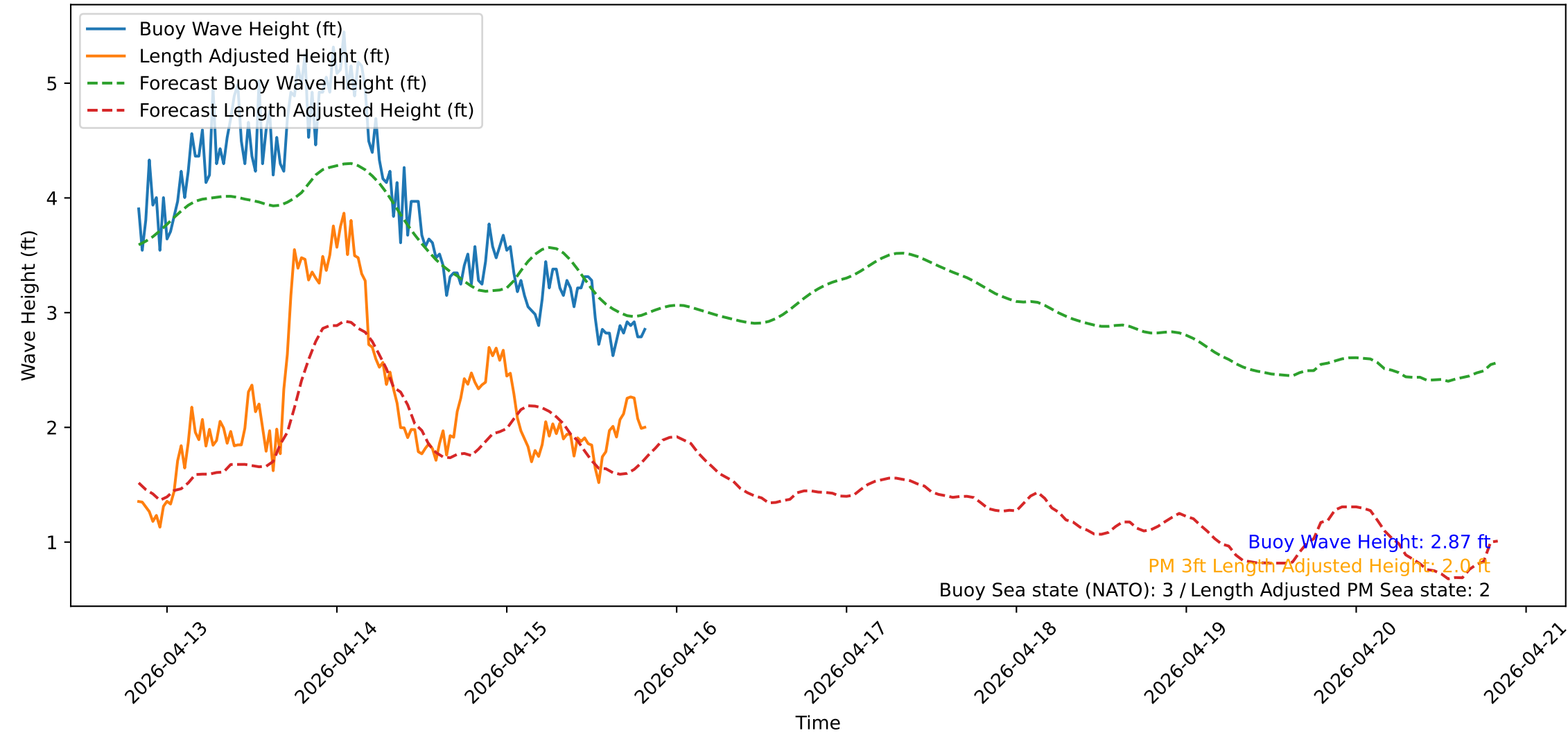
Wave Heights over Time for Oceanside Harbor at 2026-04-15 20:10:32
