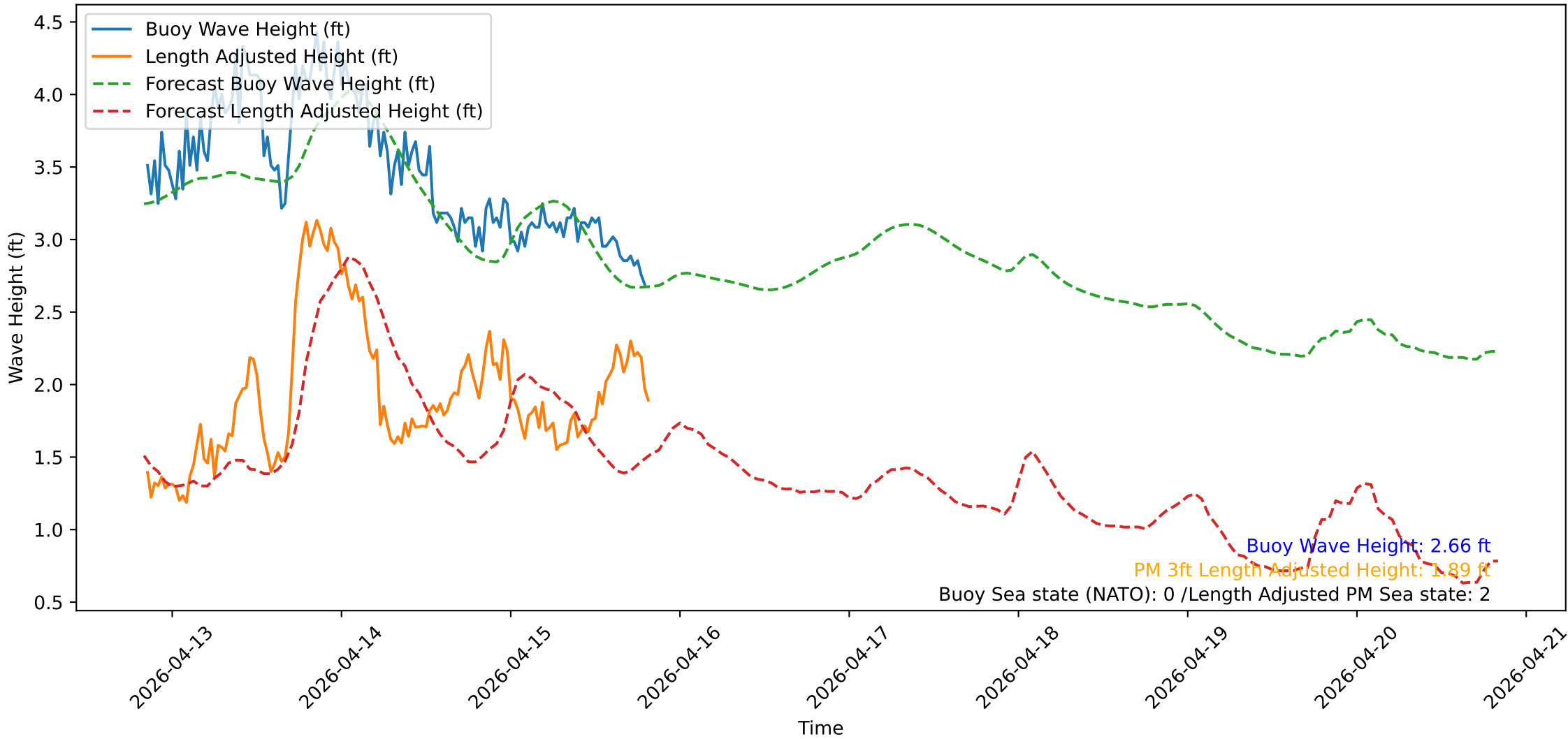
Wave Heights over Time for Red Beach at 2026-04-15 20:10:51
