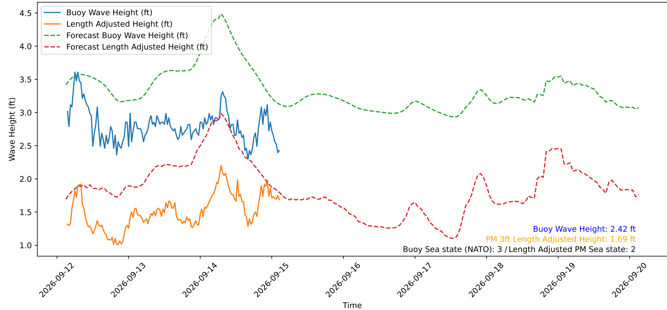
Wave Heights over Time for Green Beach at 2026-09-15 03:21:14
