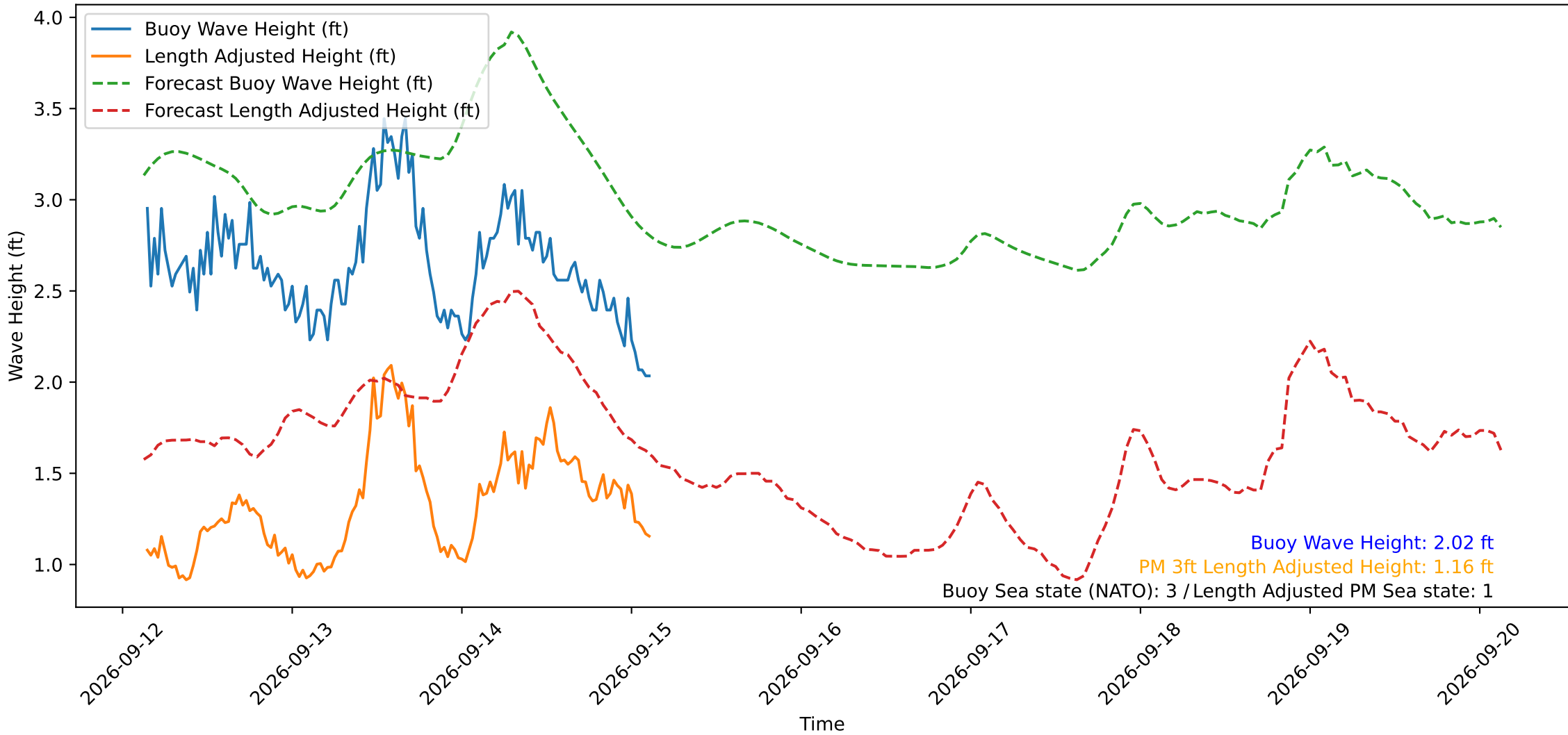
Wave Heights over Time for Red Beach at 2026-09-15 03:20:50
