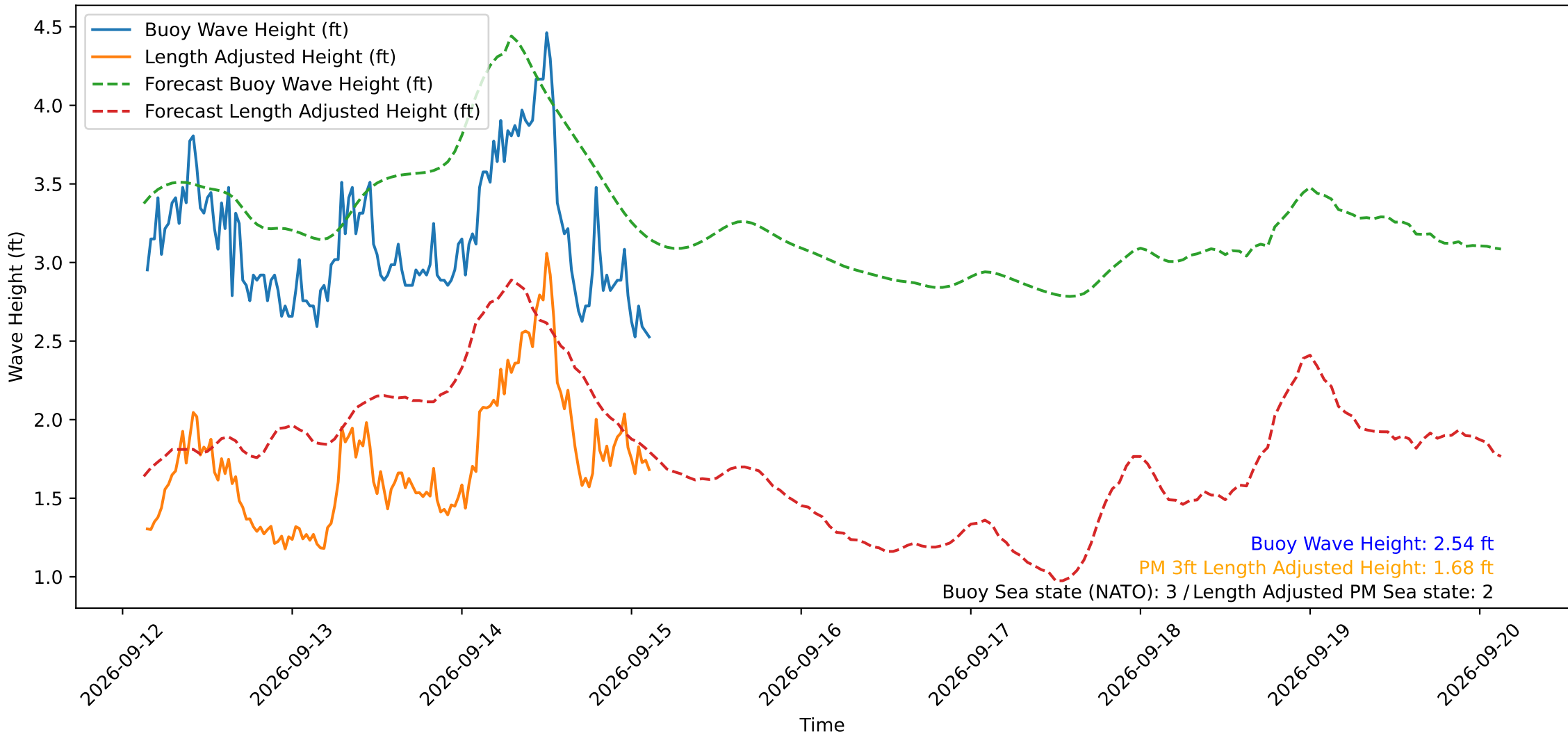
Wave Heights over Time for Oceanside Harbor at 2026-09-15 03:20:29
