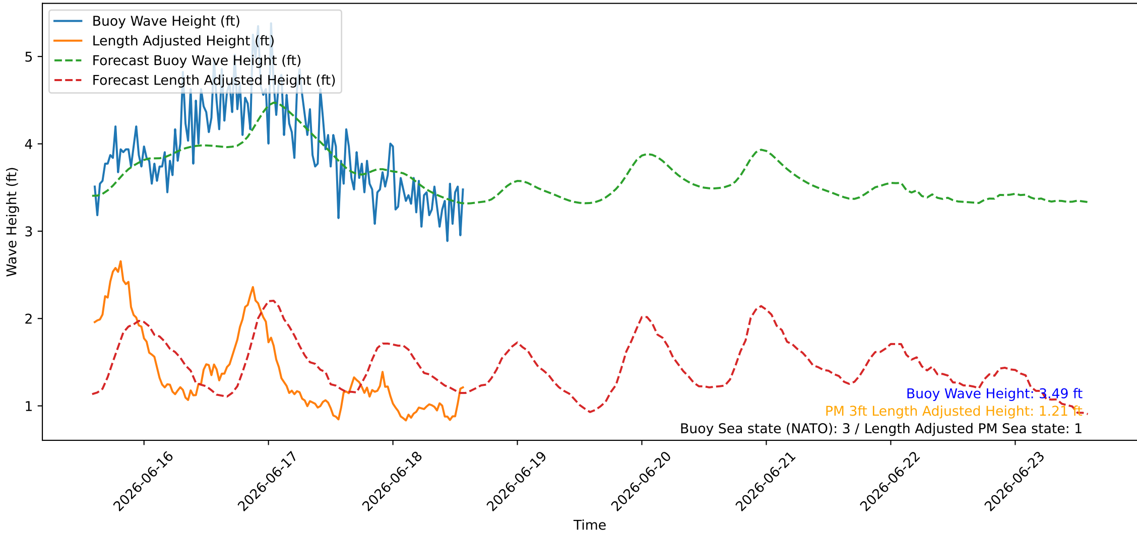
Wave Heights over Time for Red Beach at 2026-06-18 14:10:47
