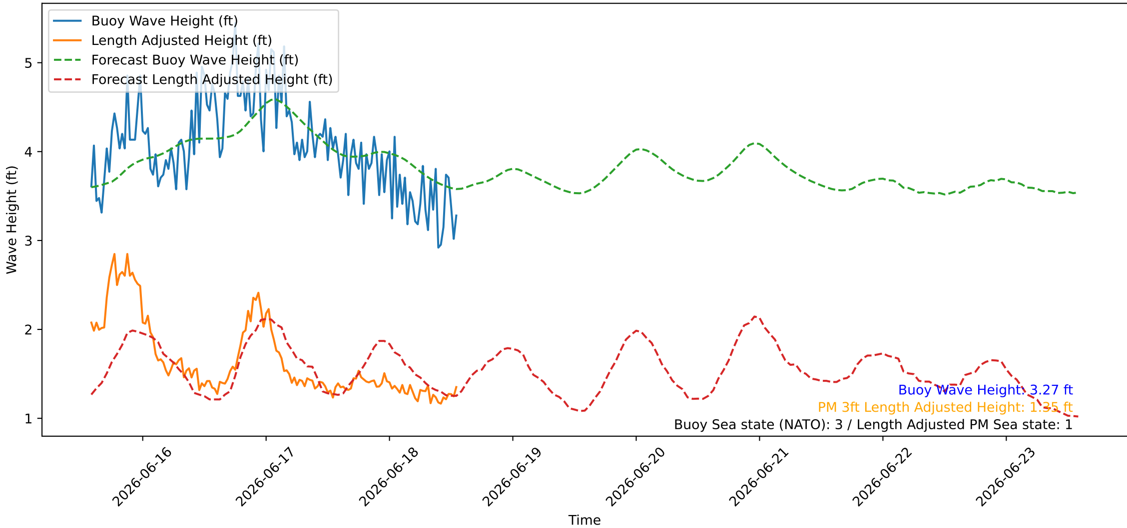
Wave Heights over Time for Oceanside Harbor at 2026-06-18 14:10:27
