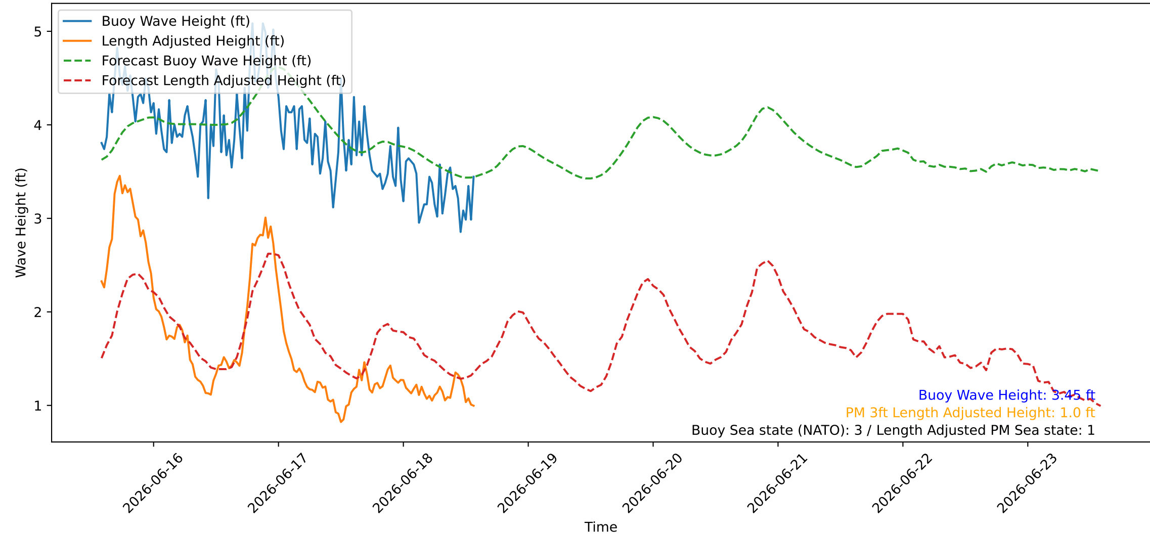
Wave Heights over Time for Green Beach at 2026-06-18 14:11:09
