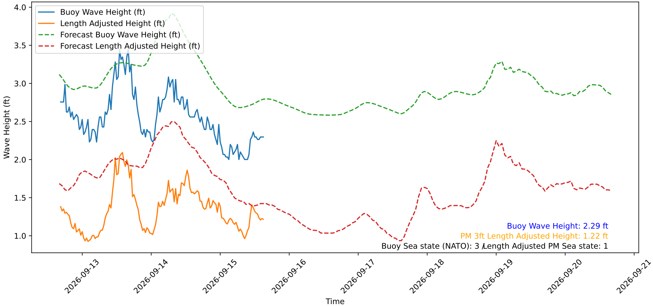
Wave Heights over Time for Red Beach at 2026-09-15 16:00:49
