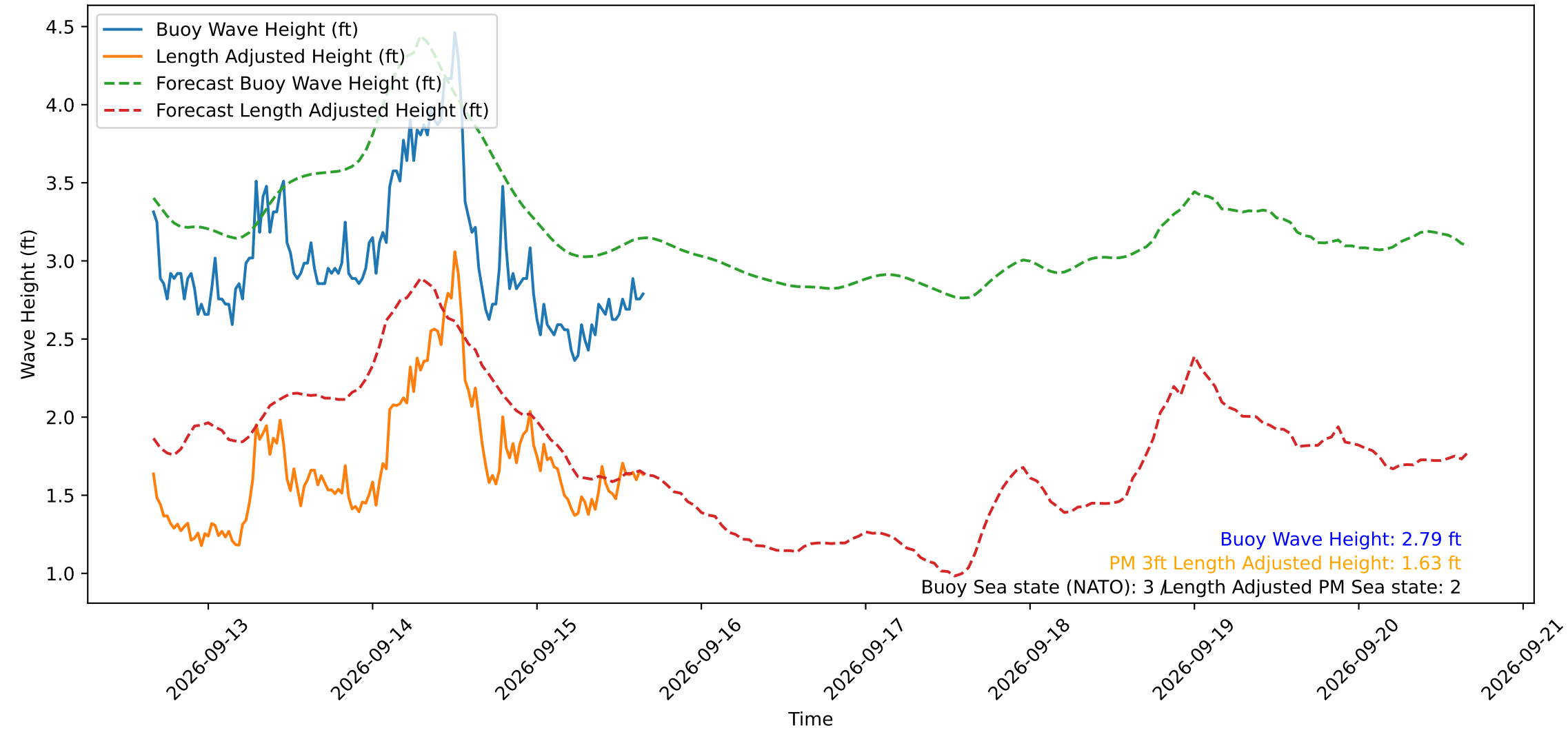
Wave Heights over Time for Oceanside Harbor at 2026-09-15 16:00:30
