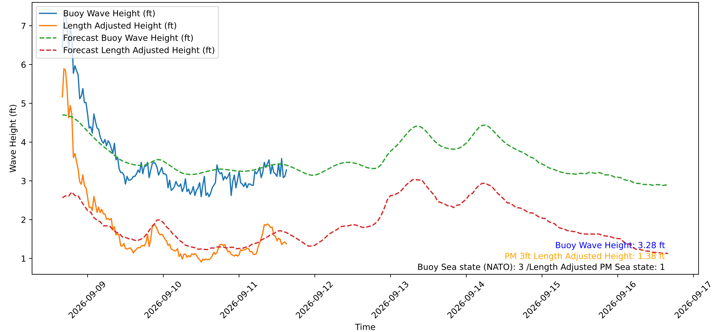
Wave Heights over Time for Green Beach at 2026-09-11 15:51:14
