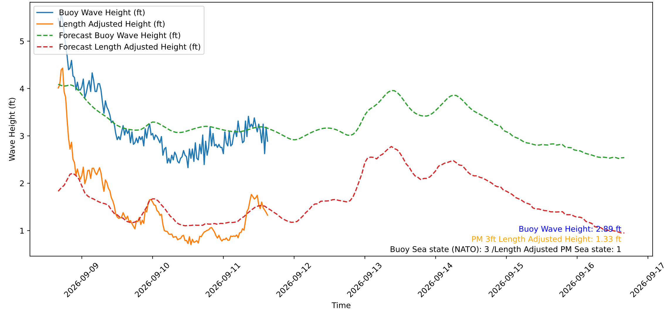
Wave Heights over Time for Red Beach at 2026-09-11 15:50:50
