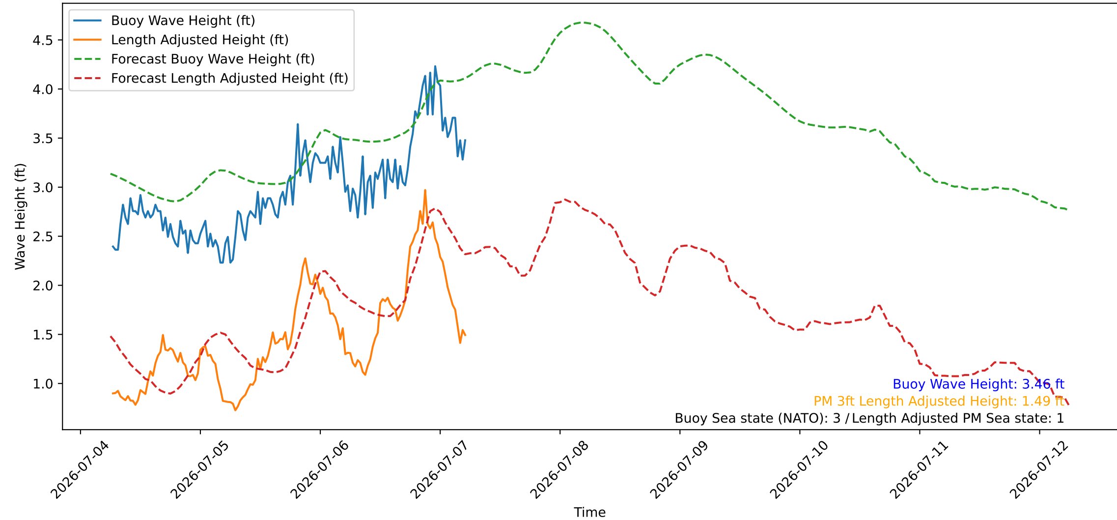
Wave Heights over Time for Red Beach at 2026-07-07 06:10:45
