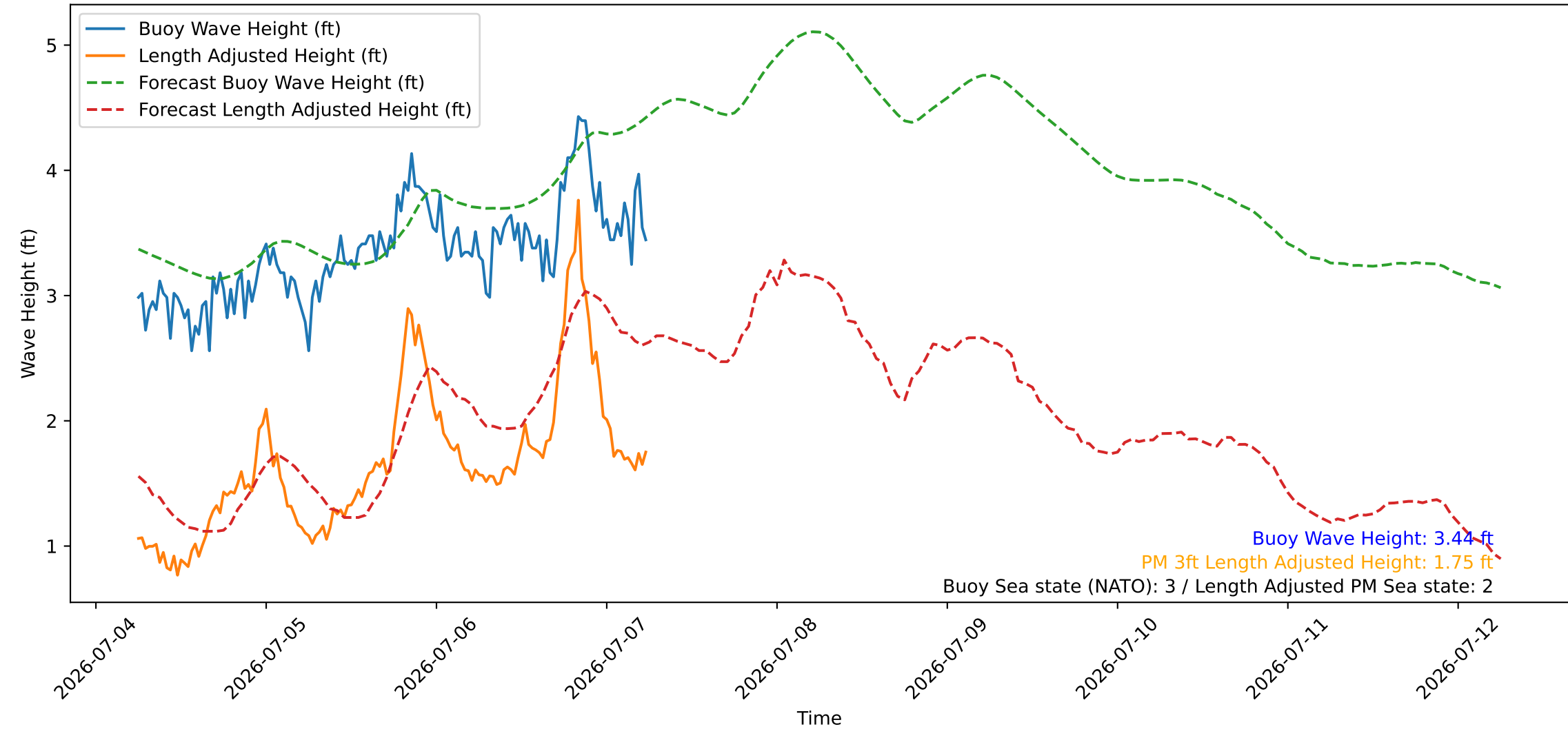
Wave Heights over Time for Green Beach at 2026-07-07 06:11:08
