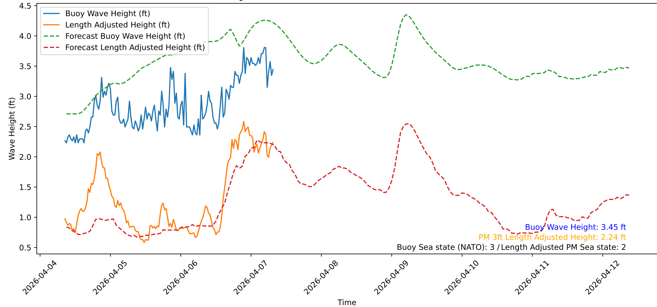
Wave Heights over Time for Green Beach at 2026-04-07 08:31:10
