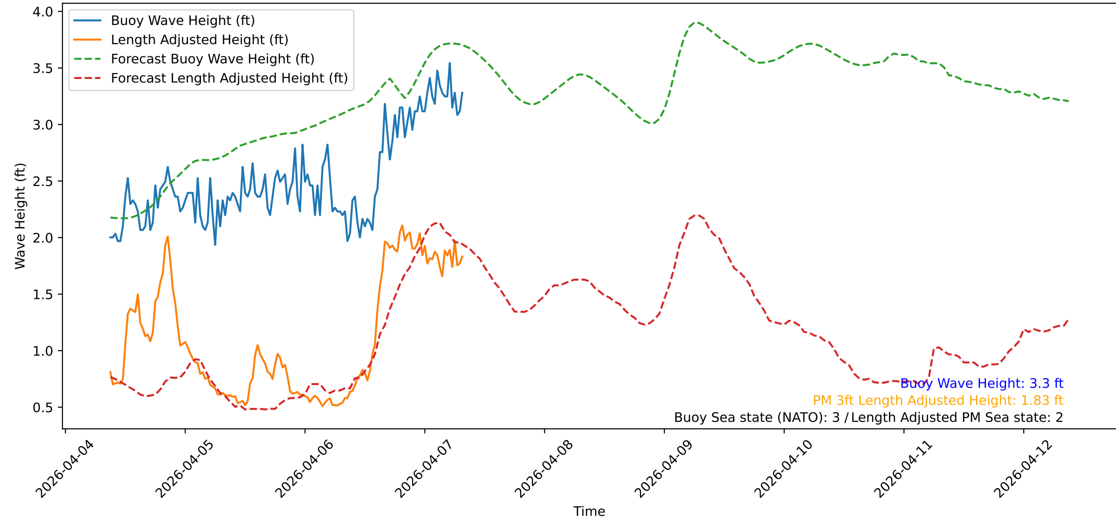
Wave Heights over Time for Red Beach at 2026-04-07 08:30:48
