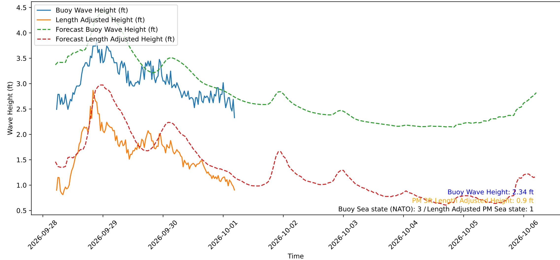
Wave Heights over Time for Red Beach at 2026-10-01 05:20:51
