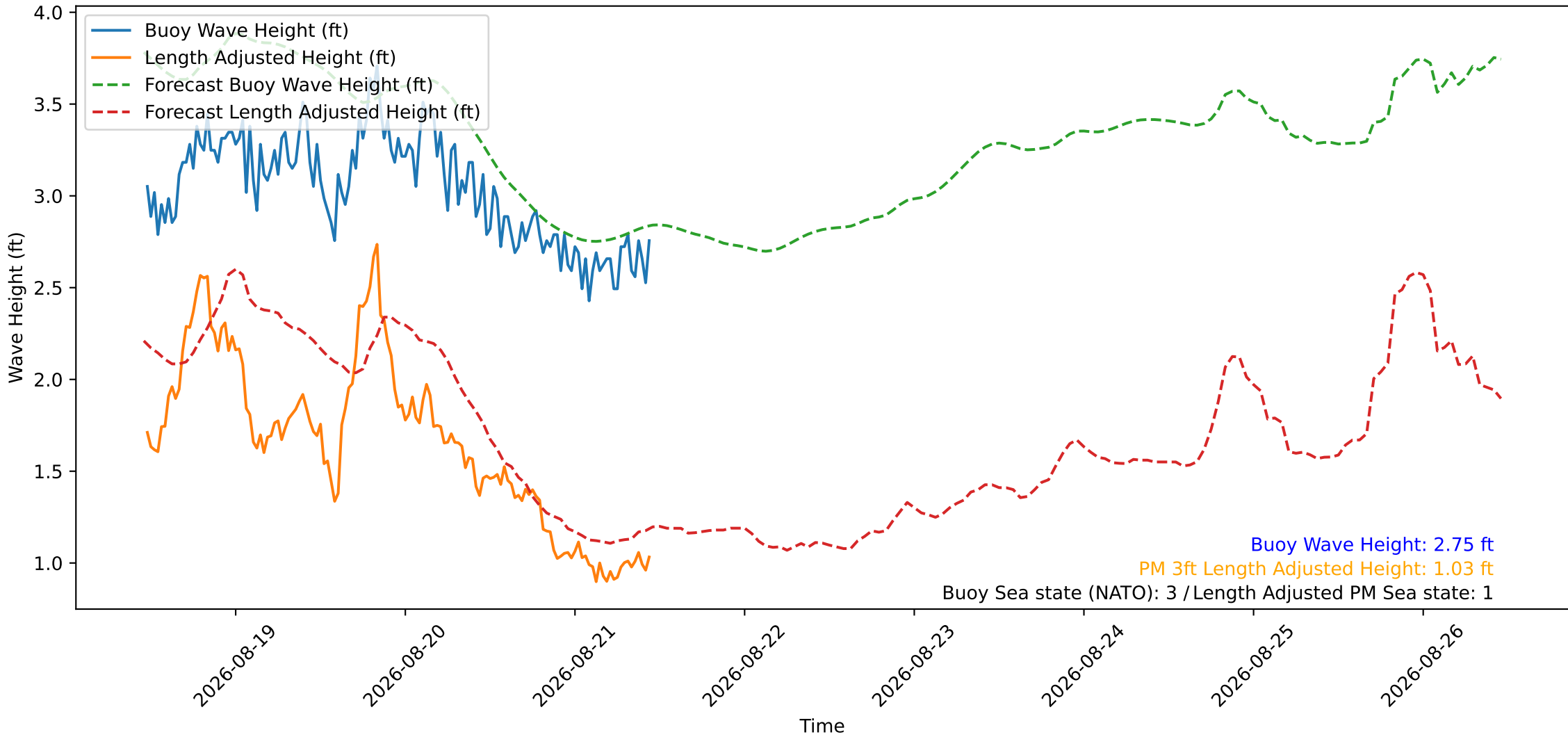
Wave Heights over Time for Green Beach at 2026-08-21 11:11:08
