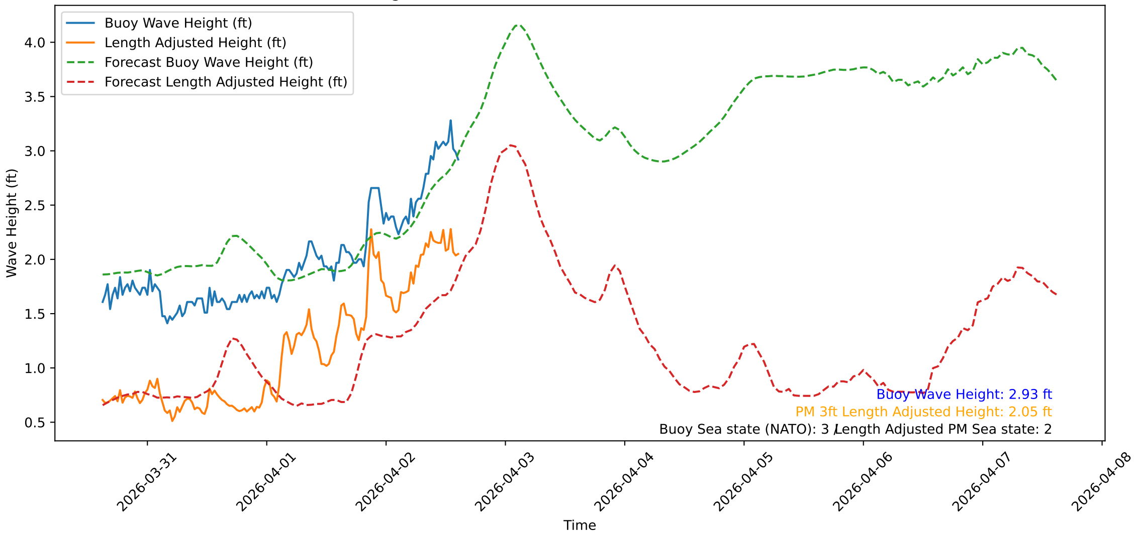
Wave Heights over Time for Green Beach at 2026-04-02 15:11:10
