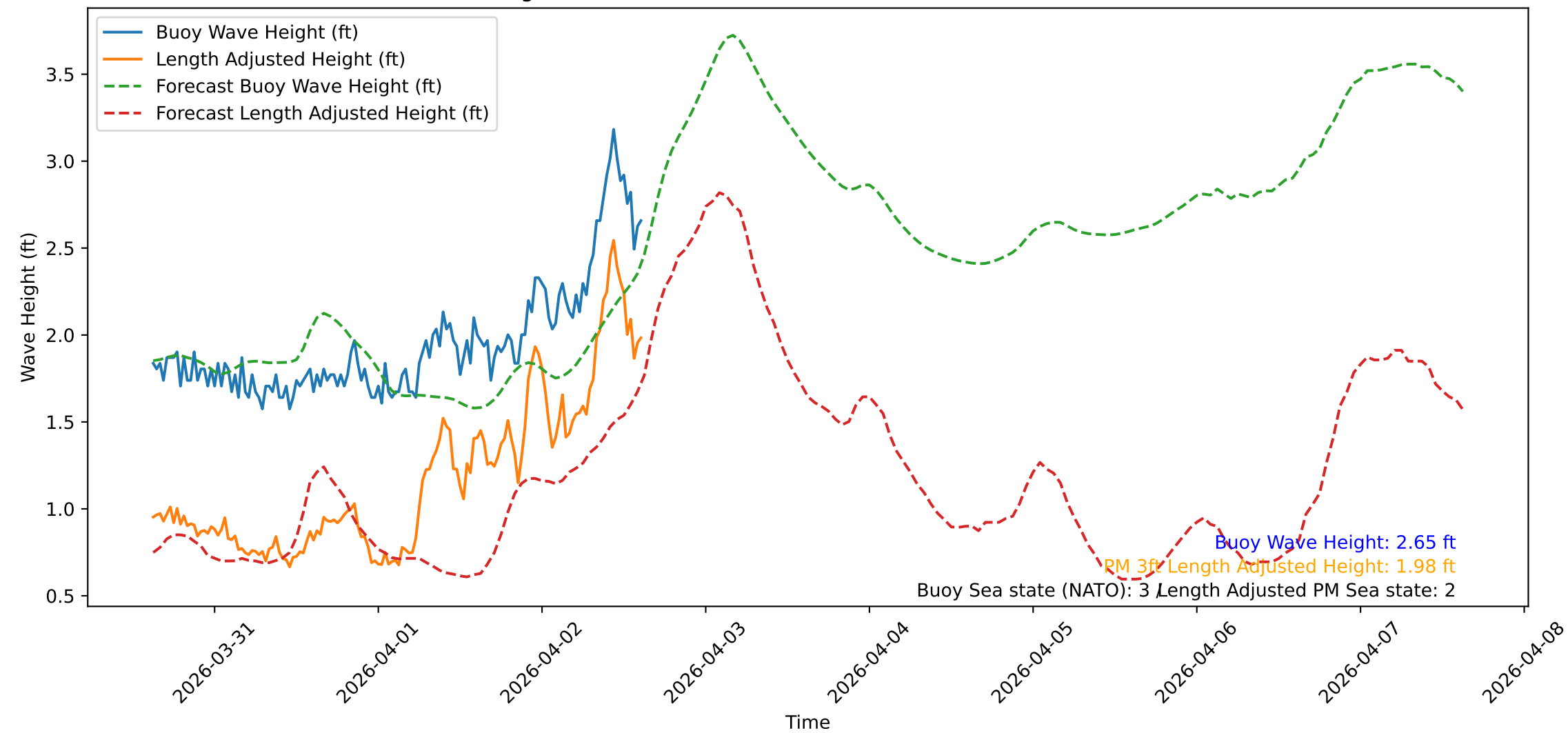
Wave Heights over Time for Oceanside Harbor at 2026-04-02 15:10:31
