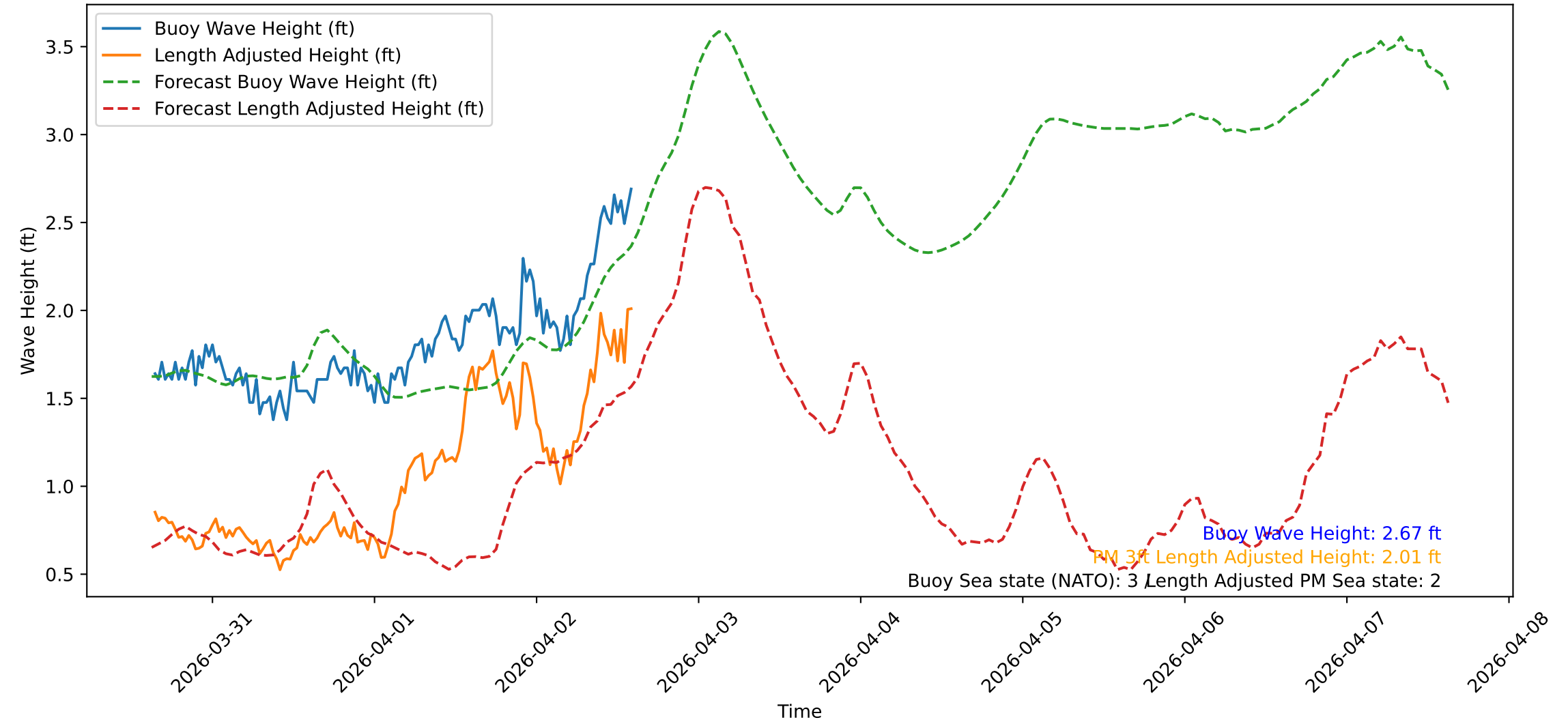
Wave Heights over Time for Red Beach at 2026-04-02 15:10:48
