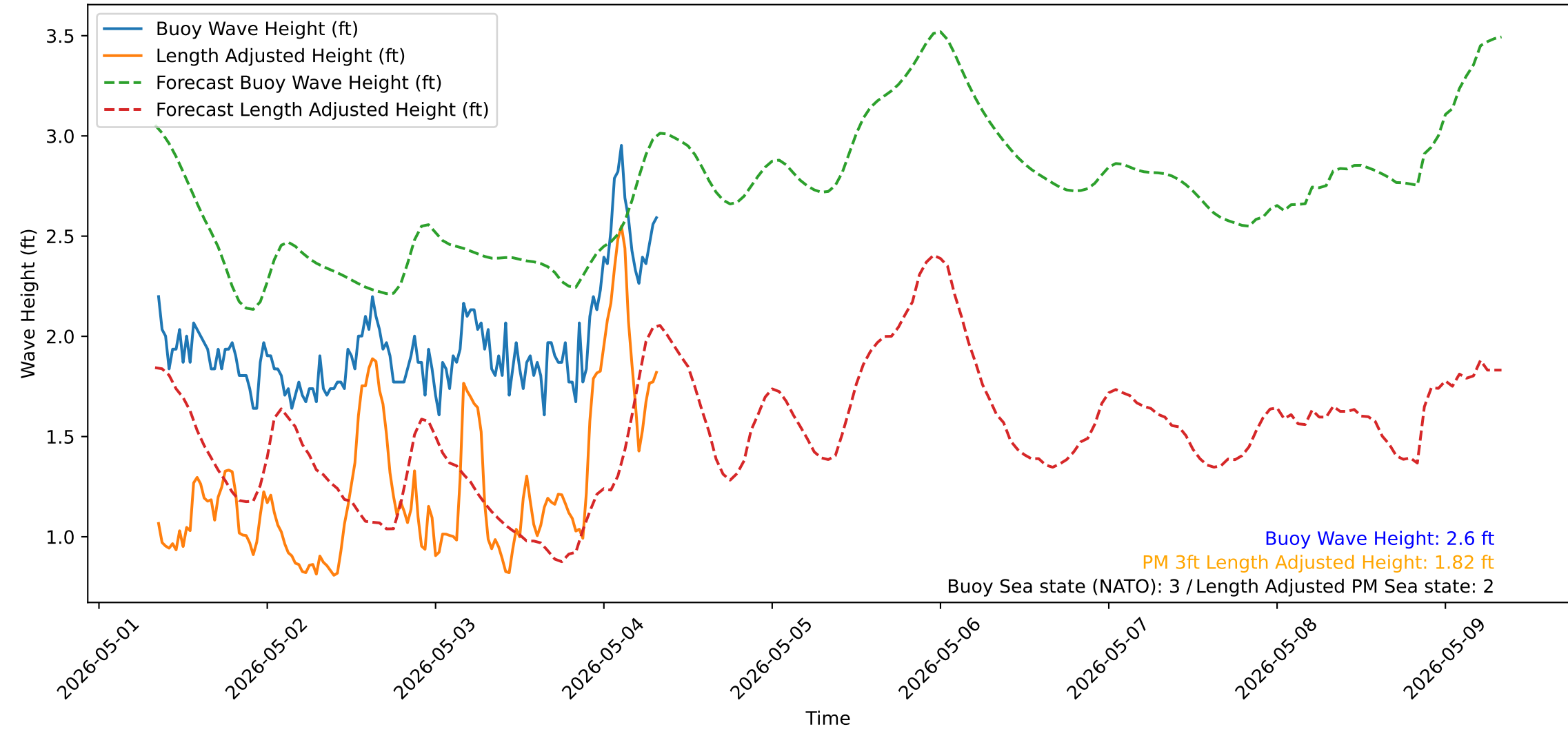
Wave Heights over Time for Red Beach at 2026-05-04 08:20:56
