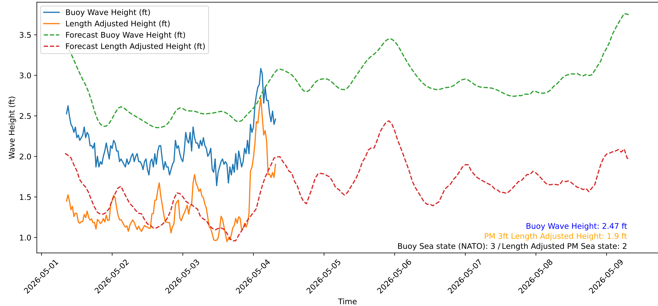
Wave Heights over Time for Oceanside Harbor at 2026-05-04 08:20:36
