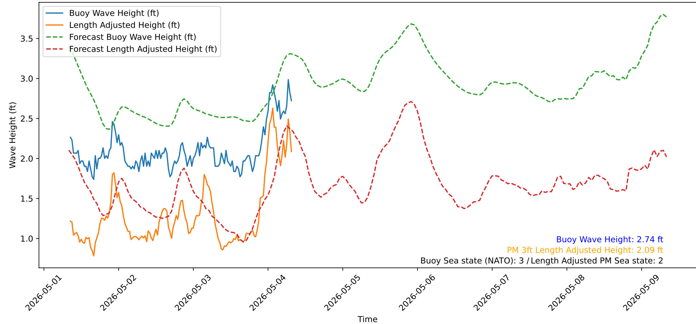
Wave Heights over Time for Green Beach at 2026-05-04 08:21:18
