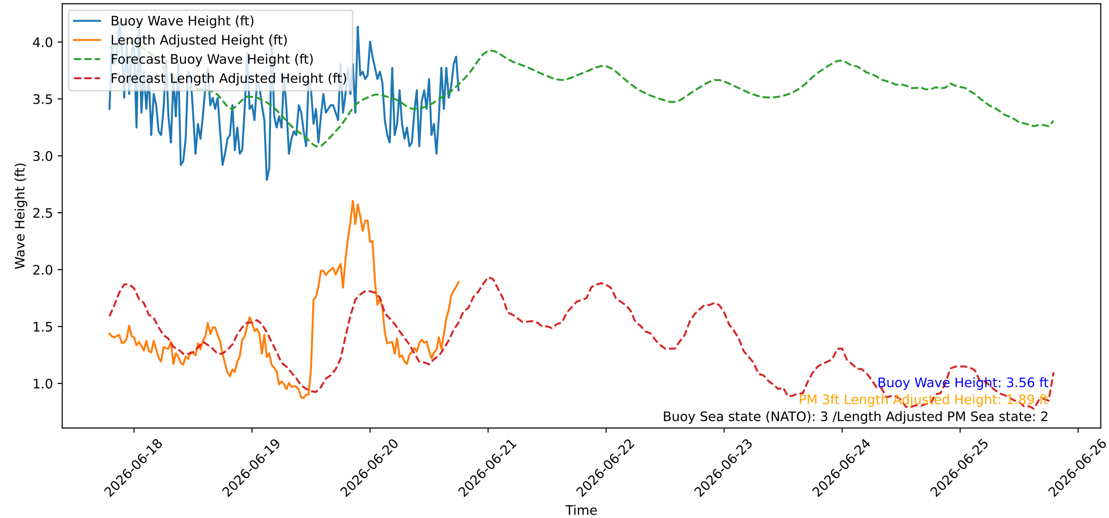
Wave Heights over Time for Oceanside Harbor at 2026-06-20 18:50:26
