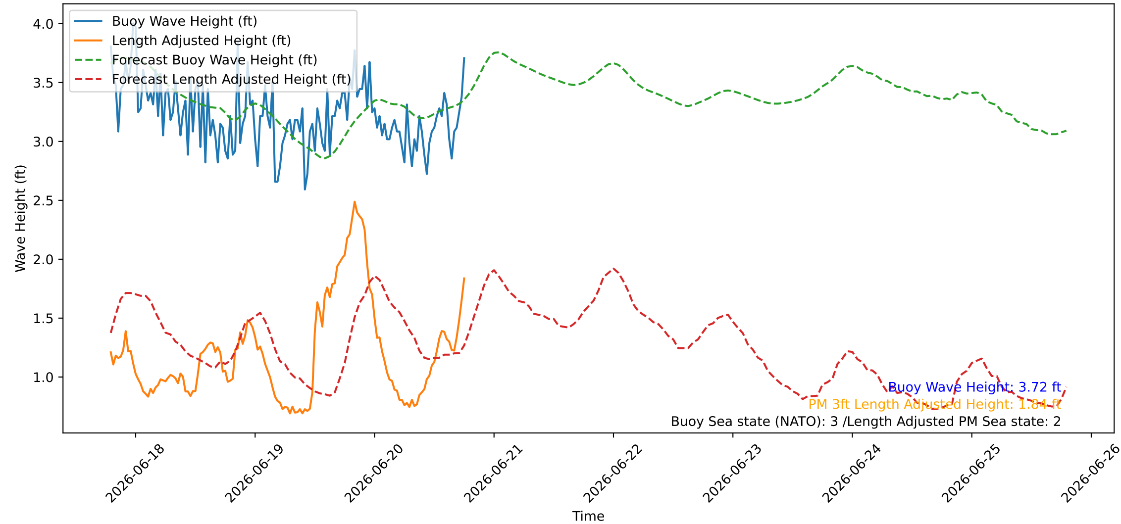
Wave Heights over Time for Red Beach at 2026-06-20 18:50:46
