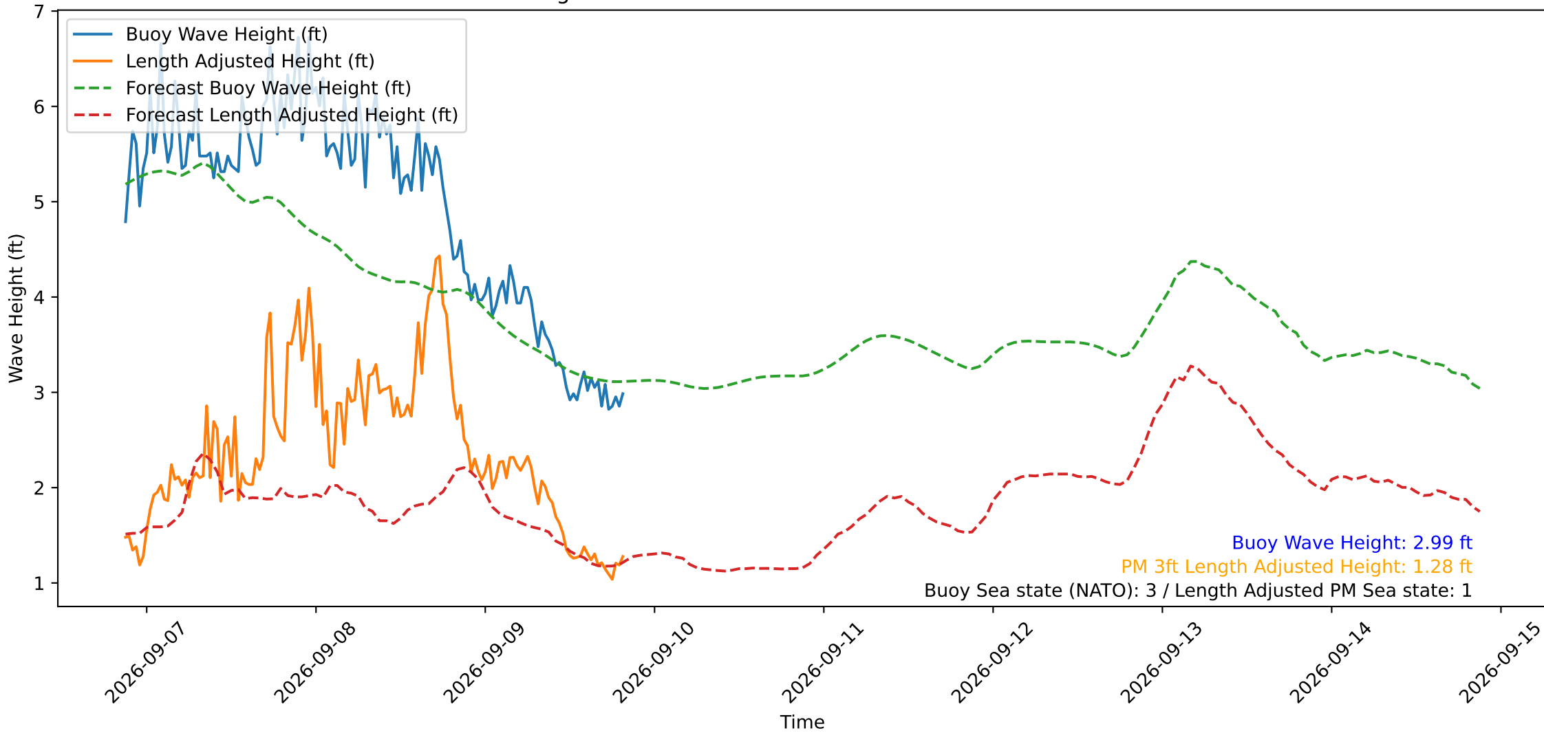
Wave Heights over Time for Red Beach at 2026-09-09 20:30:49
