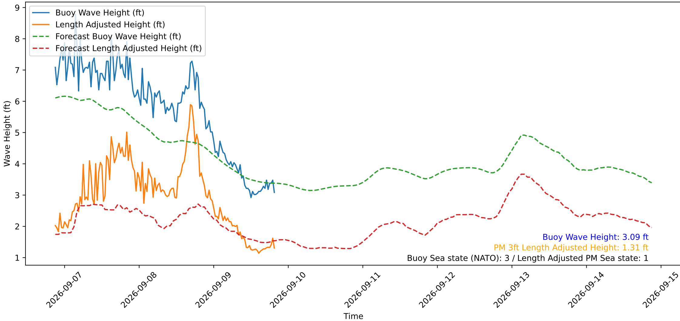
Wave Heights over Time for Green Beach at 2026-09-09 20:31:11
