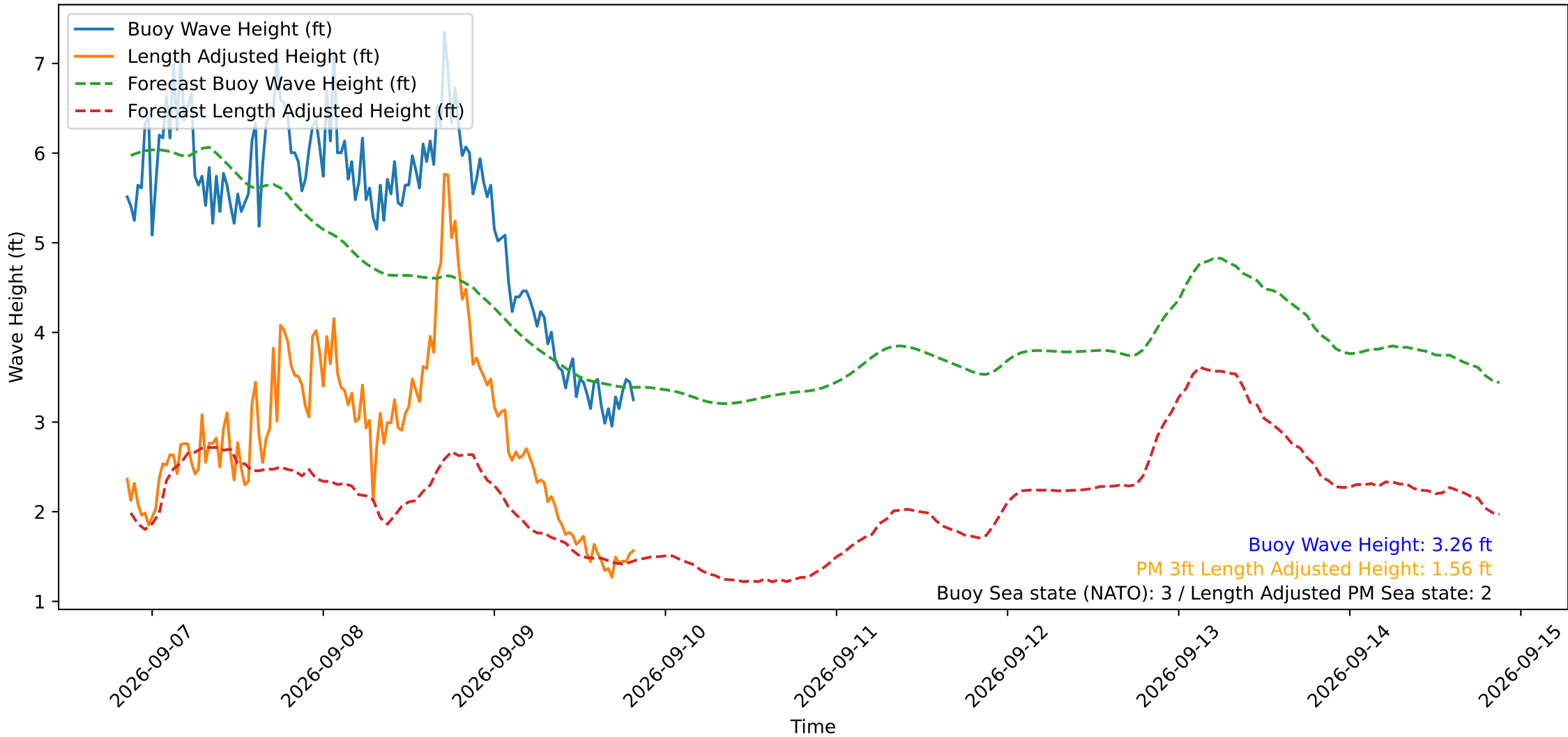
Wave Heights over Time for Oceanside Harbor at 2026-09-09 20:30:29
