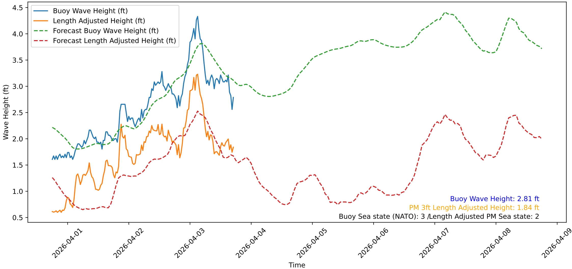
Wave Heights over Time for Green Beach at 2026-04-03 18:01:11
