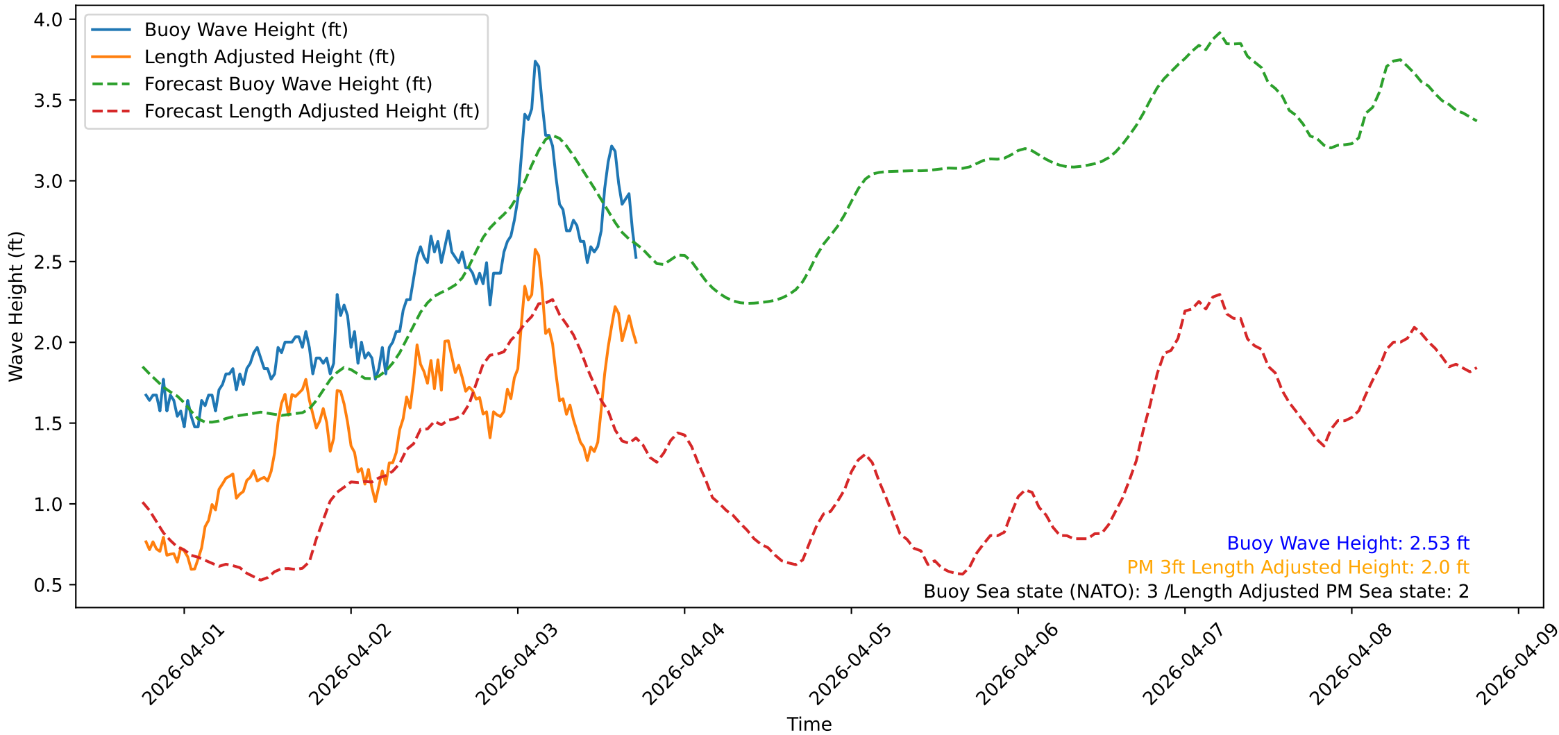
Wave Heights over Time for Red Beach at 2026-04-03 18:00:48
