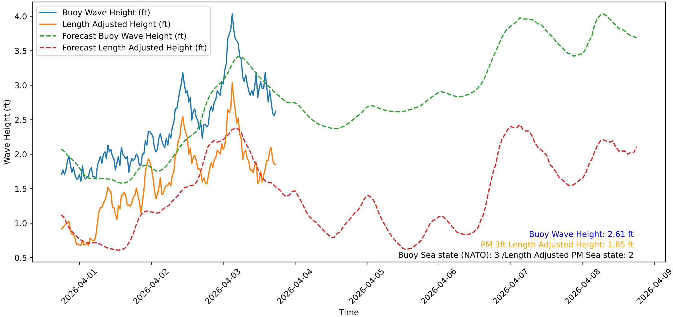
Wave Heights over Time for Oceanside Harbor at 2026-04-03 18:00:32
