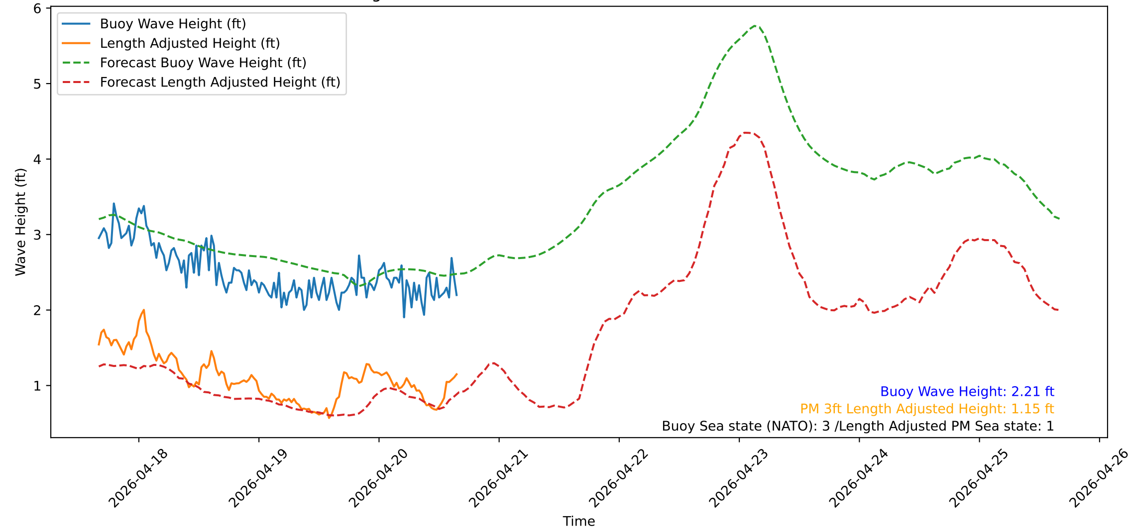
Wave Heights over Time for Oceanside Harbor at 2026-04-20 16:10:31
