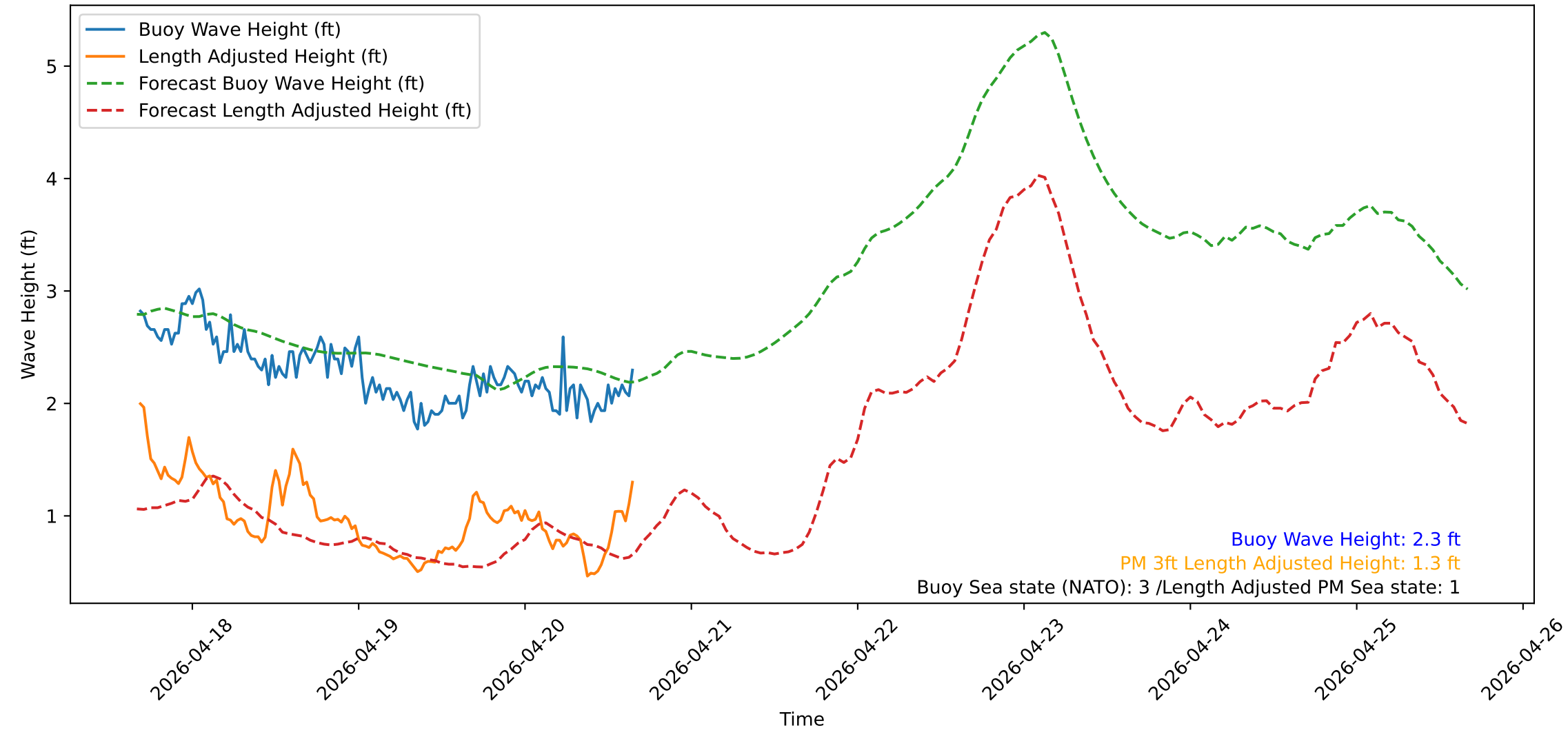
Wave Heights over Time for Red Beach at 2026-04-20 16:10:50
