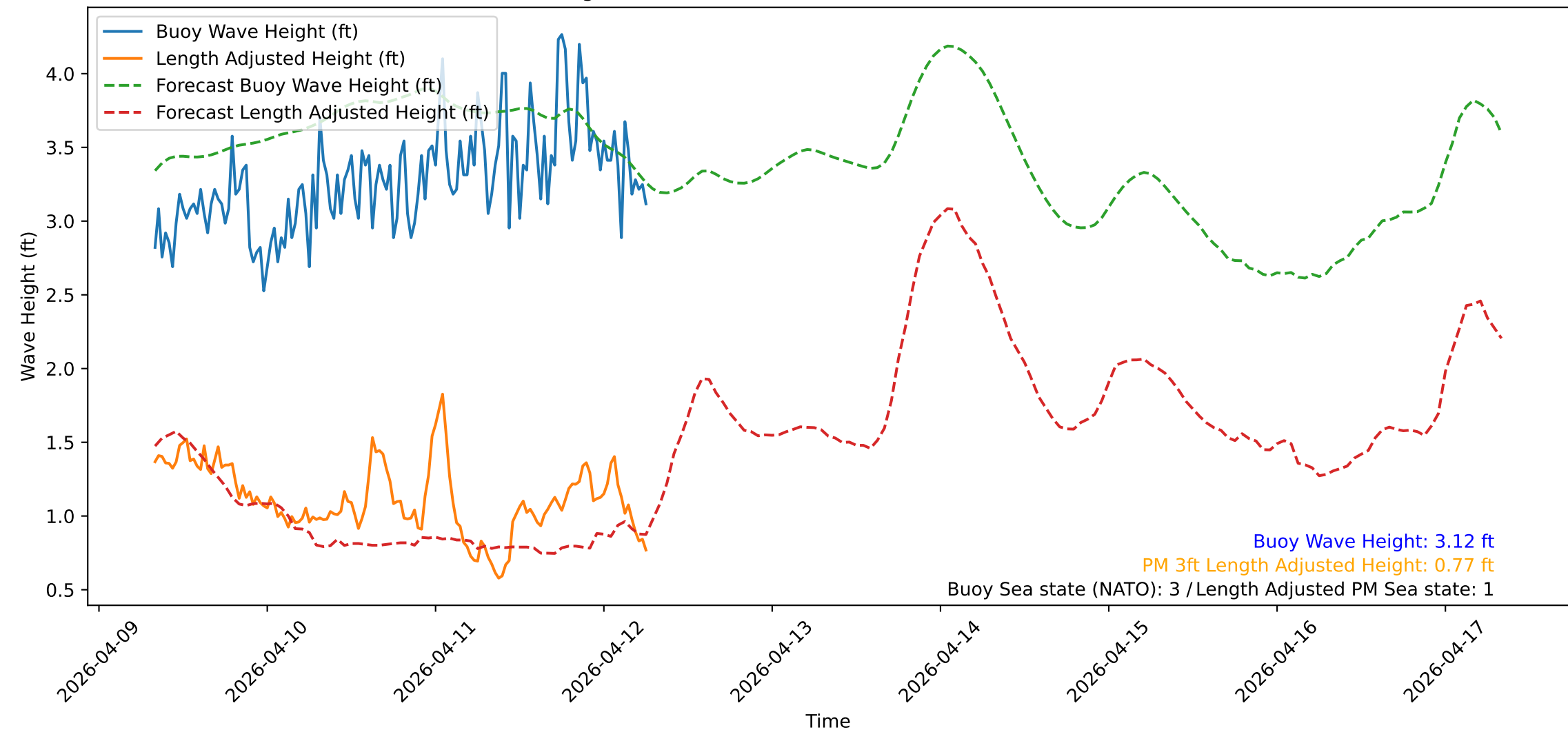
Wave Heights over Time for Red Beach at 2026-04-12 07:30:50
