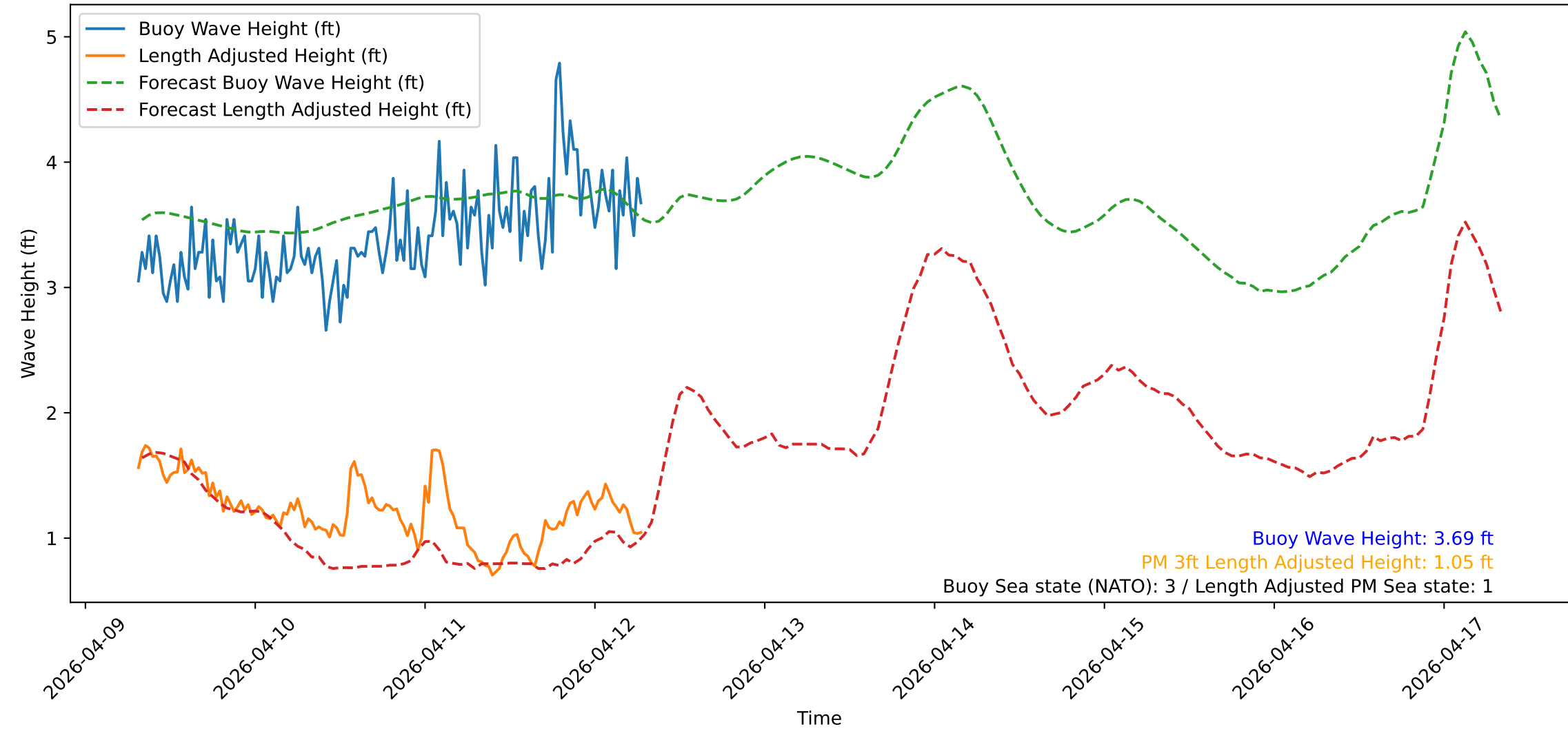
Wave Heights over Time for Oceanside Harbor at 2026-04-12 07:30:31
