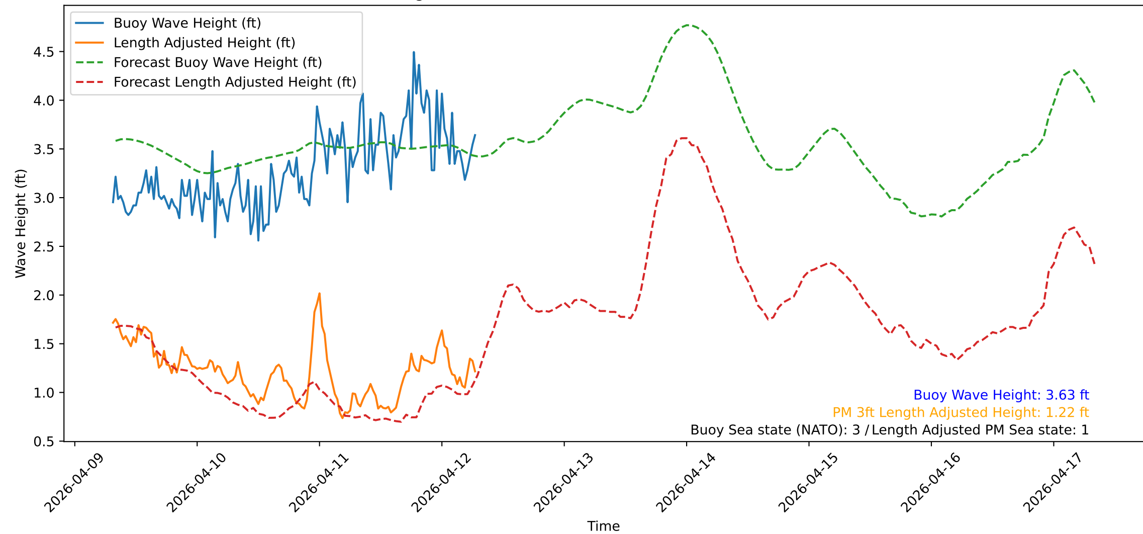
Wave Heights over Time for Green Beach at 2026-04-12 07:31:12
