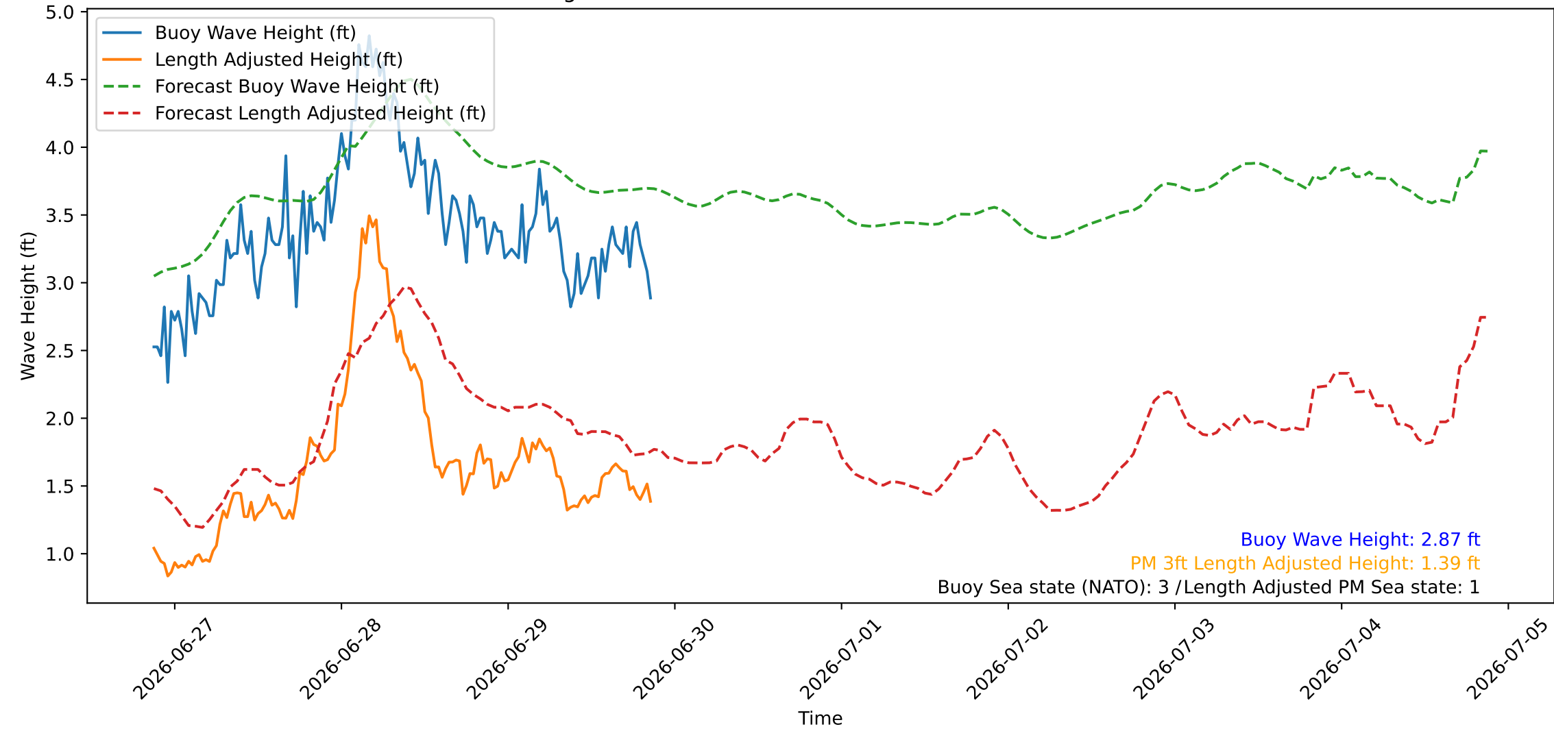
Wave Heights over Time for Green Beach at 2026-06-29 21:11:08
