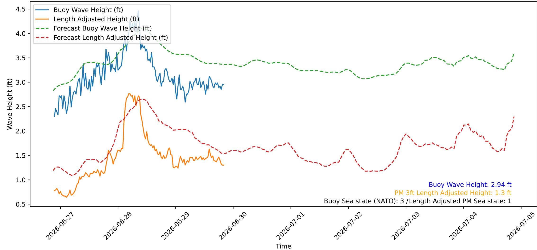
Wave Heights over Time for Red Beach at 2026-06-29 21:10:45
