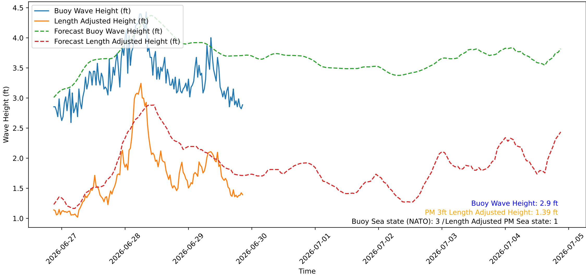
Wave Heights over Time for Oceanside Harbor at 2026-06-29 21:10:26
