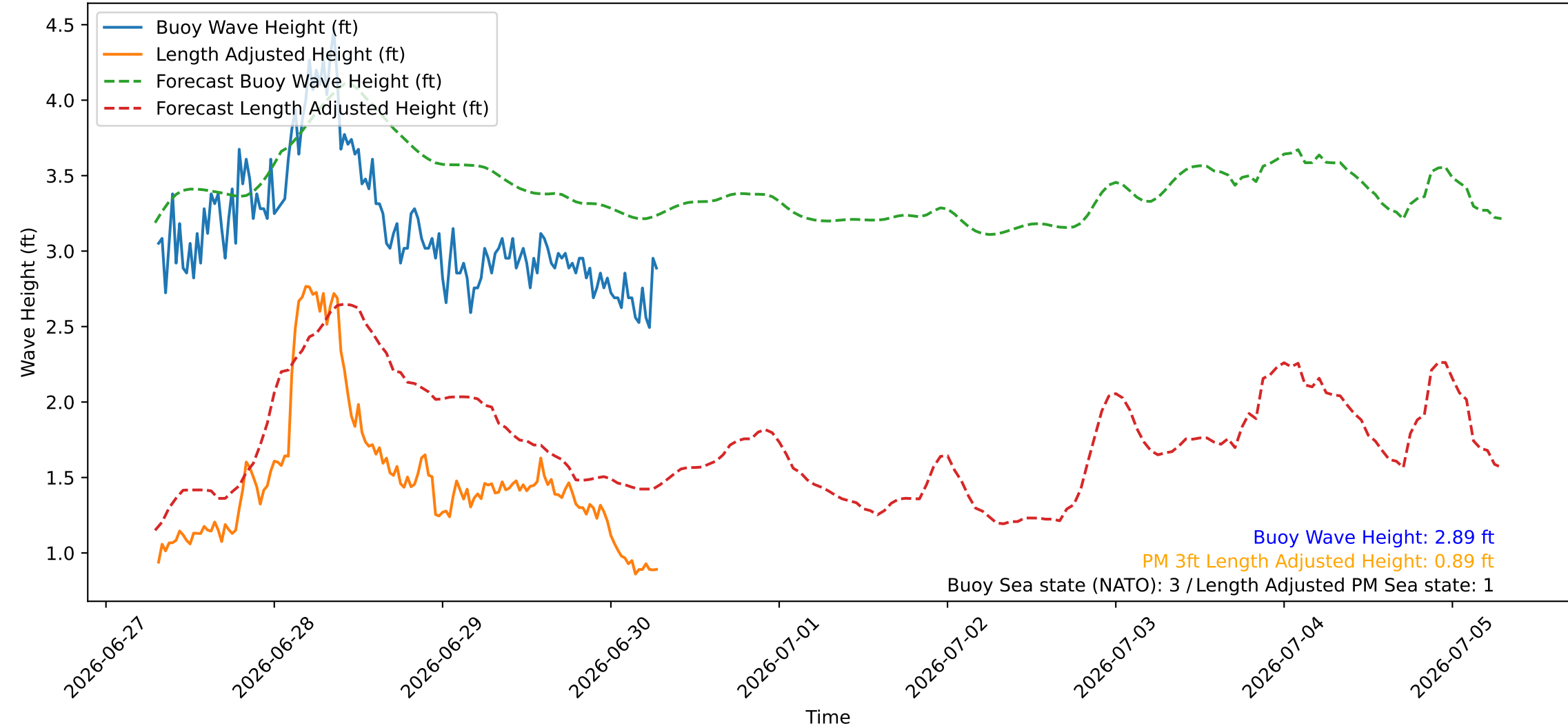
Wave Heights over Time for Red Beach at 2026-06-30 07:20:48
