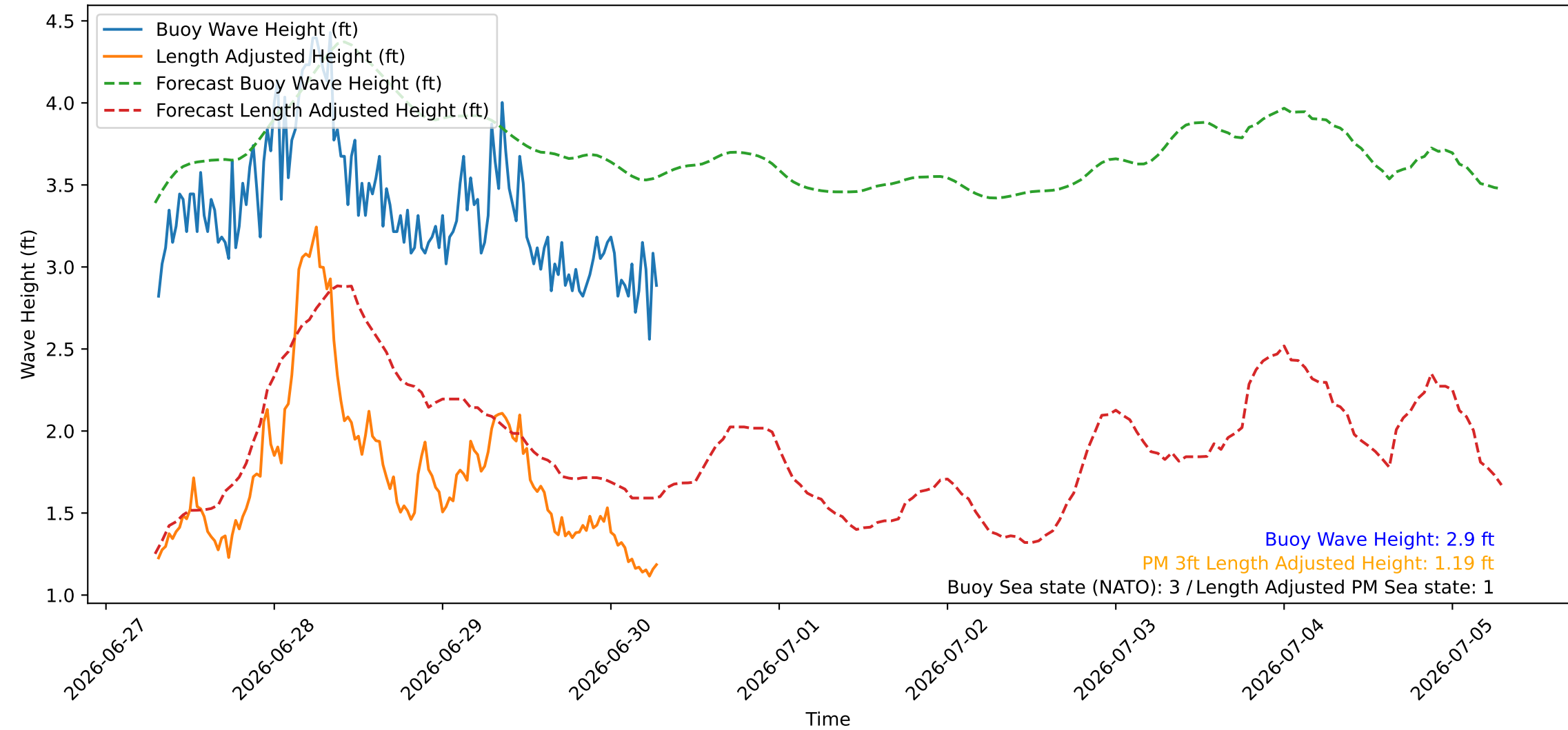
Wave Heights over Time for Oceanside Harbor at 2026-06-30 07:20:26
