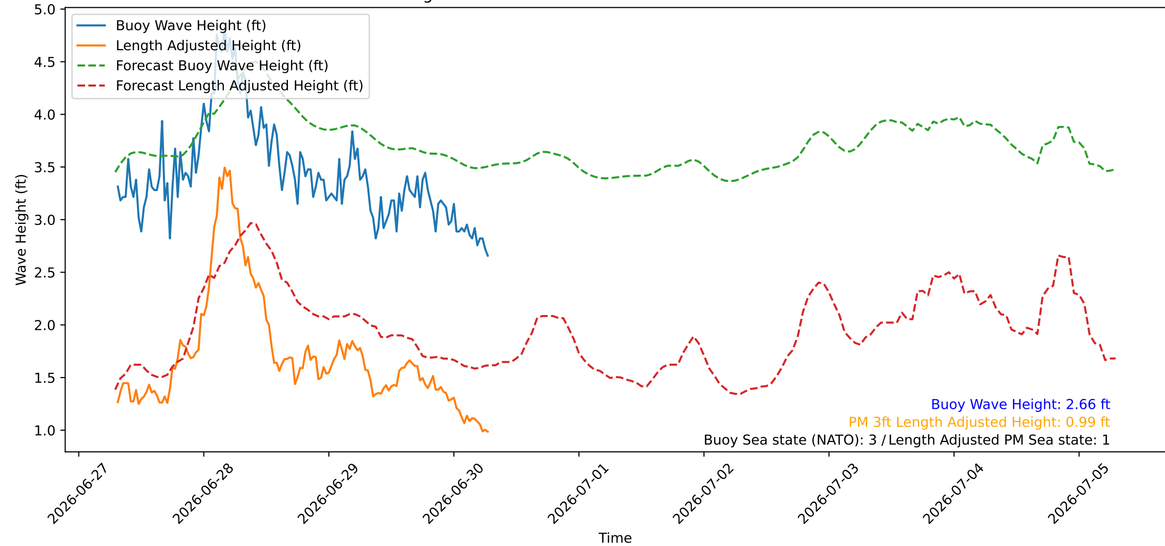
Wave Heights over Time for Green Beach at 2026-06-30 07:21:12
