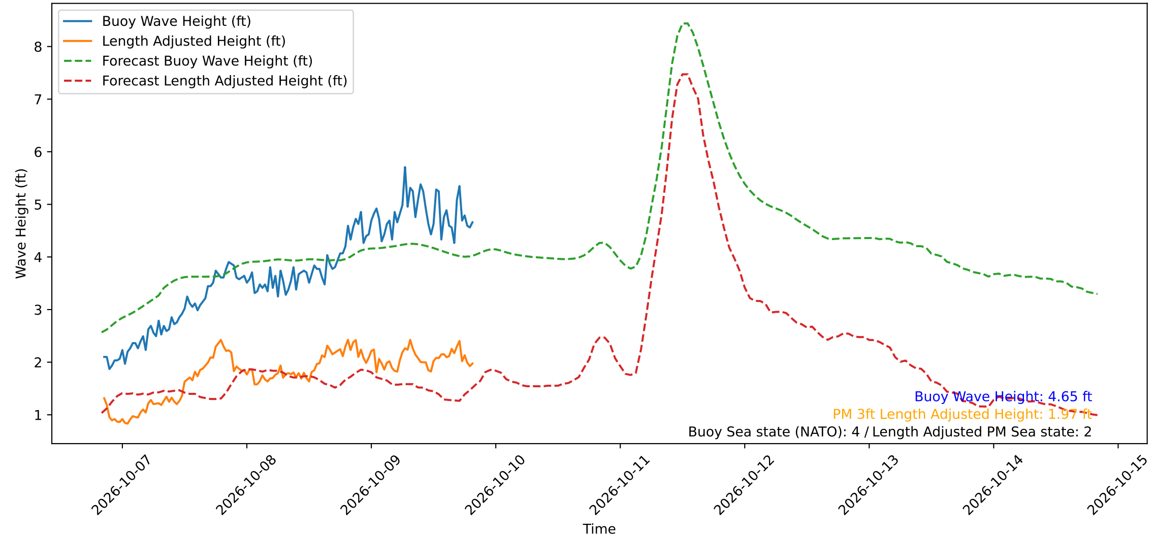
Wave Heights over Time for Red Beach at 2026-10-09 20:20:50
