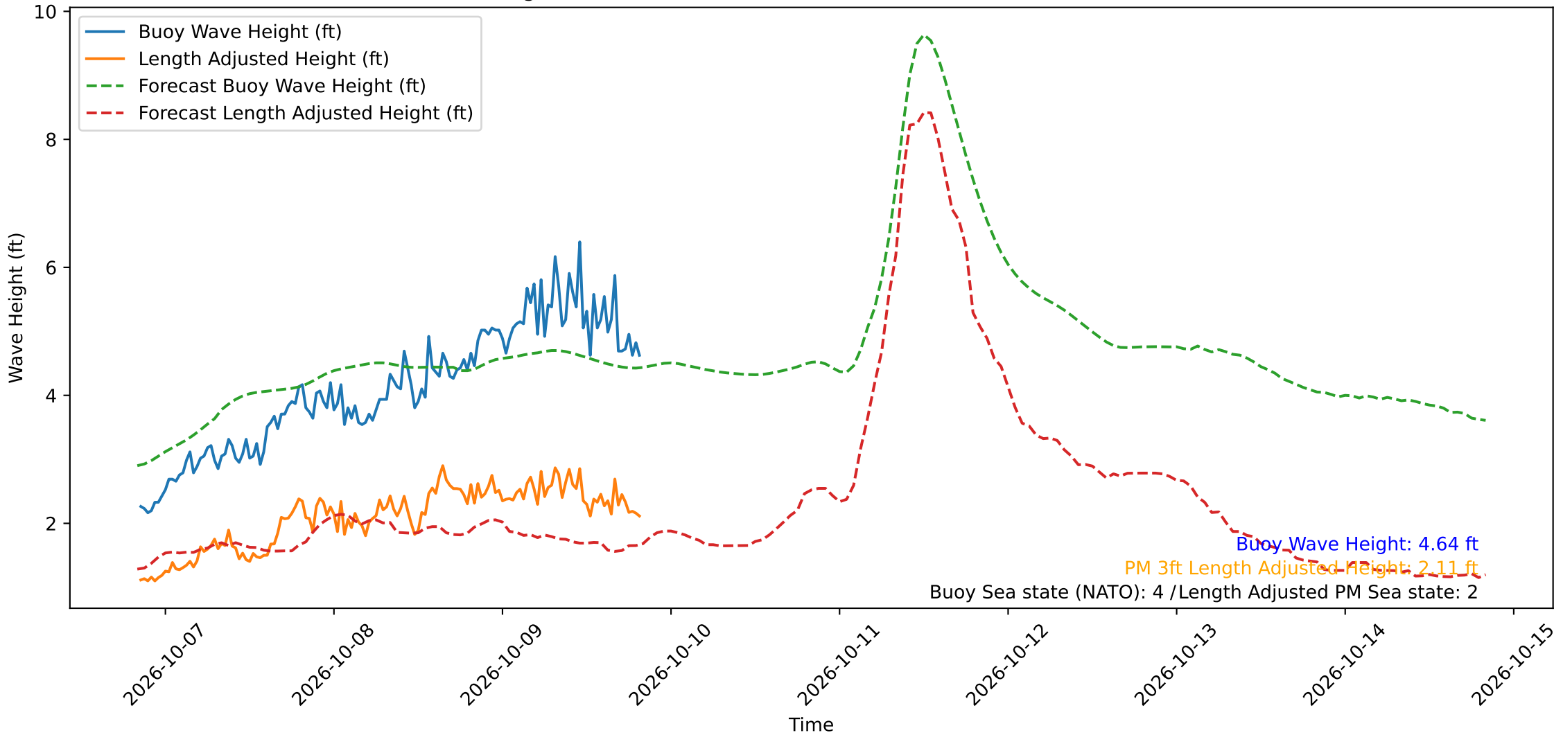
Wave Heights over Time for Oceanside Harbor at 2026-10-09 20:20:29
