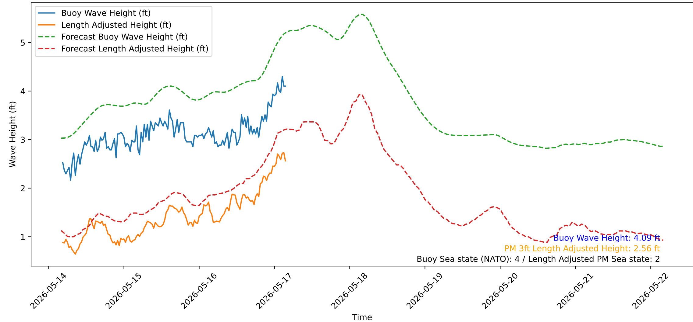
Wave Heights over Time for Oceanside Harbor at 2026-05-17 04:20:31
