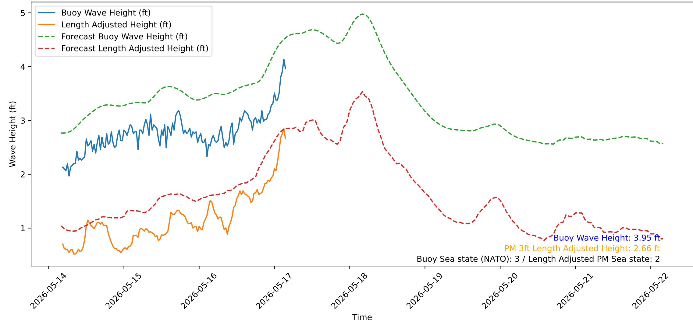
Wave Heights over Time for Red Beach at 2026-05-17 04:20:51
