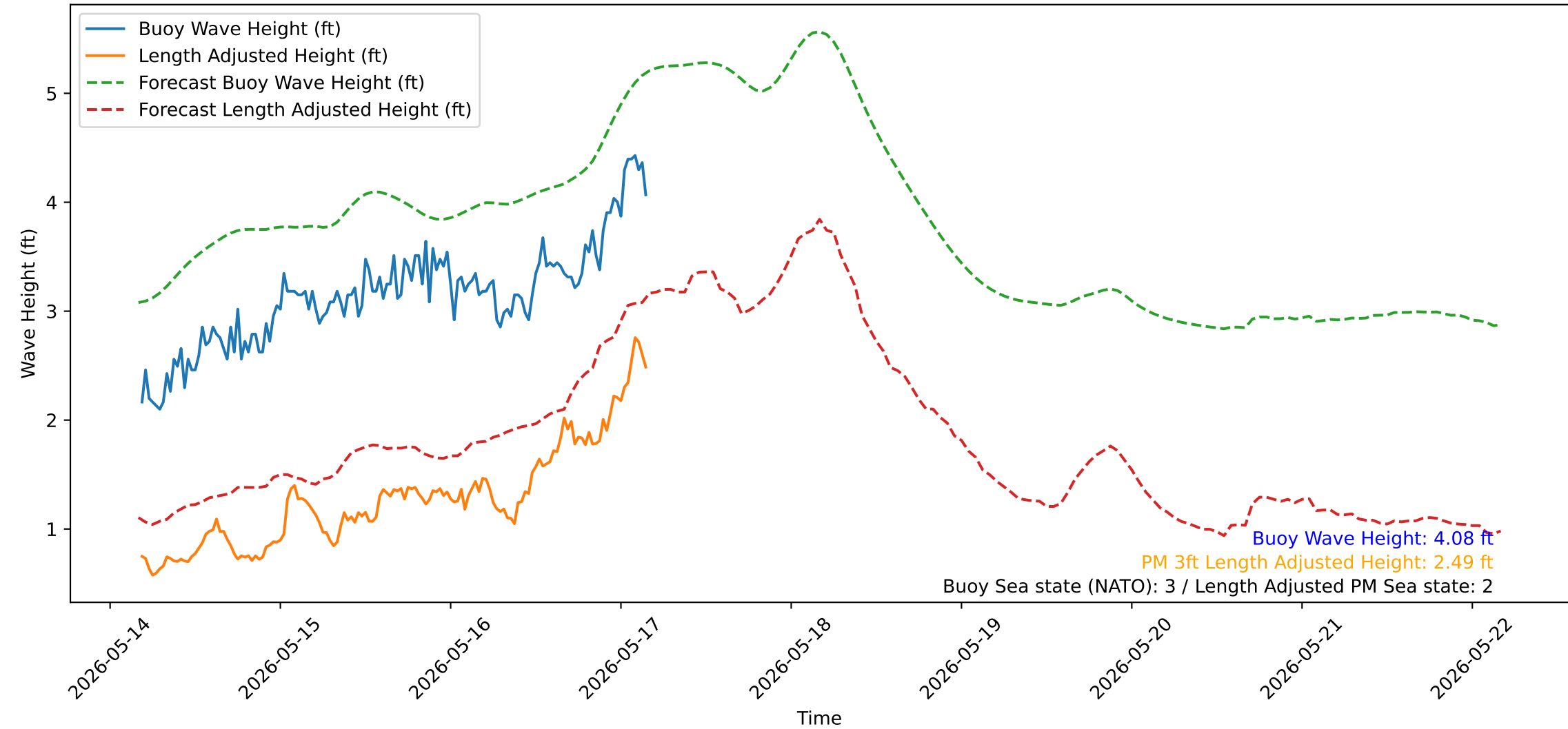
Wave Heights over Time for Green Beach at 2026-05-17 04:21:14
