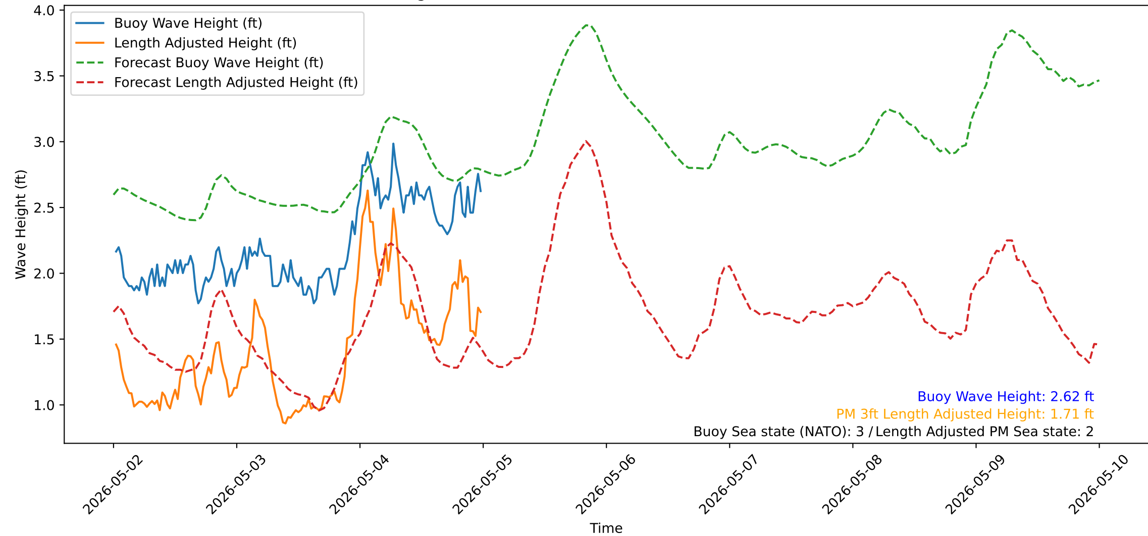
Wave Heights over Time for Green Beach at 2026-05-05 00:21:13
