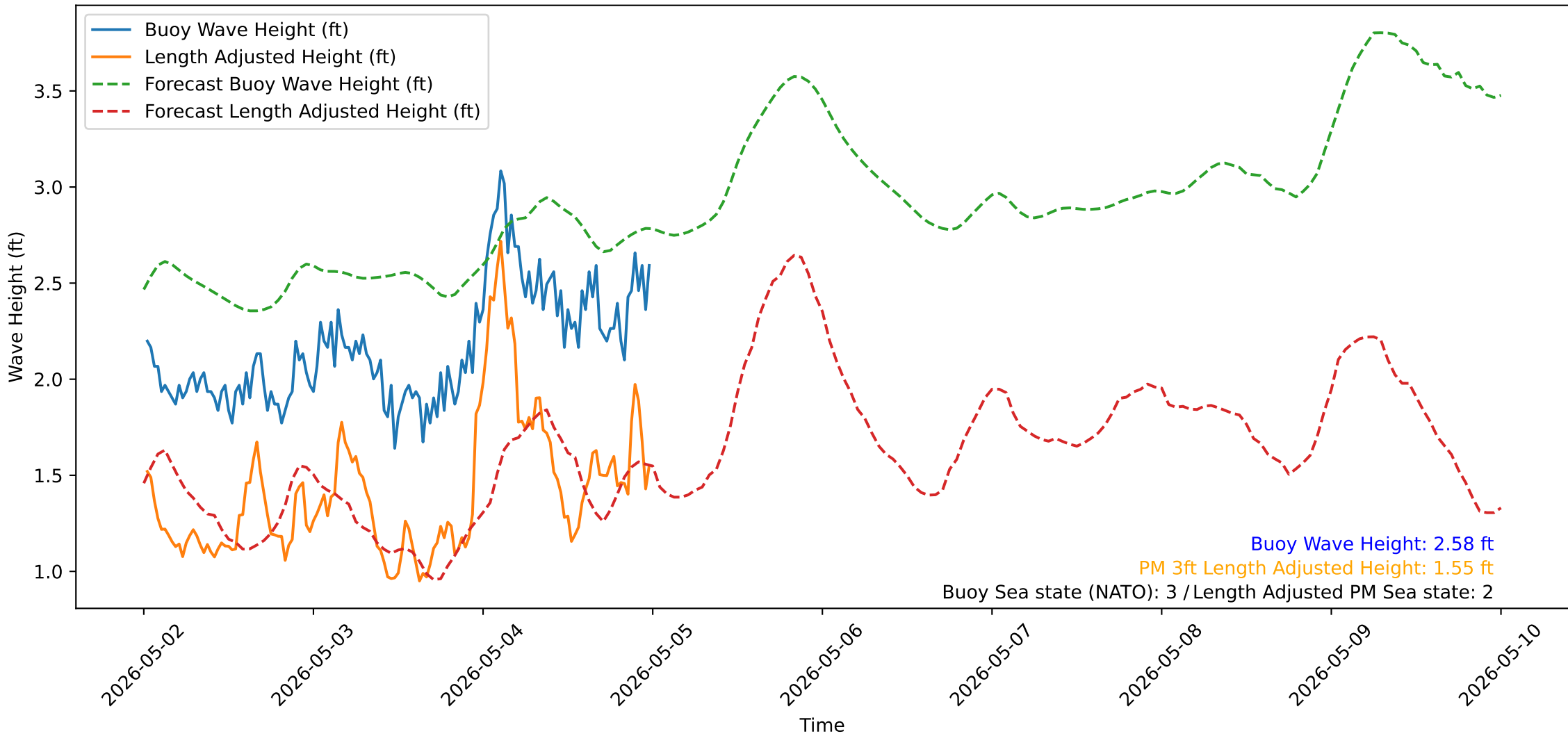
Wave Heights over Time for Oceanside Harbor at 2026-05-05 00:20:31
