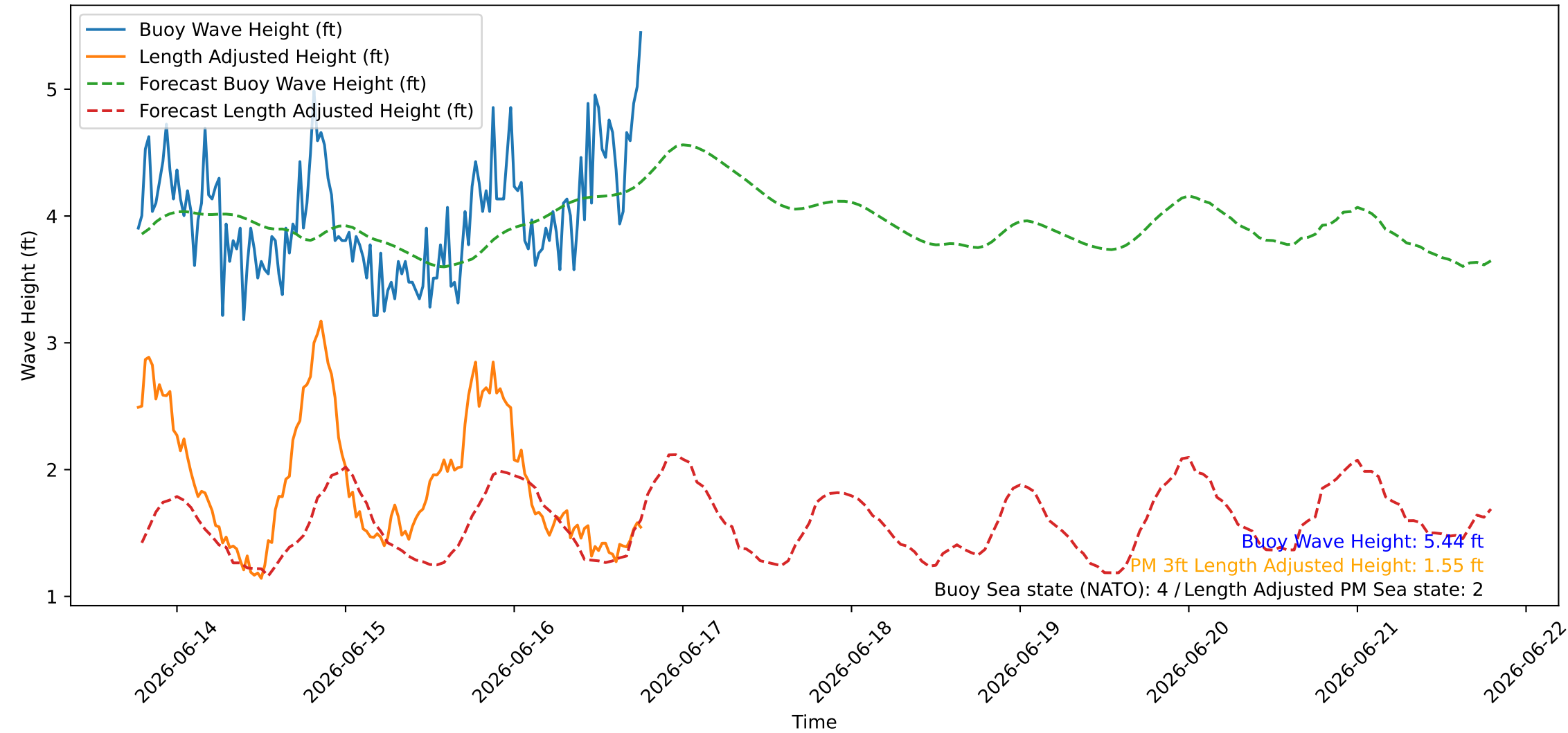
Wave Heights over Time for Oceanside Harbor at 2026-06-16 18:40:27
