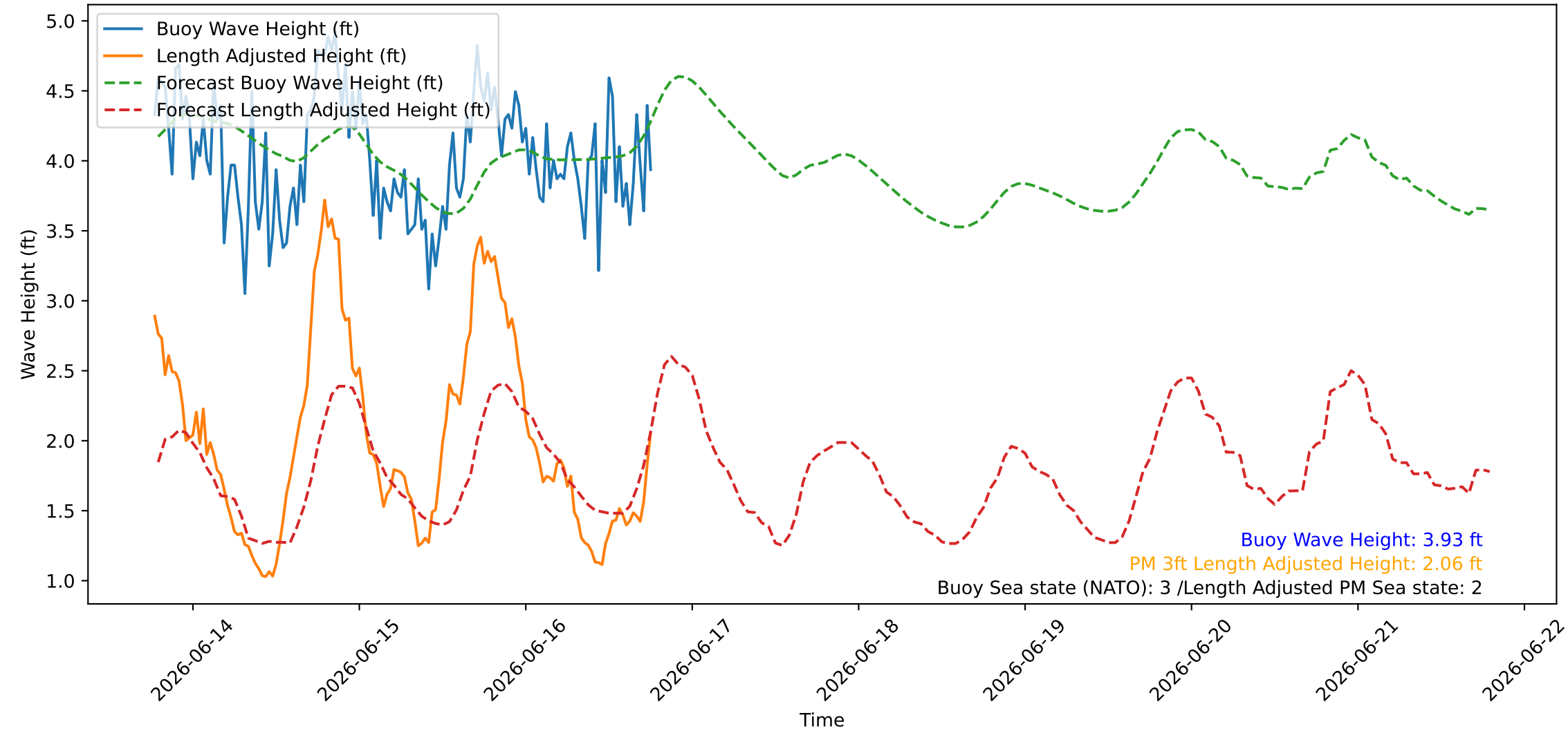
Wave Heights over Time for Green Beach at 2026-06-16 18:41:09
