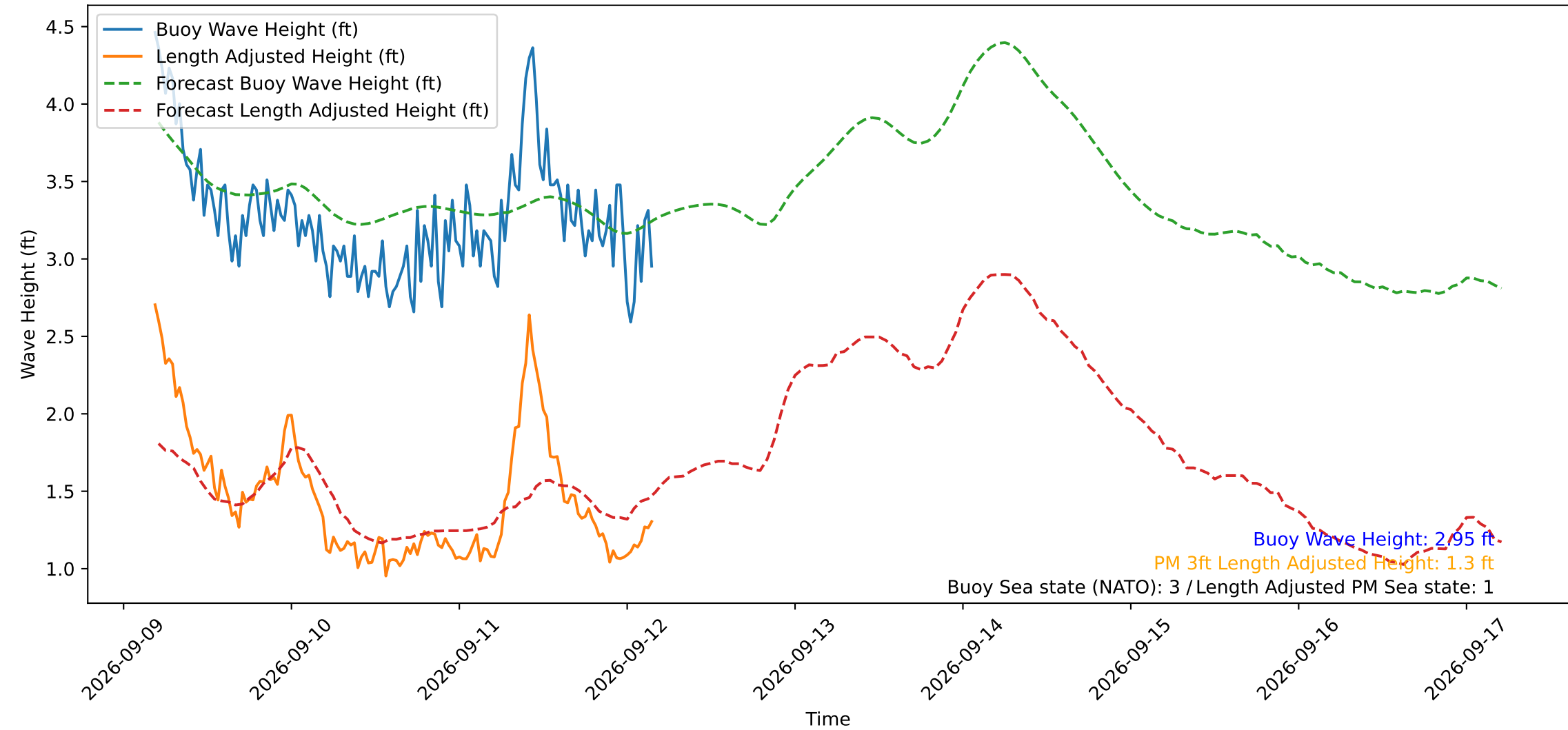
Wave Heights over Time for Oceanside Harbor at 2026-09-12 04:30:30
