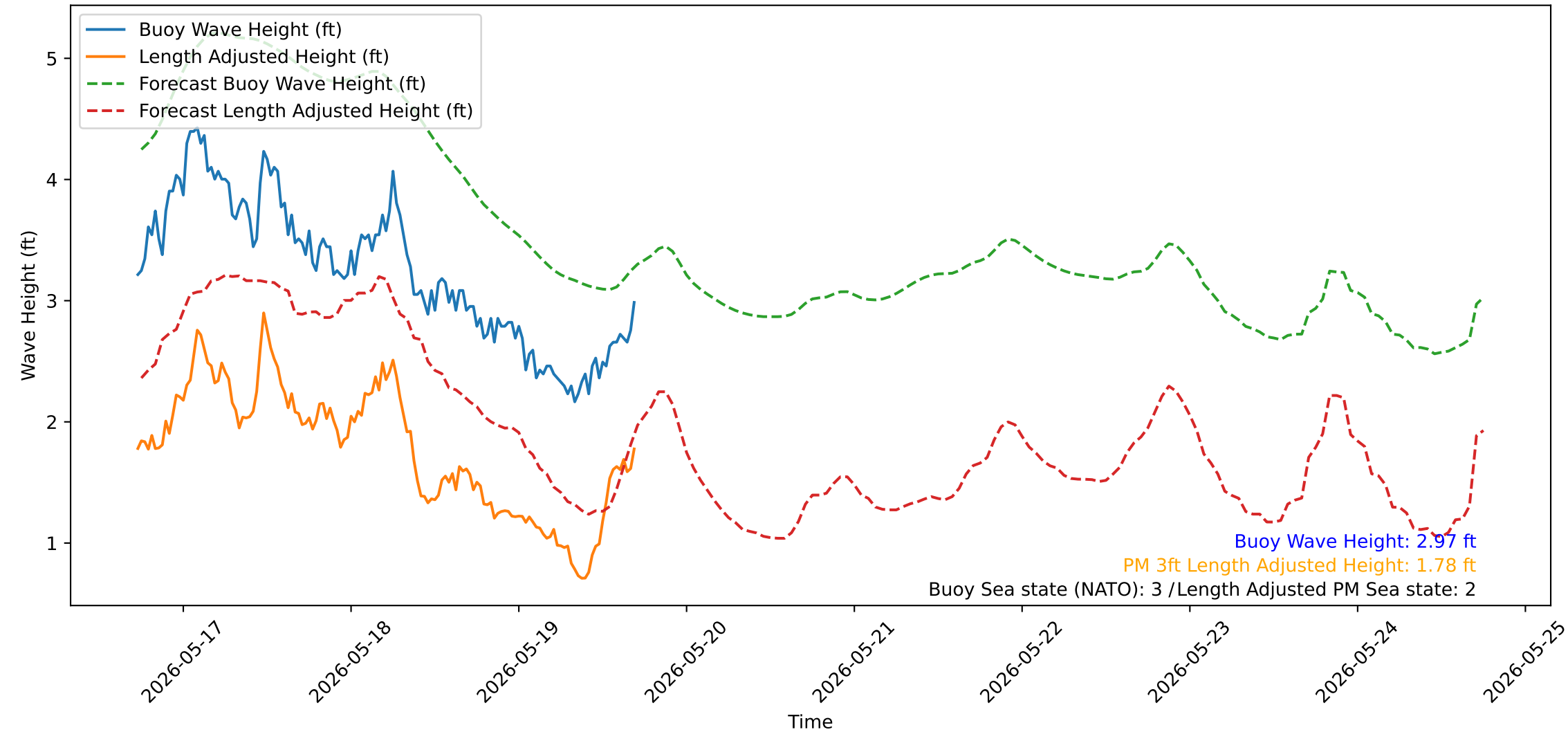
Wave Heights over Time for Green Beach at 2026-05-19 17:31:14
