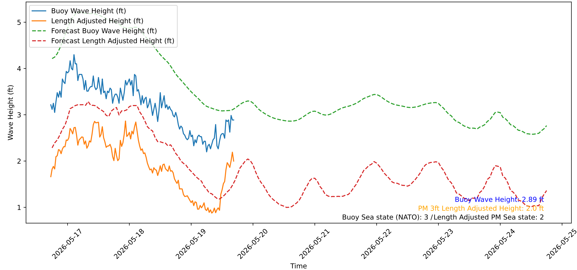
Wave Heights over Time for Oceanside Harbor at 2026-05-19 17:30:32
