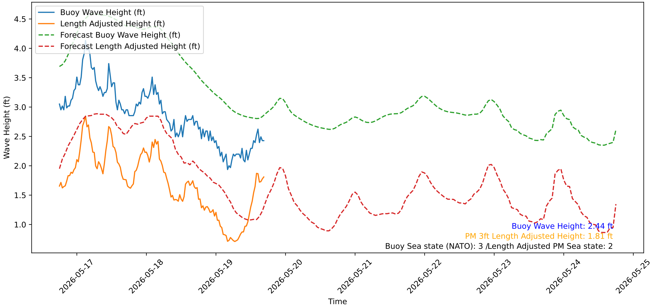
Wave Heights over Time for Red Beach at 2026-05-19 17:30:51
