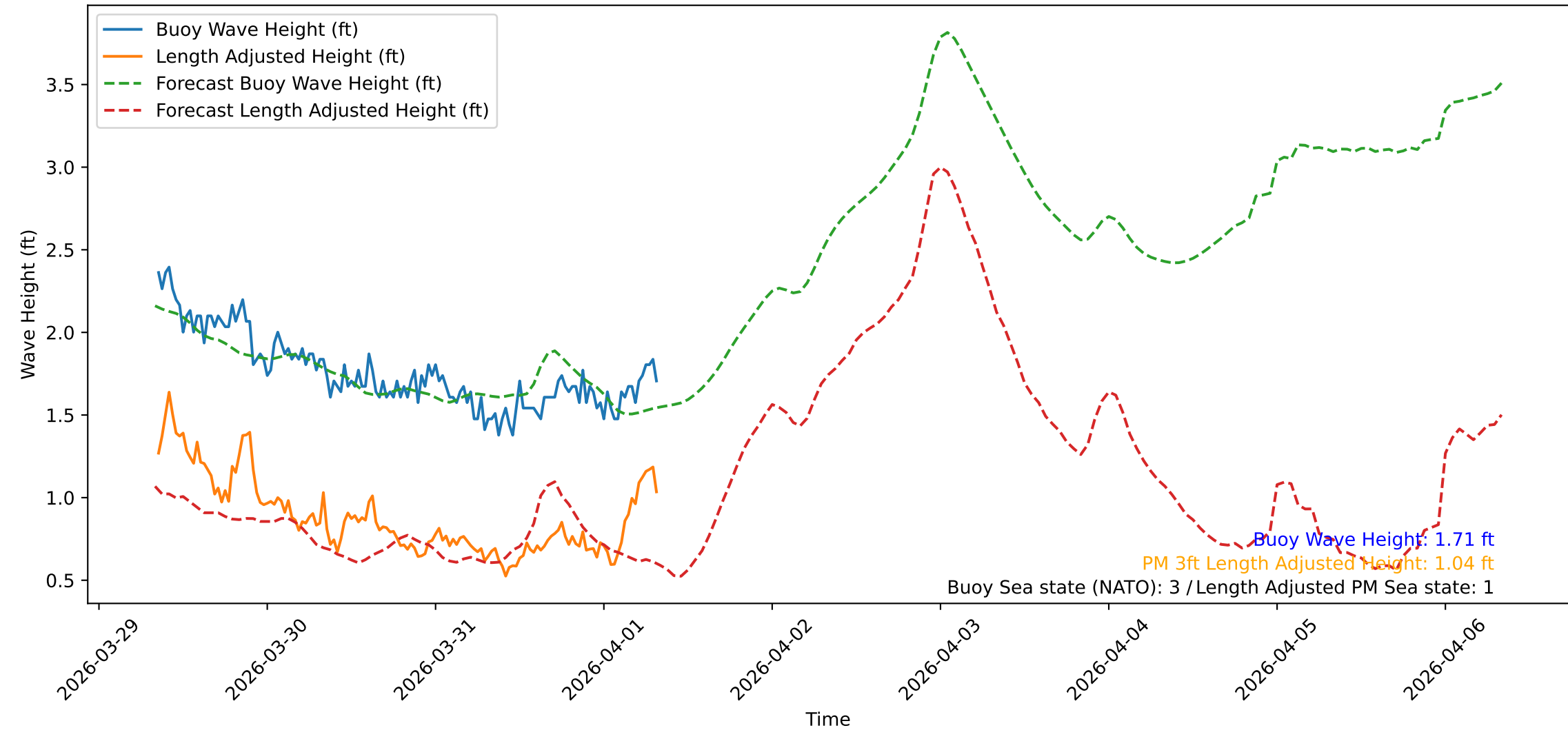
Wave Heights over Time for Red Beach at 2026-04-01 08:20:51
