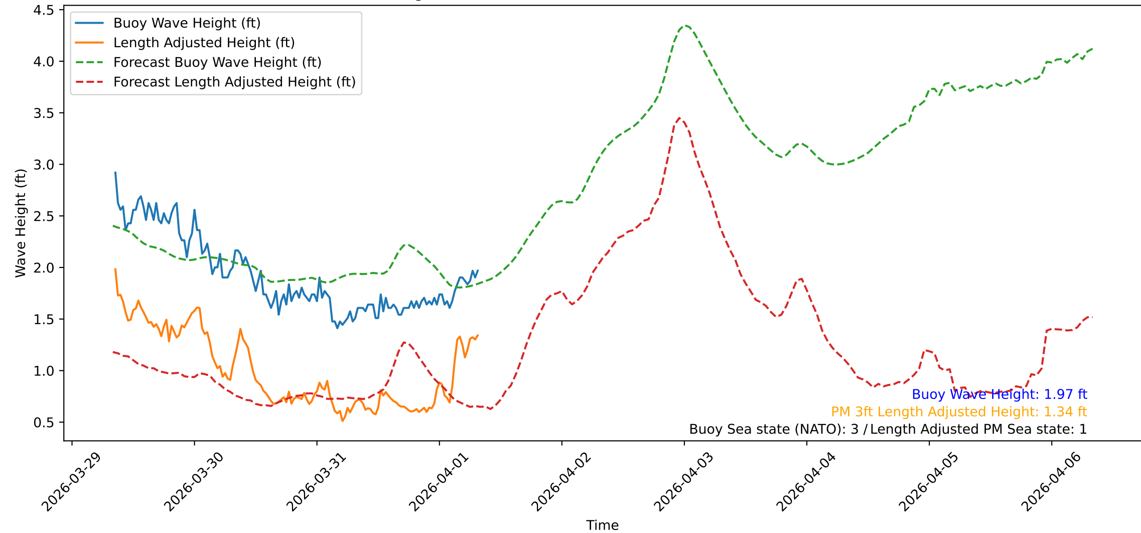
Wave Heights over Time for Green Beach at 2026-04-01 08:21:14
