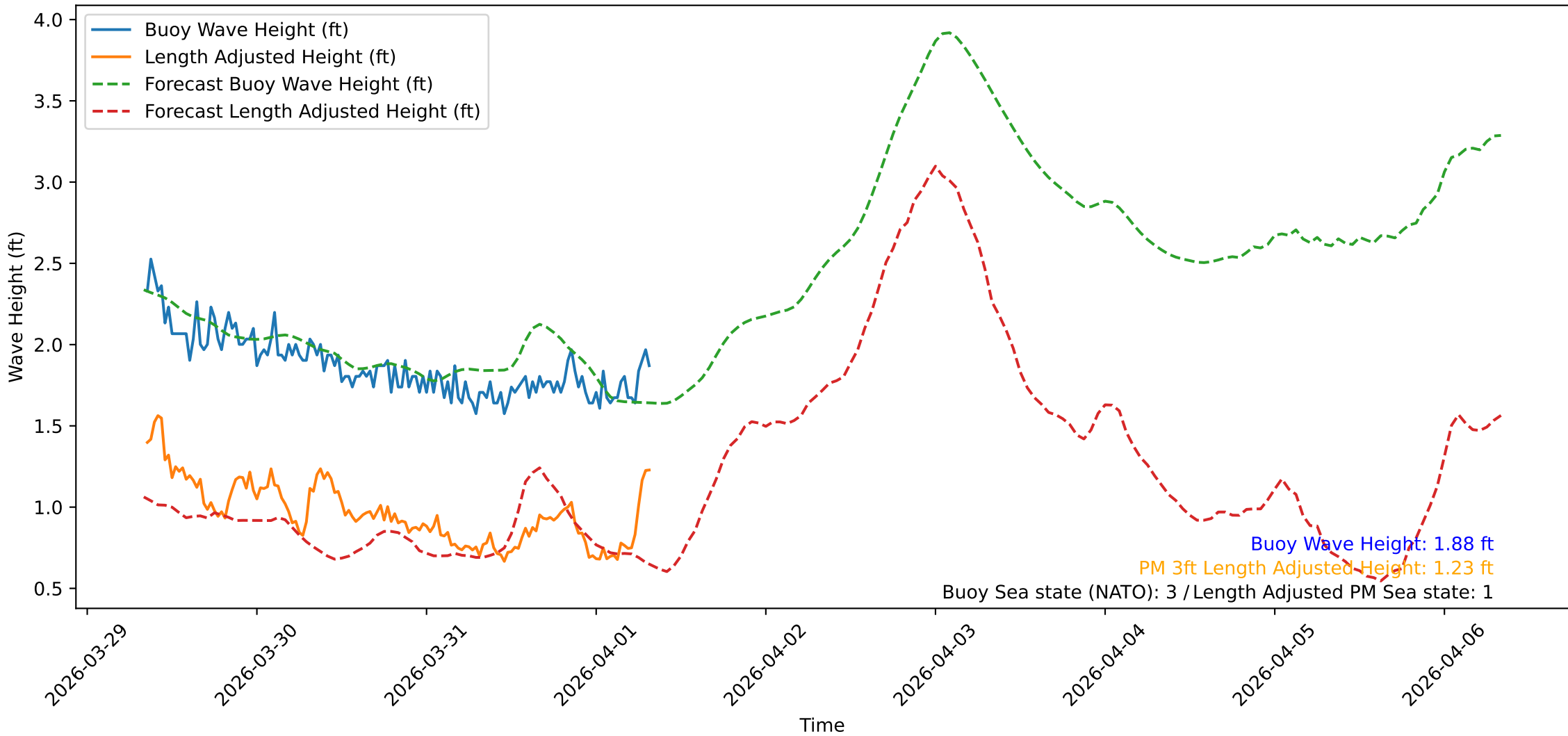
Wave Heights over Time for Oceanside Harbor at 2026-04-01 08:20:35
