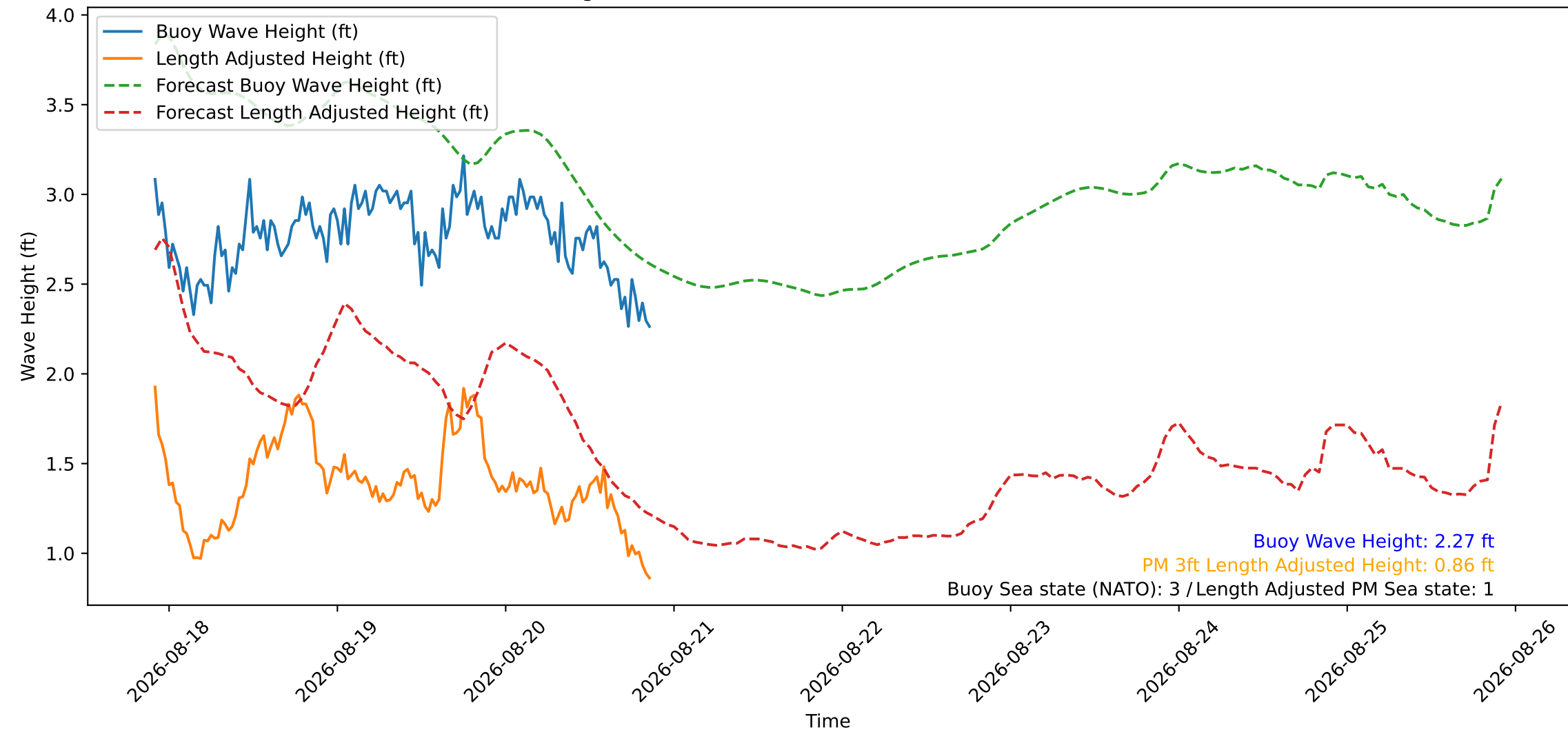
Wave Heights over Time for Red Beach at 2026-08-20 21:30:45
