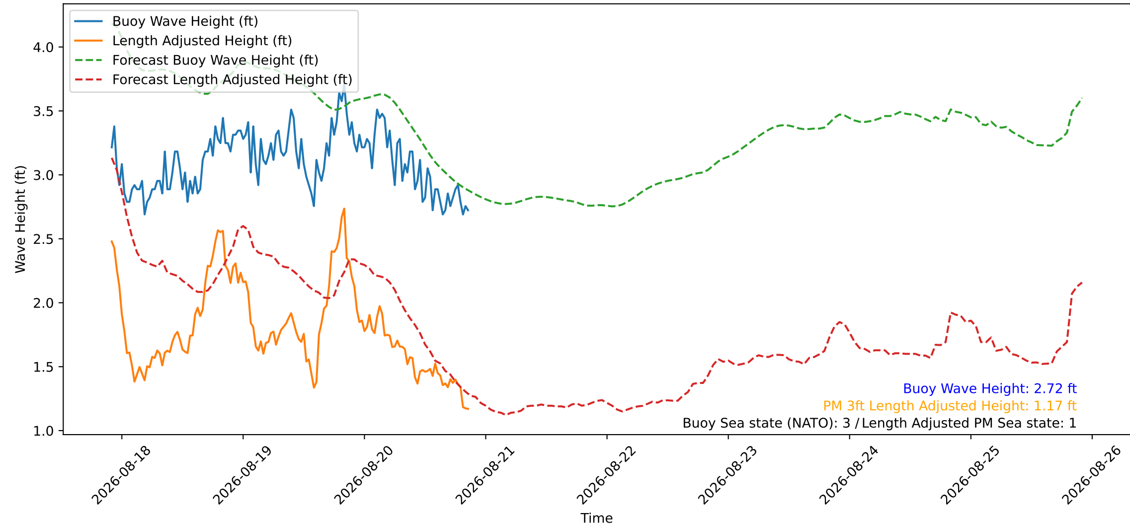
Wave Heights over Time for Green Beach at 2026-08-20 21:31:08
