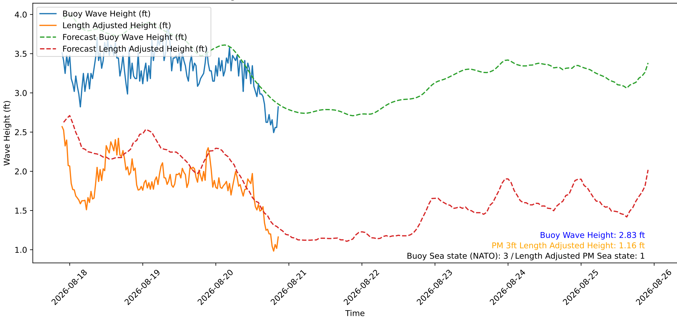
Wave Heights over Time for Oceanside Harbor at 2026-08-20 21:30:26
