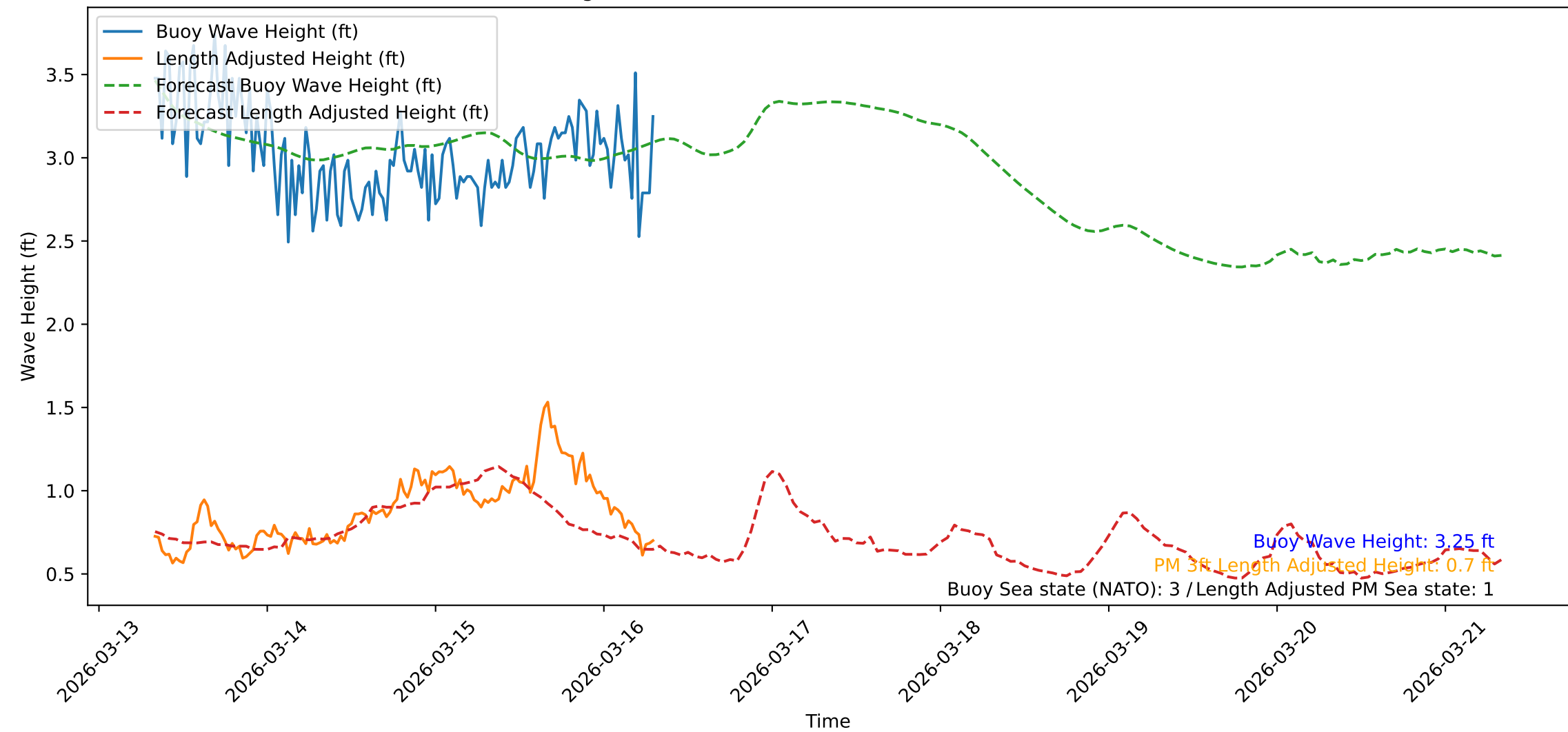
Wave Heights over Time for Red Beach at 2026-03-16 07:41:12
