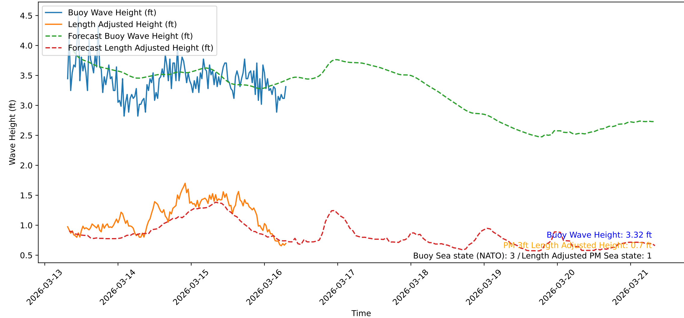
Wave Heights over Time for Green Beach at 2026-03-16 07:41:46
