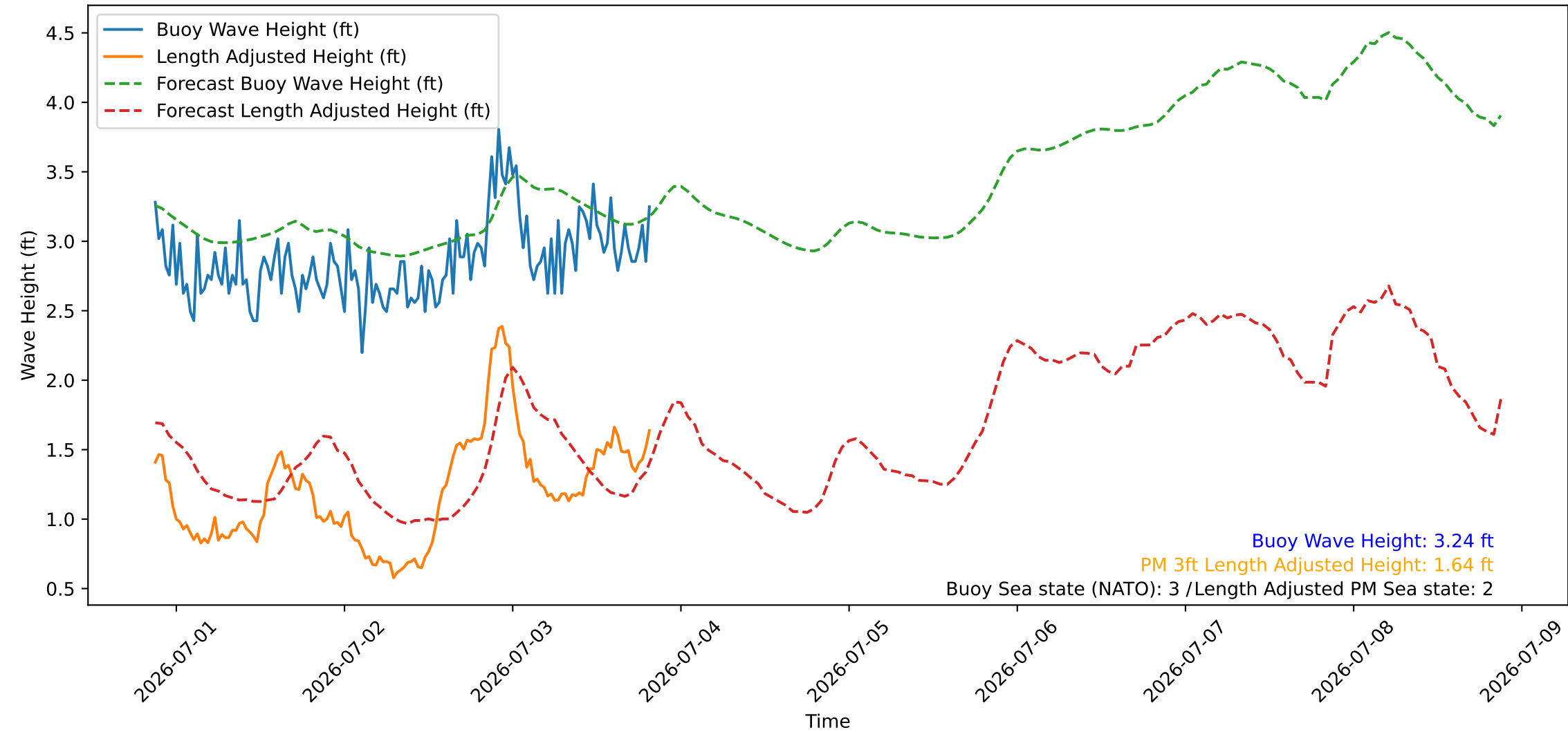
Wave Heights over Time for Red Beach at 2026-07-03 20:30:45
