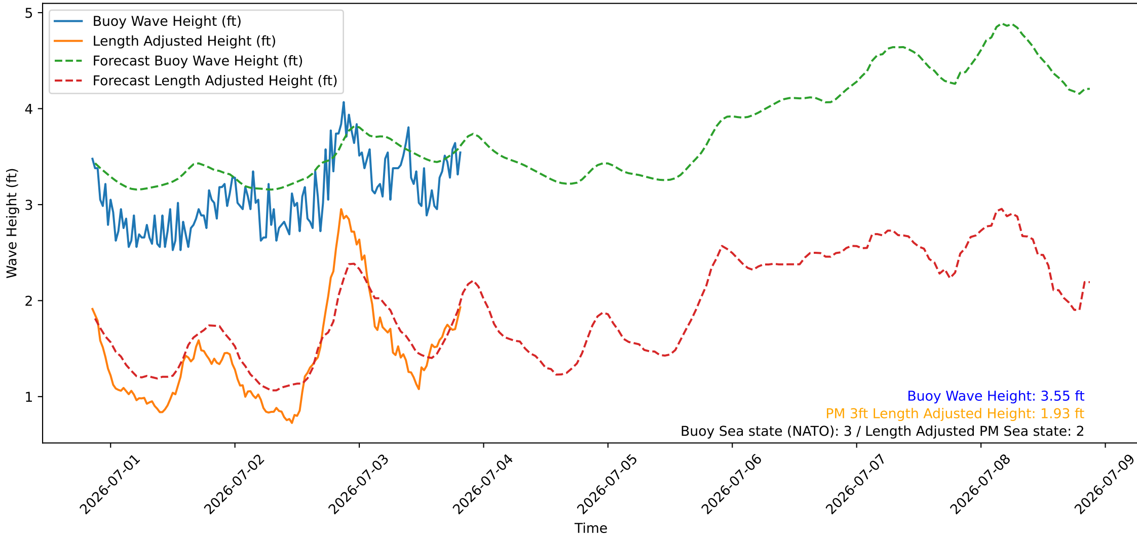
Wave Heights over Time for Green Beach at 2026-07-03 20:31:08
