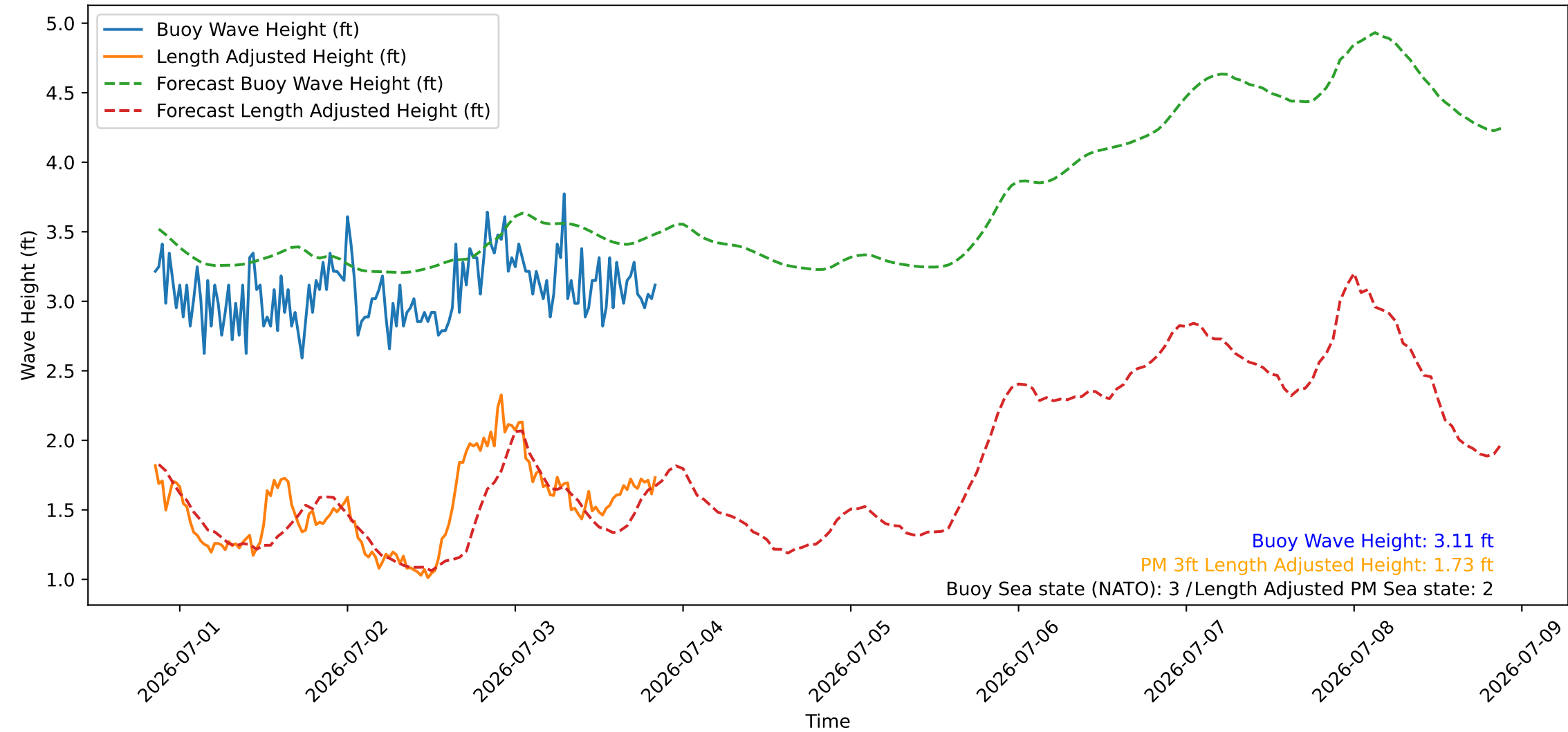
Wave Heights over Time for Oceanside Harbor at 2026-07-03 20:30:26
