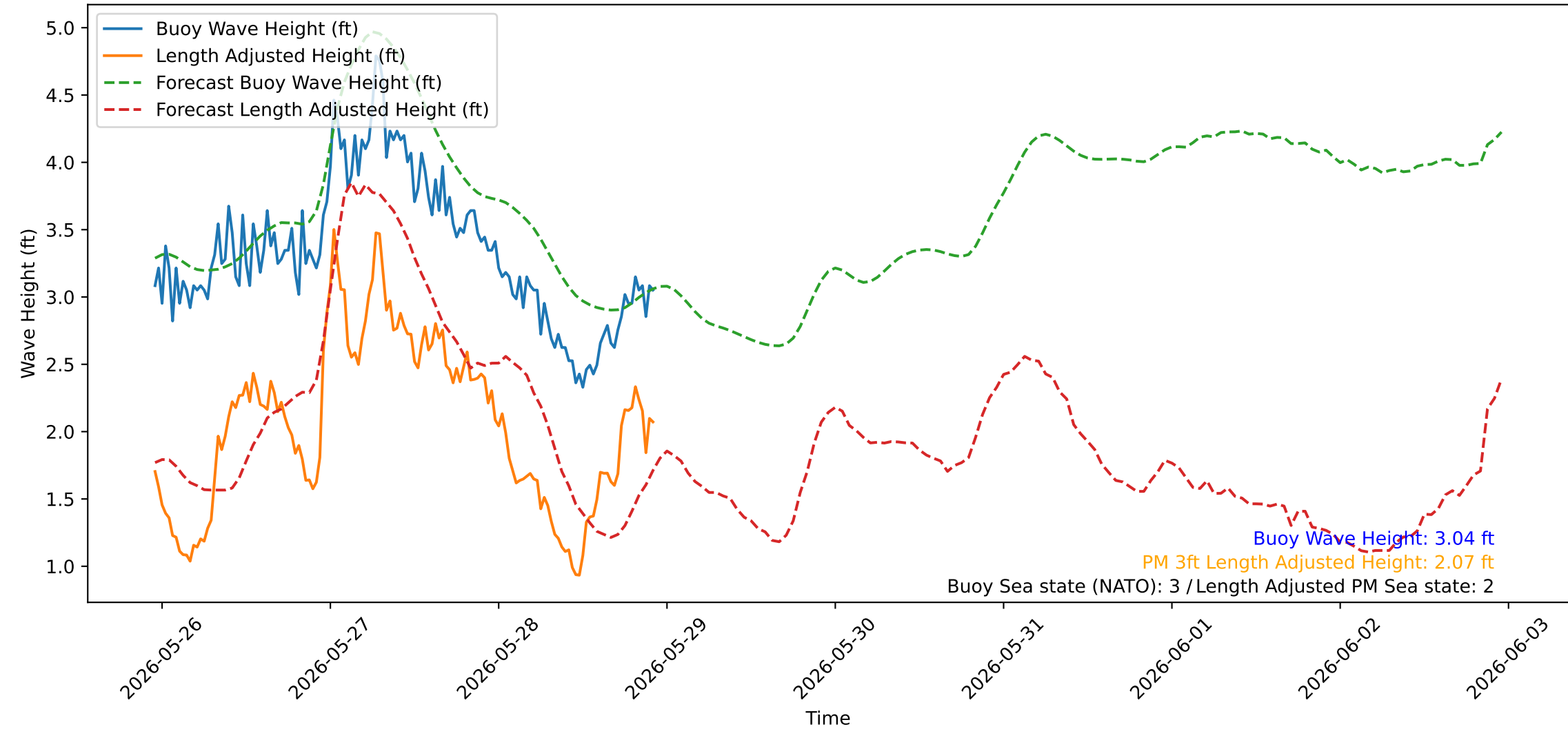
Wave Heights over Time for Red Beach at 2026-05-28 22:40:39
