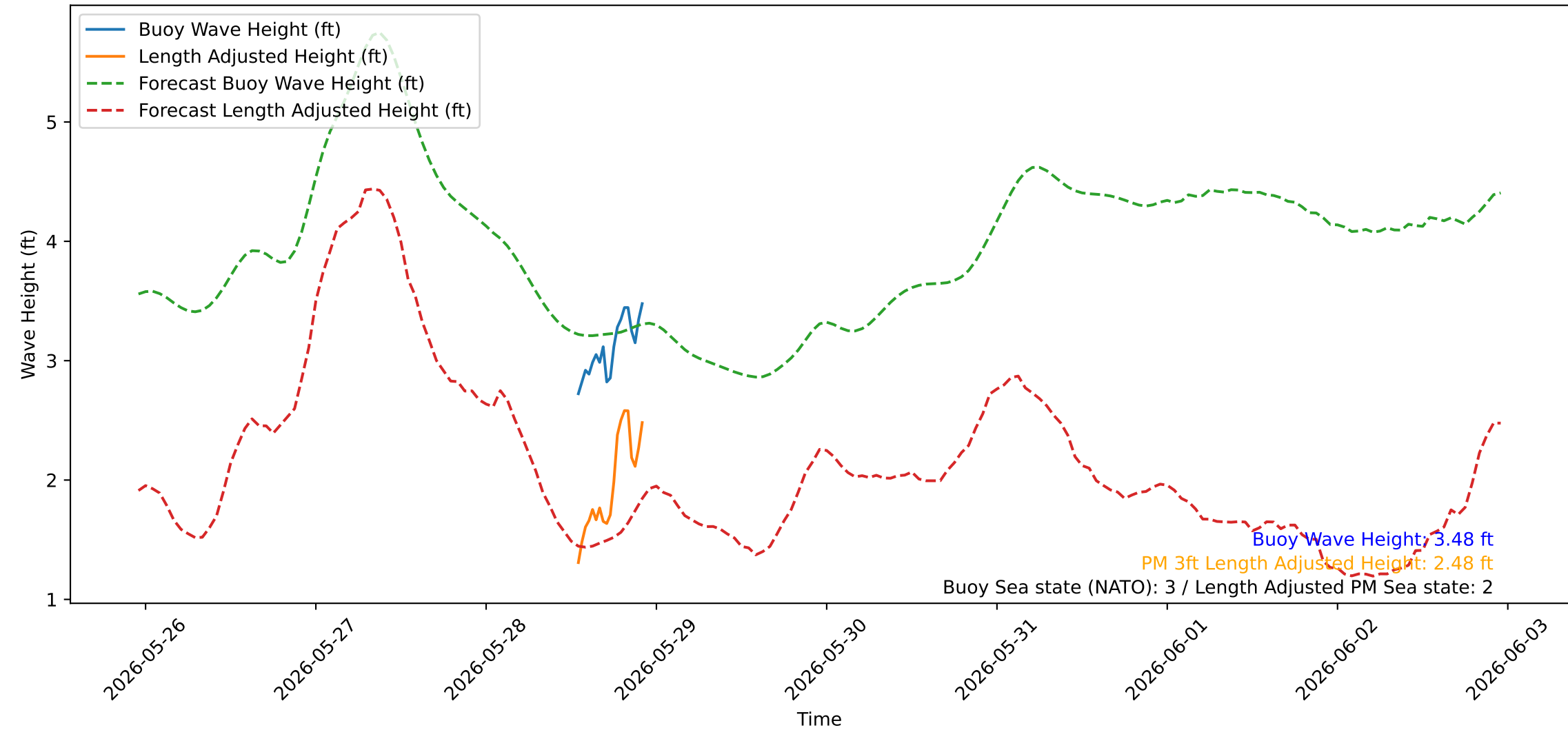
Wave Heights over Time for Oceanside Harbor at 2026-05-28 22:40:20
