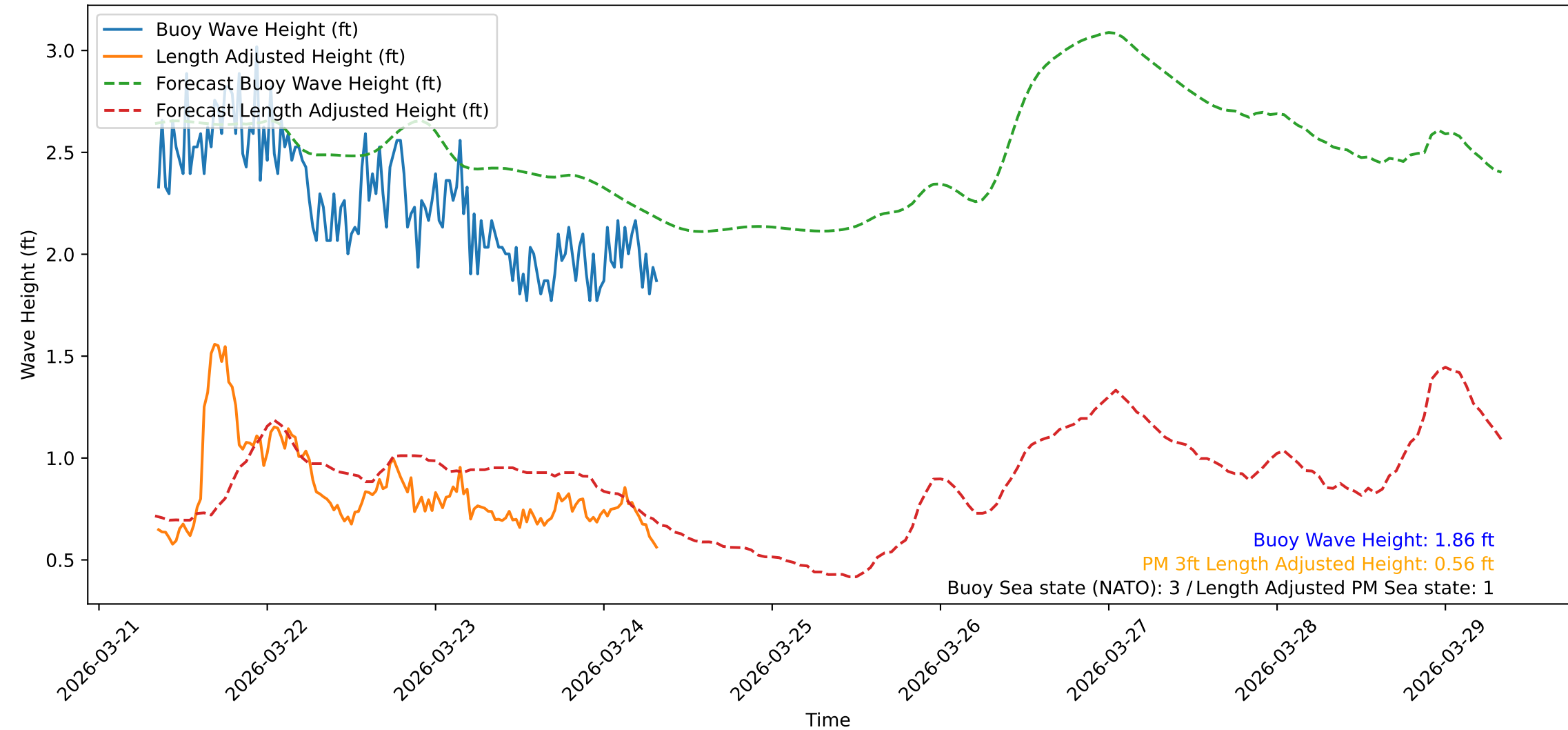
Wave Heights over Time for Oceanside Harbor at 2026-03-24 08:20:31
