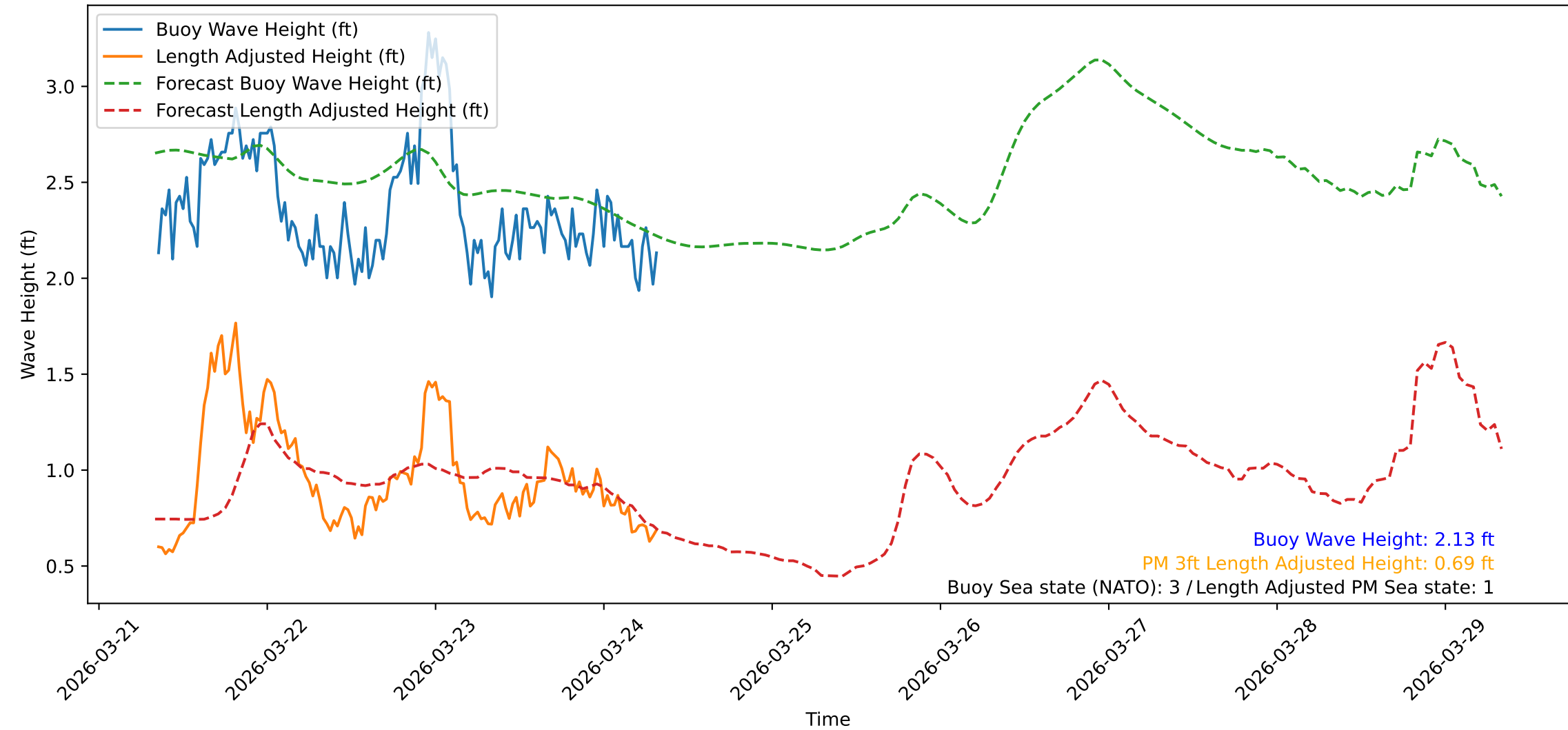
Wave Heights over Time for Green Beach at 2026-03-24 08:21:10
