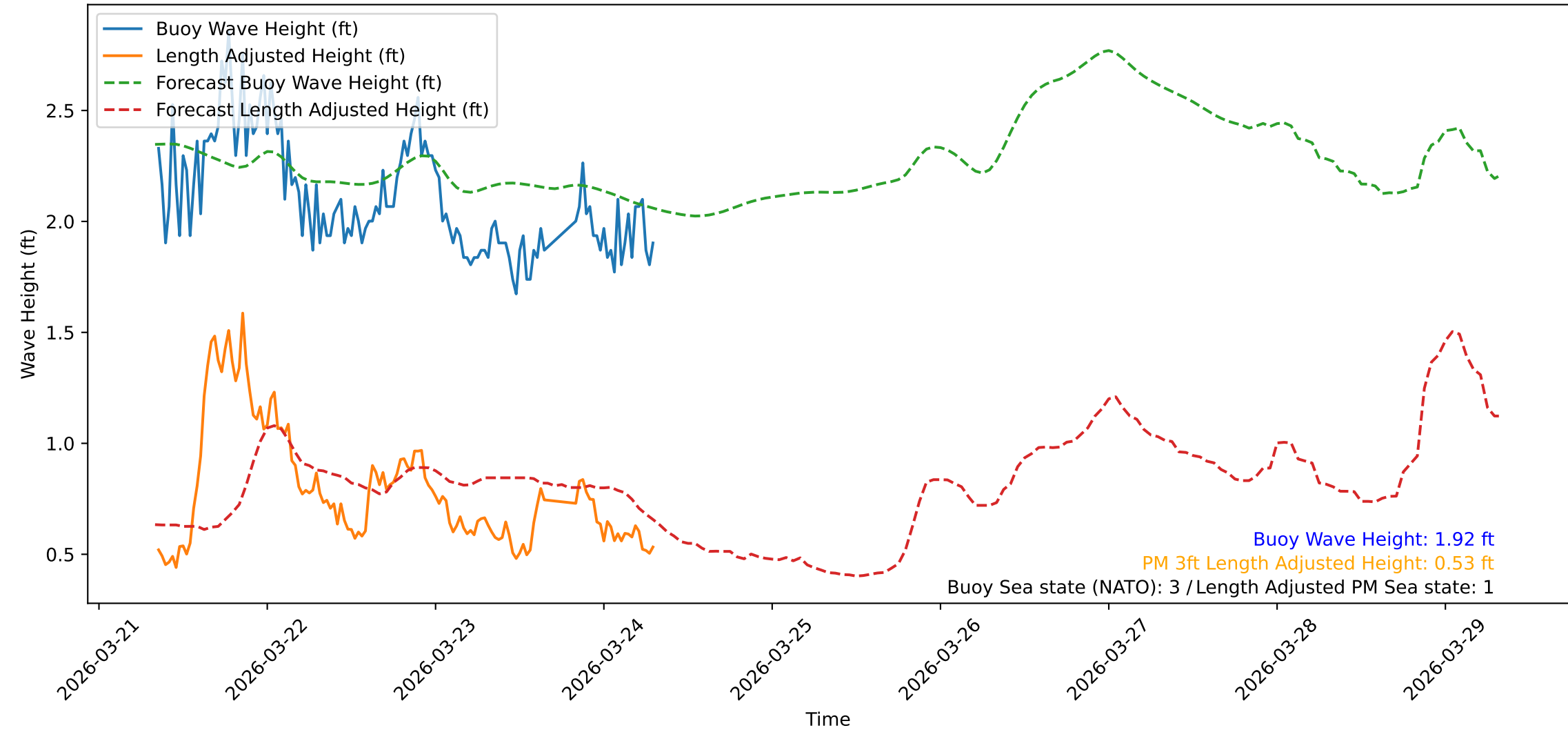
Wave Heights over Time for Red Beach at 2026-03-24 08:20:47
