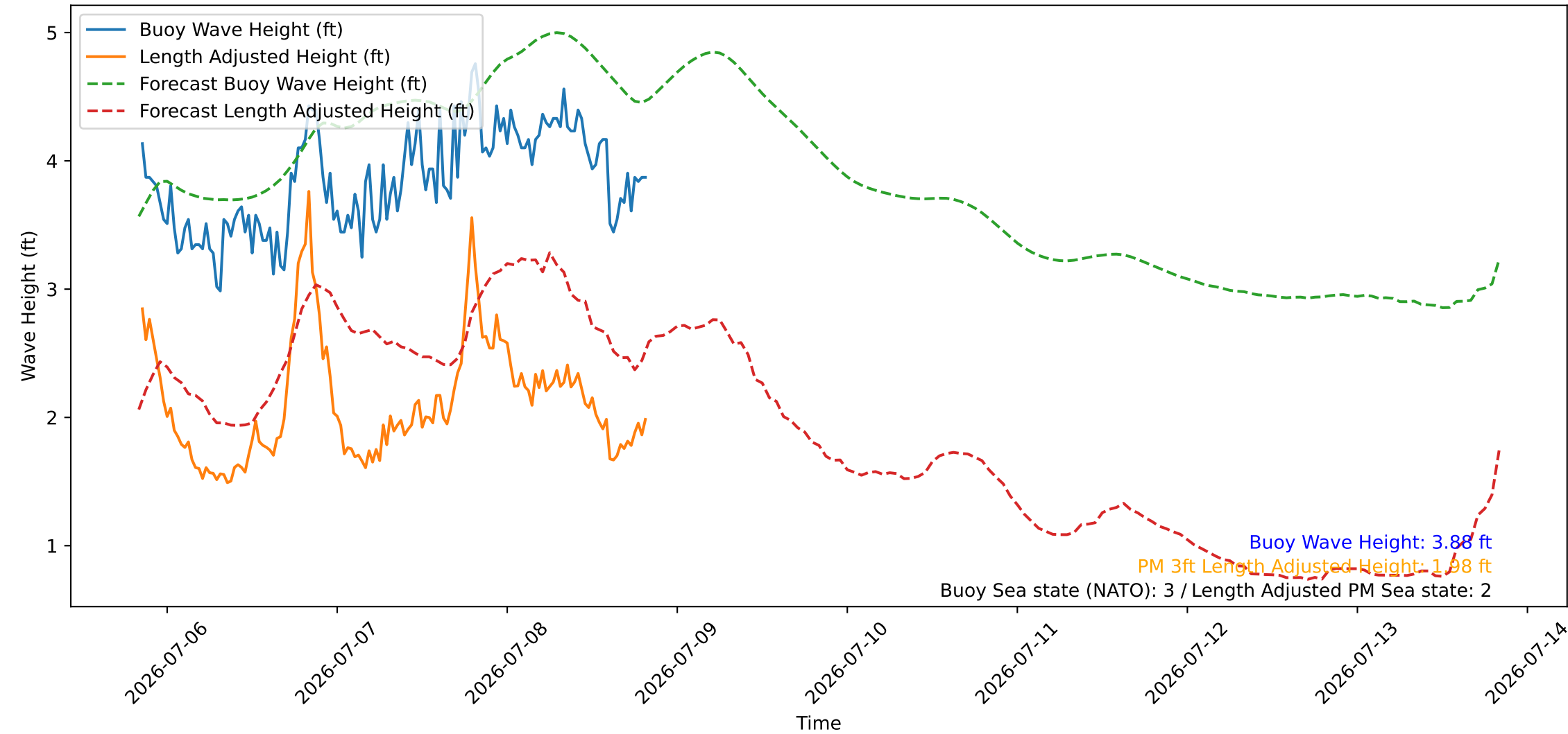
Wave Heights over Time for Green Beach at 2026-07-08 20:21:08
