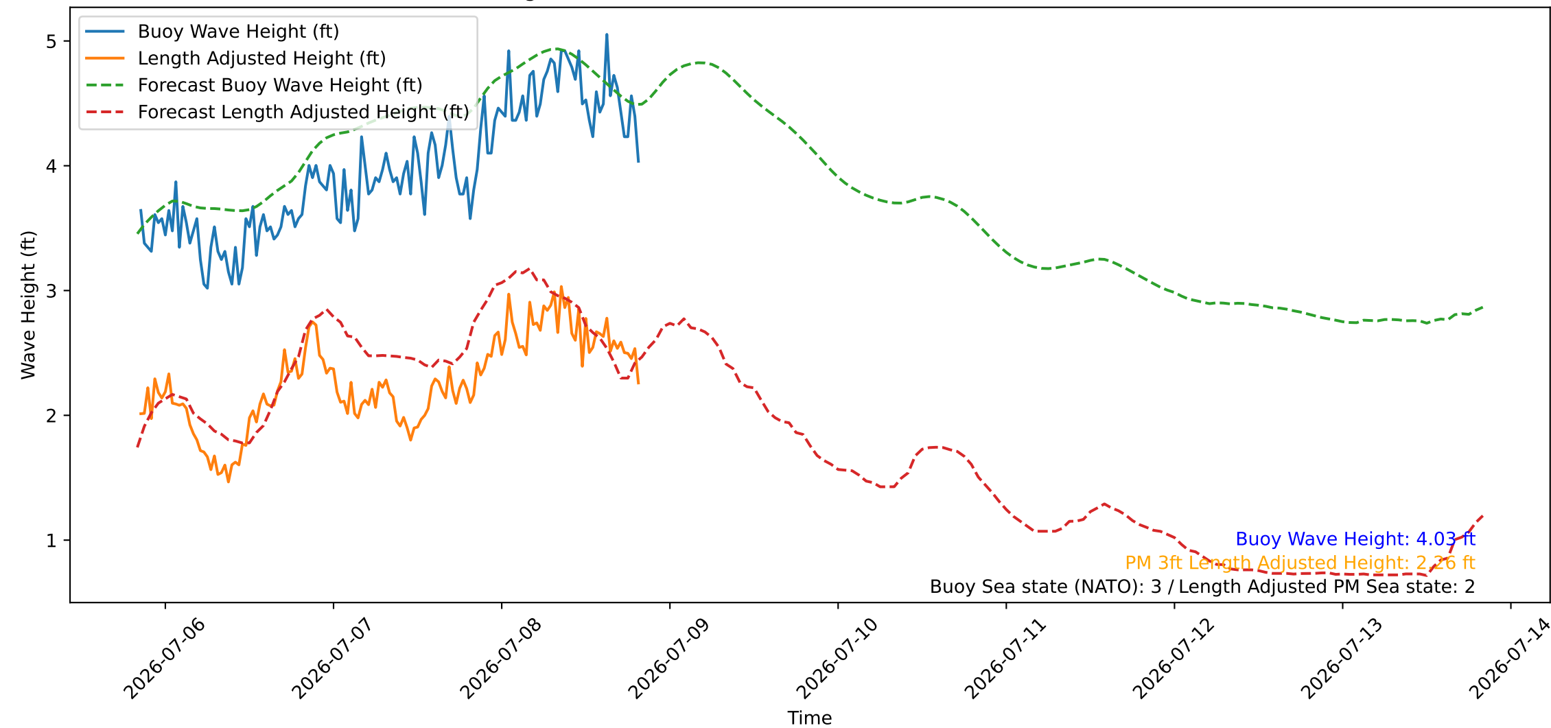
Wave Heights over Time for Oceanside Harbor at 2026-07-08 20:20:26
