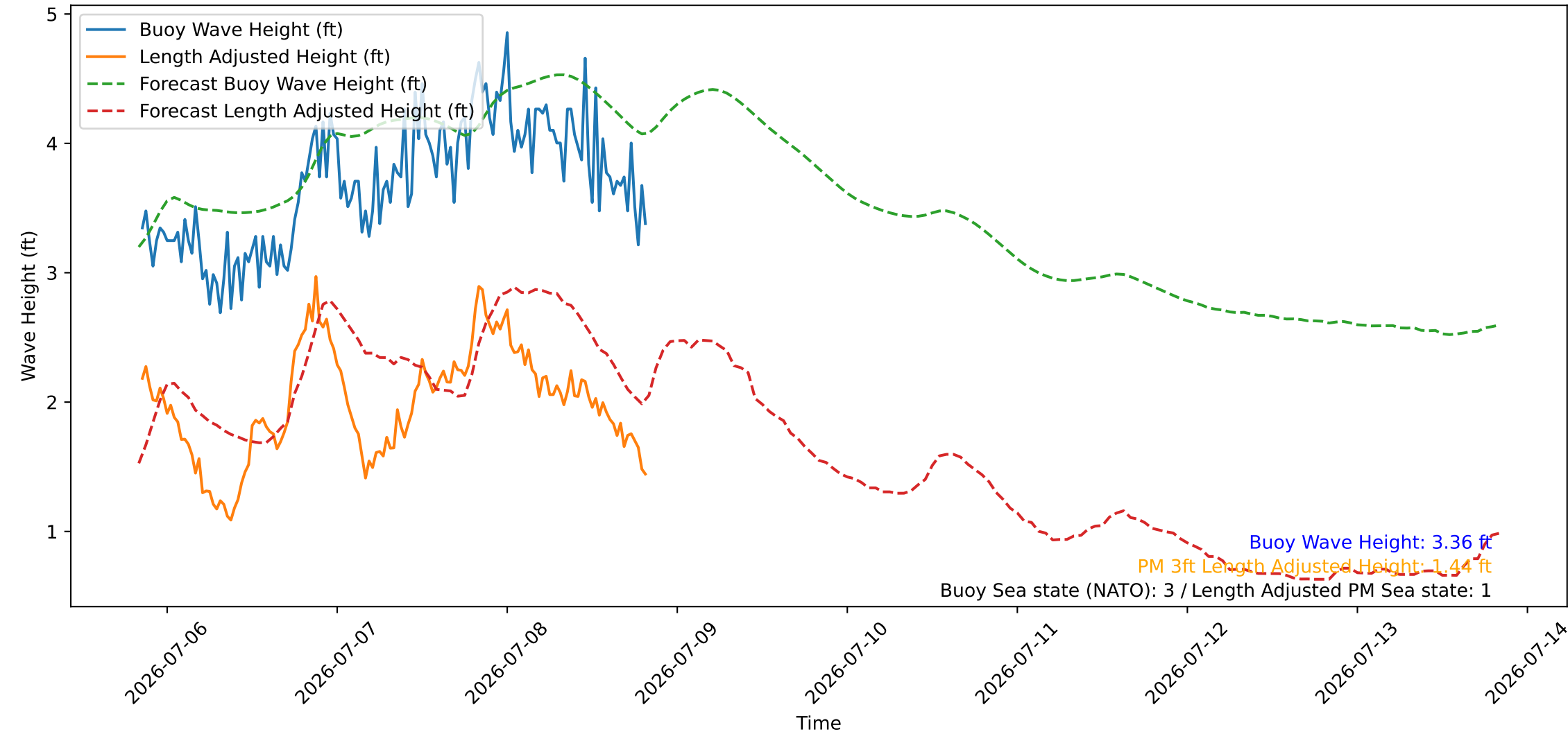
Wave Heights over Time for Red Beach at 2026-07-08 20:20:46
