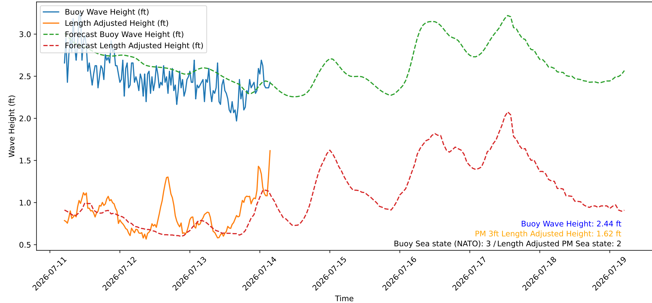
Wave Heights over Time for Red Beach at 2026-07-14 04:30:47
