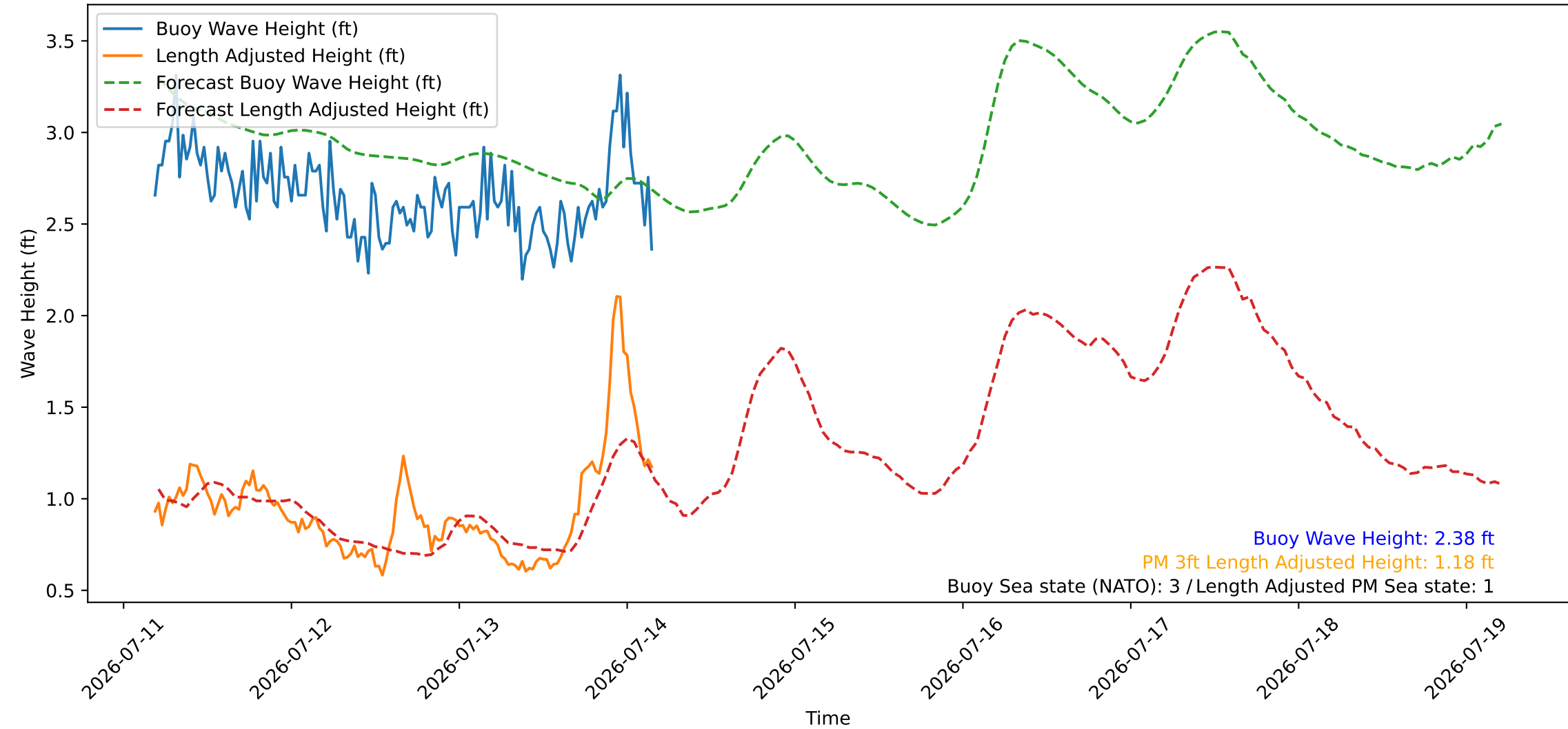
Wave Heights over Time for Green Beach at 2026-07-14 04:31:10
