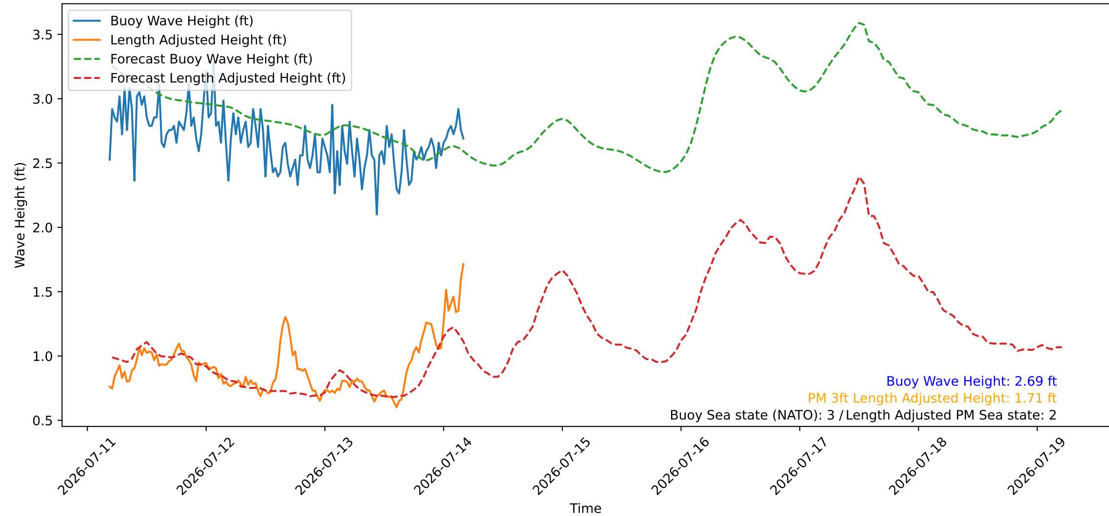
Wave Heights over Time for Oceanside Harbor at 2026-07-14 04:30:27
