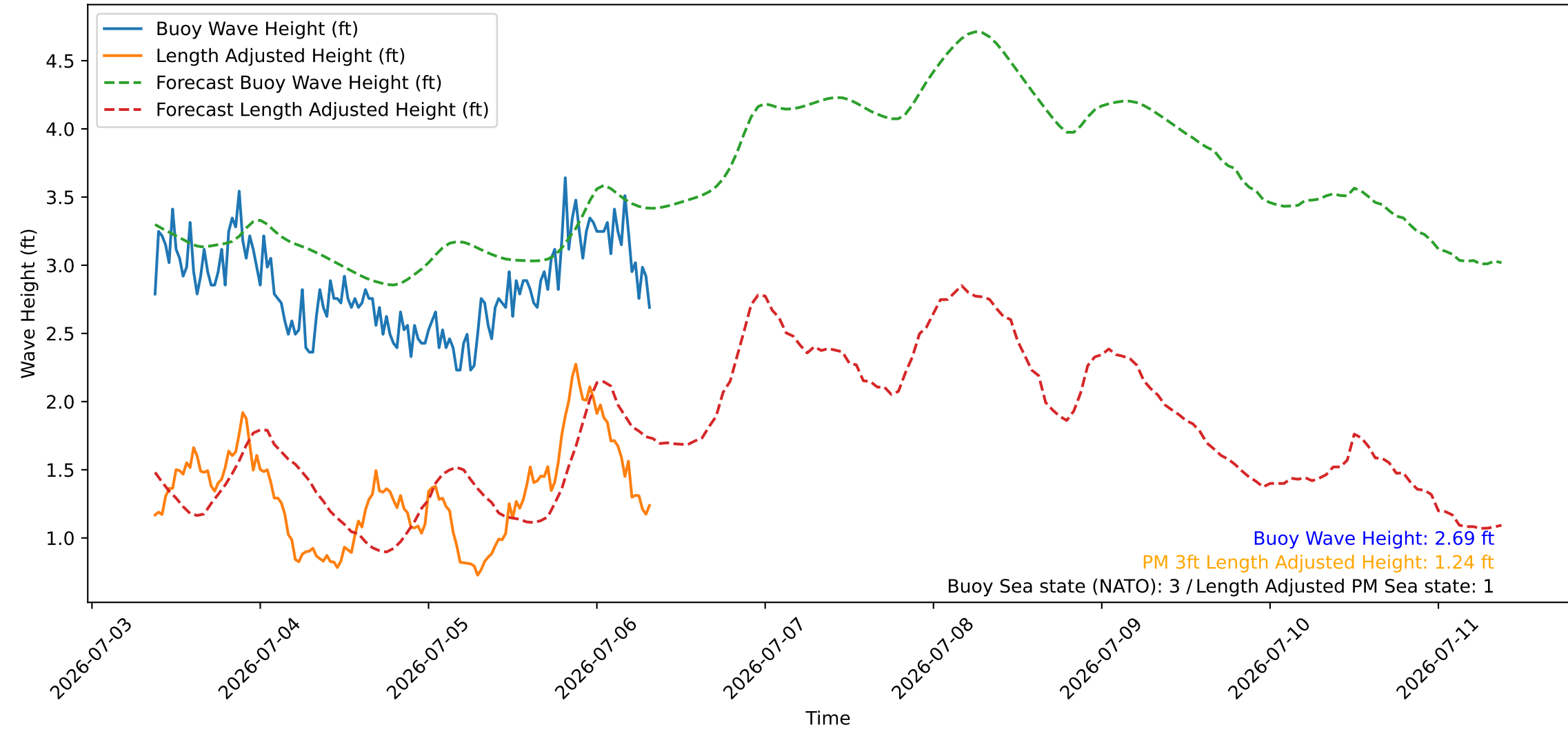
Wave Heights over Time for Red Beach at 2026-07-06 08:30:47
