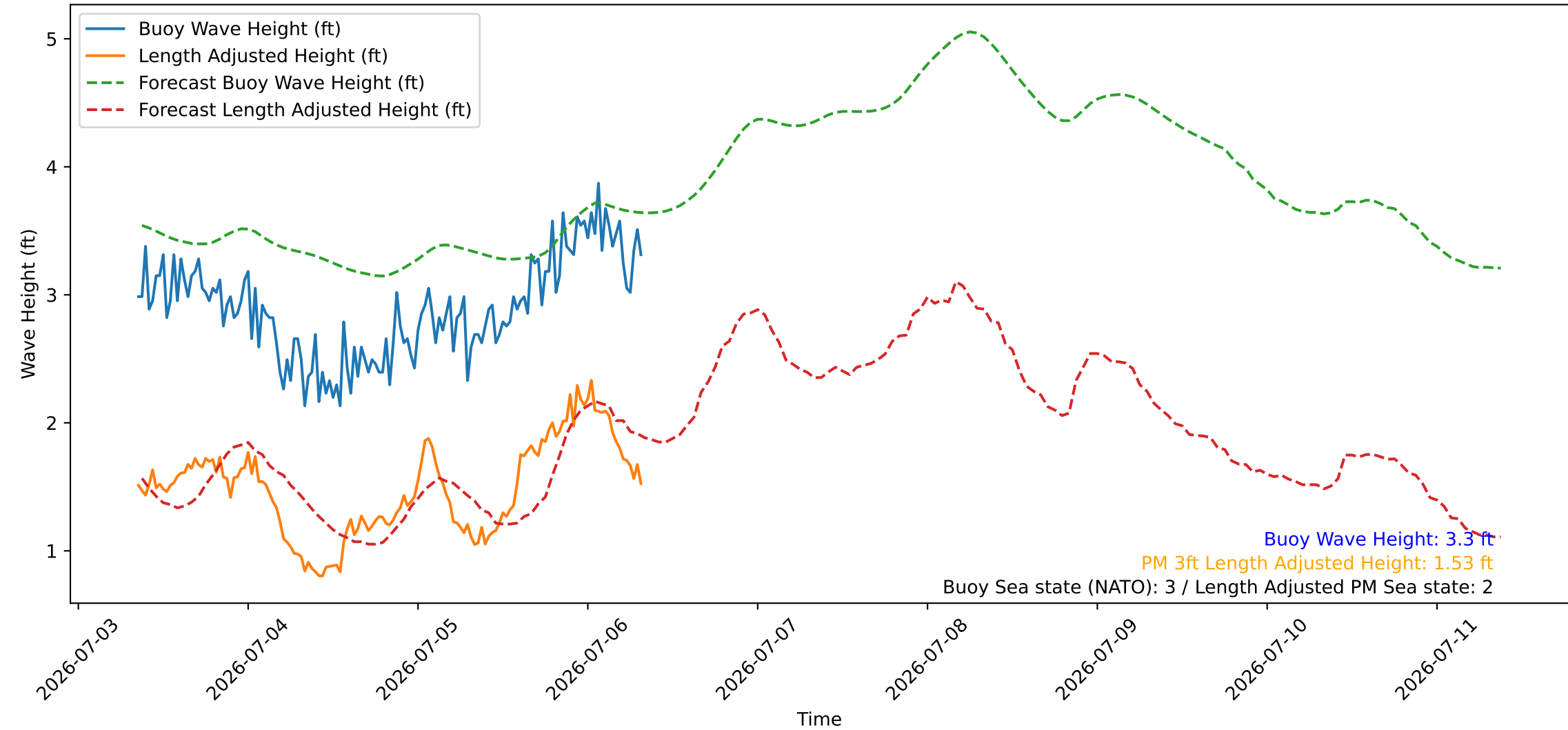
Wave Heights over Time for Oceanside Harbor at 2026-07-06 08:30:27
