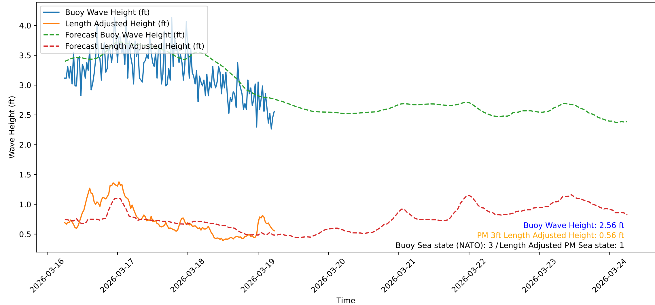
Wave Heights over Time for Green Beach at 2026-03-19 06:11:10
