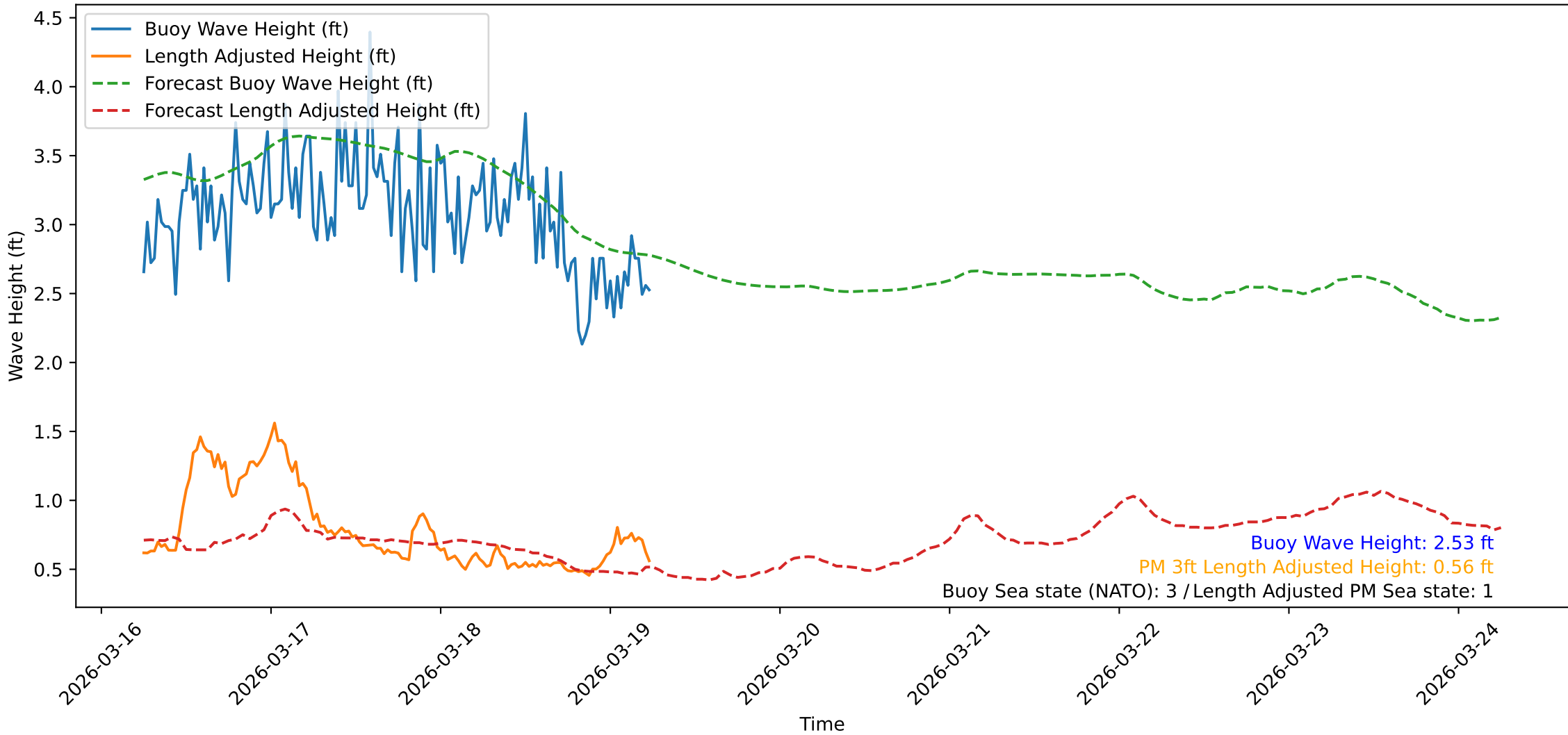
Wave Heights over Time for Oceanside Harbor at 2026-03-19 06:10:31
