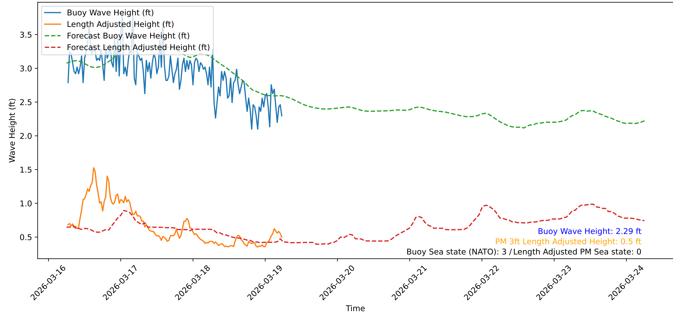
Wave Heights over Time for Red Beach at 2026-03-19 06:10:48
