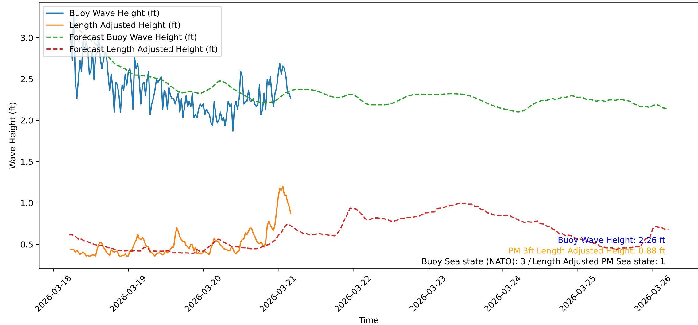
Wave Heights over Time for Red Beach at 2026-03-21 05:00:47
