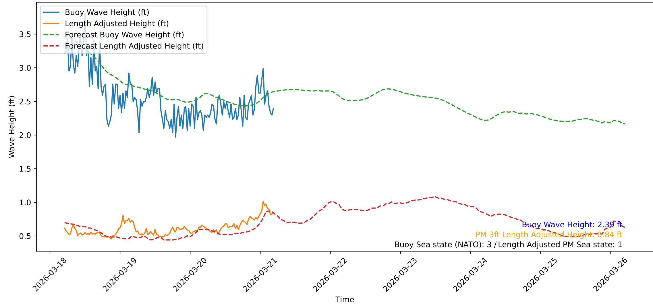
Wave Heights over Time for Oceanside Harbor at 2026-03-21 05:00:31
