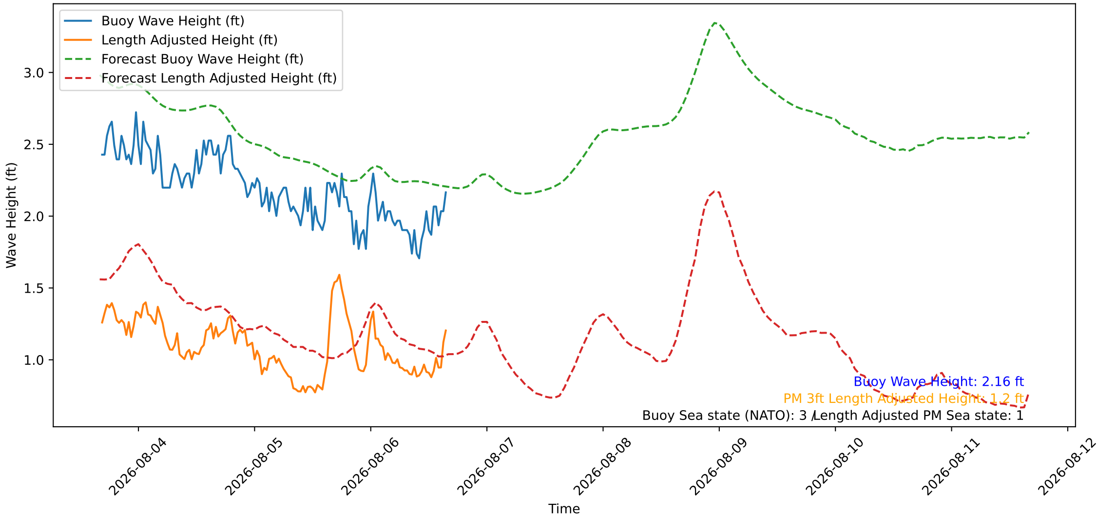
Wave Heights over Time for Oceanside Harbor at 2026-08-06 16:20:26
