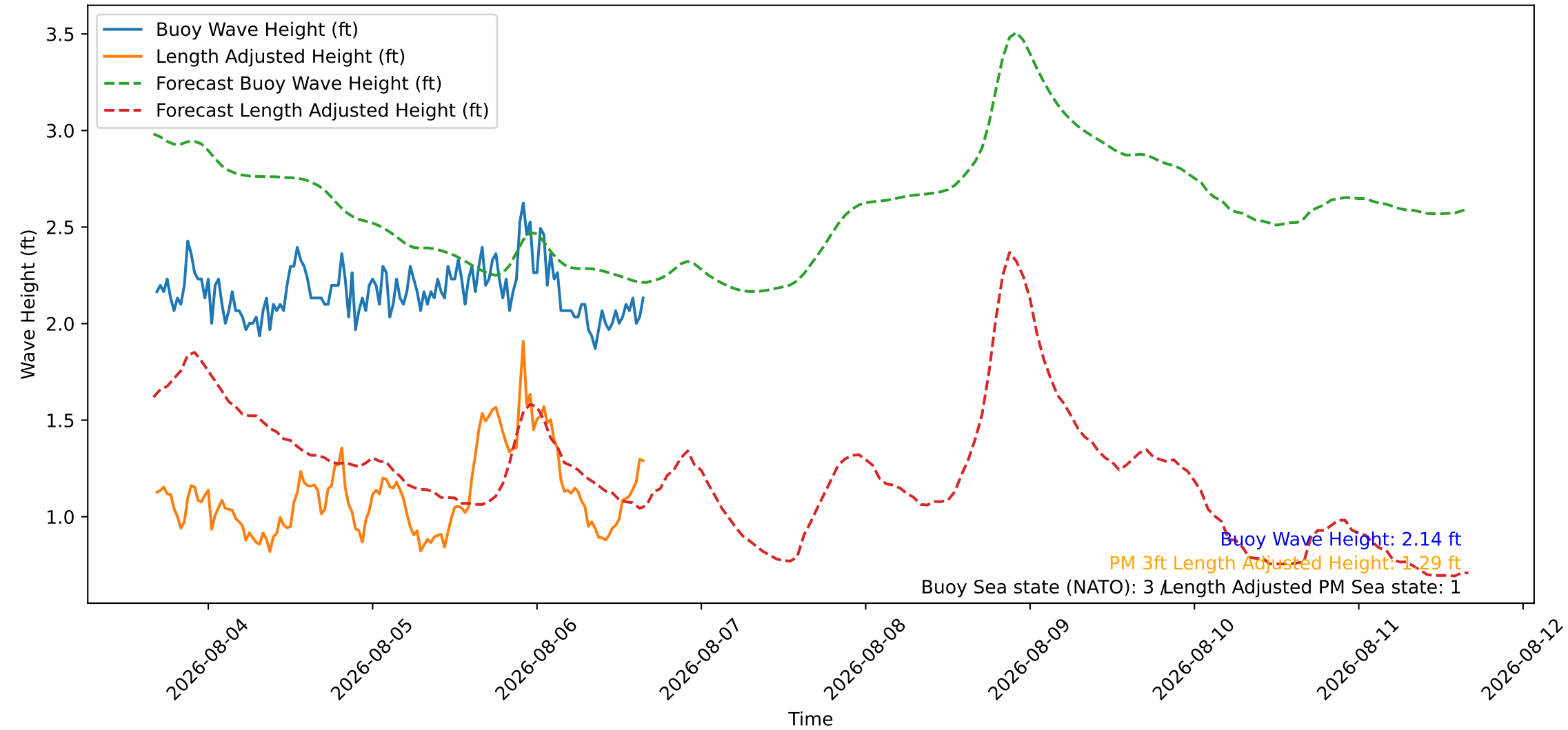
Wave Heights over Time for Green Beach at 2026-08-06 16:21:08
