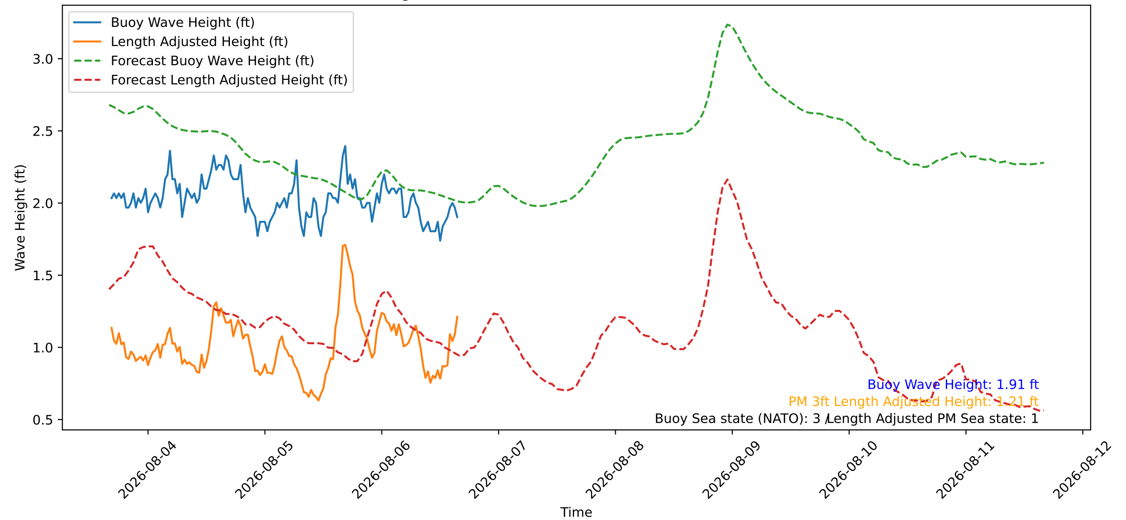
Wave Heights over Time for Red Beach at 2026-08-06 16:20:46
