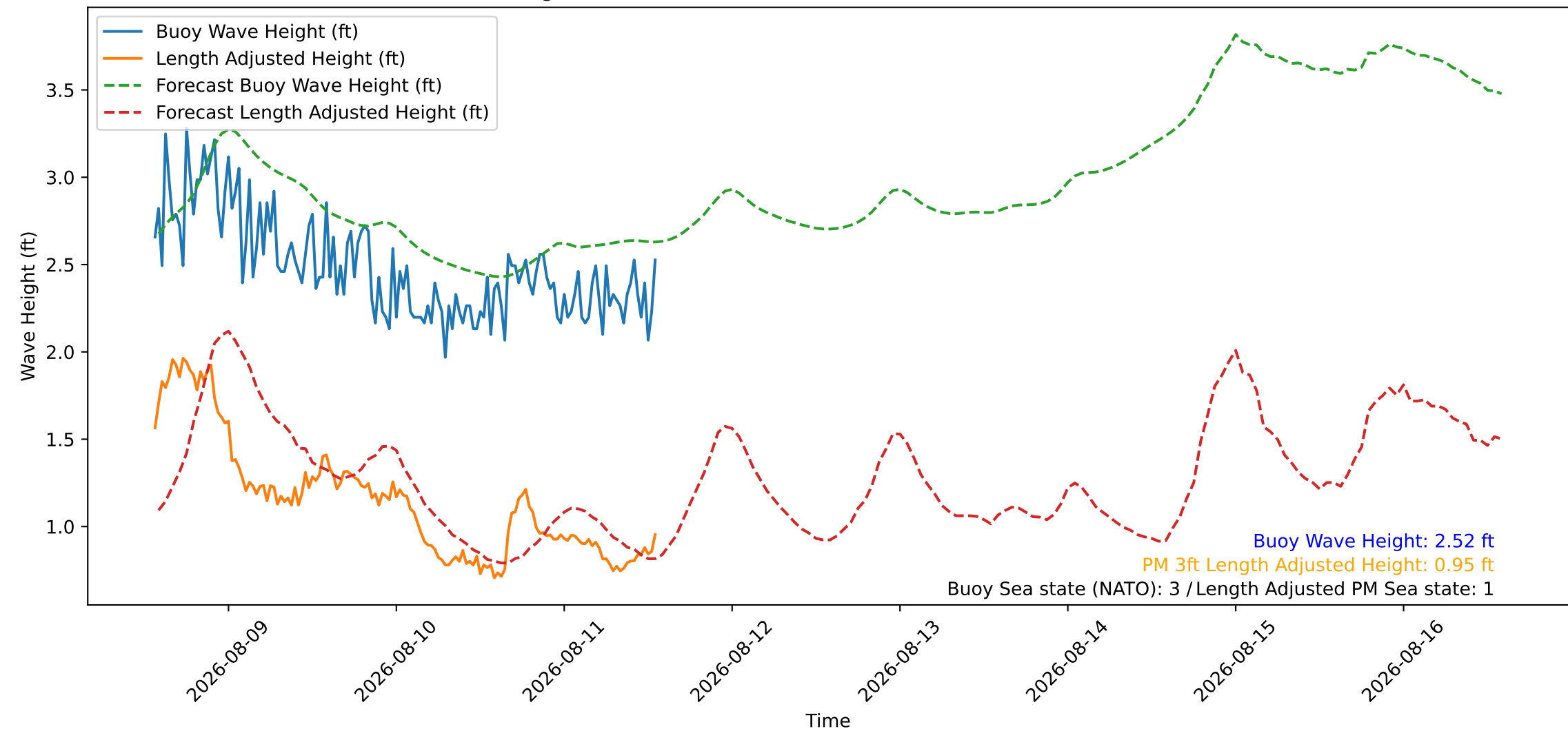
Wave Heights over Time for Oceanside Harbor at 2026-08-11 13:40:27
