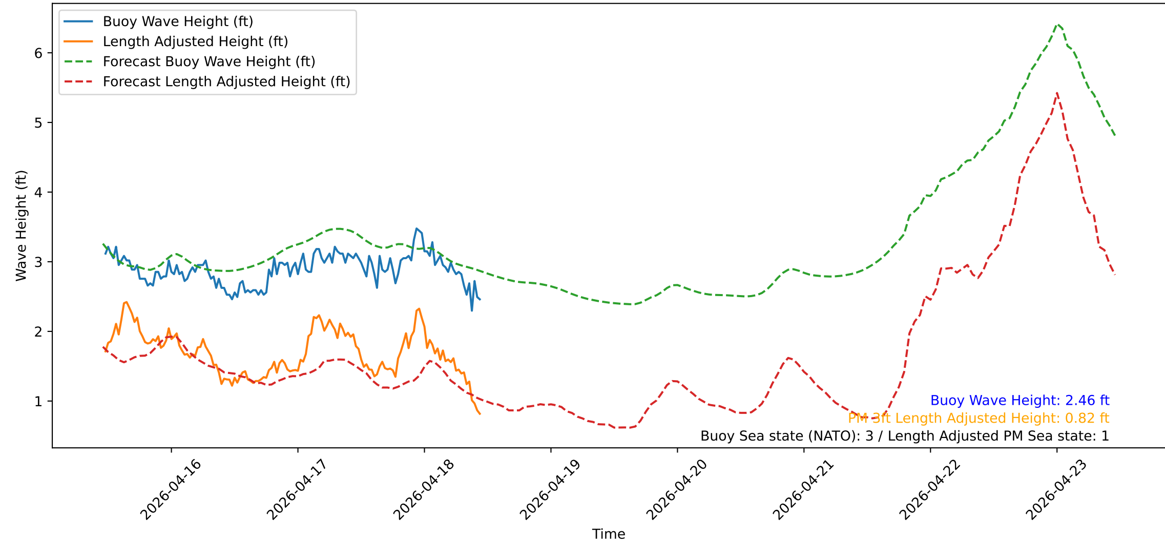
Wave Heights over Time for Green Beach at 2026-04-18 11:21:13
