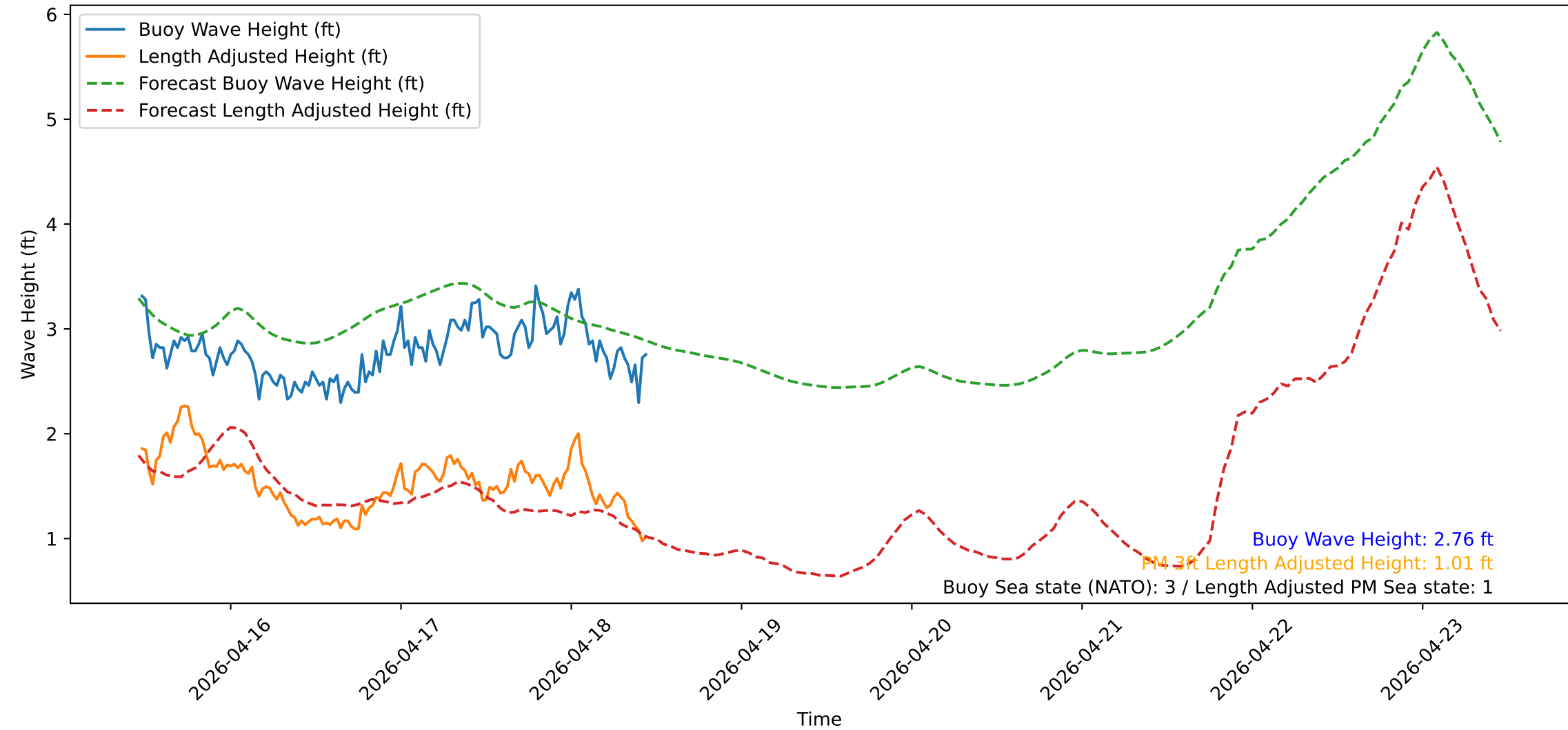
Wave Heights over Time for Oceanside Harbor at 2026-04-18 11:20:31
