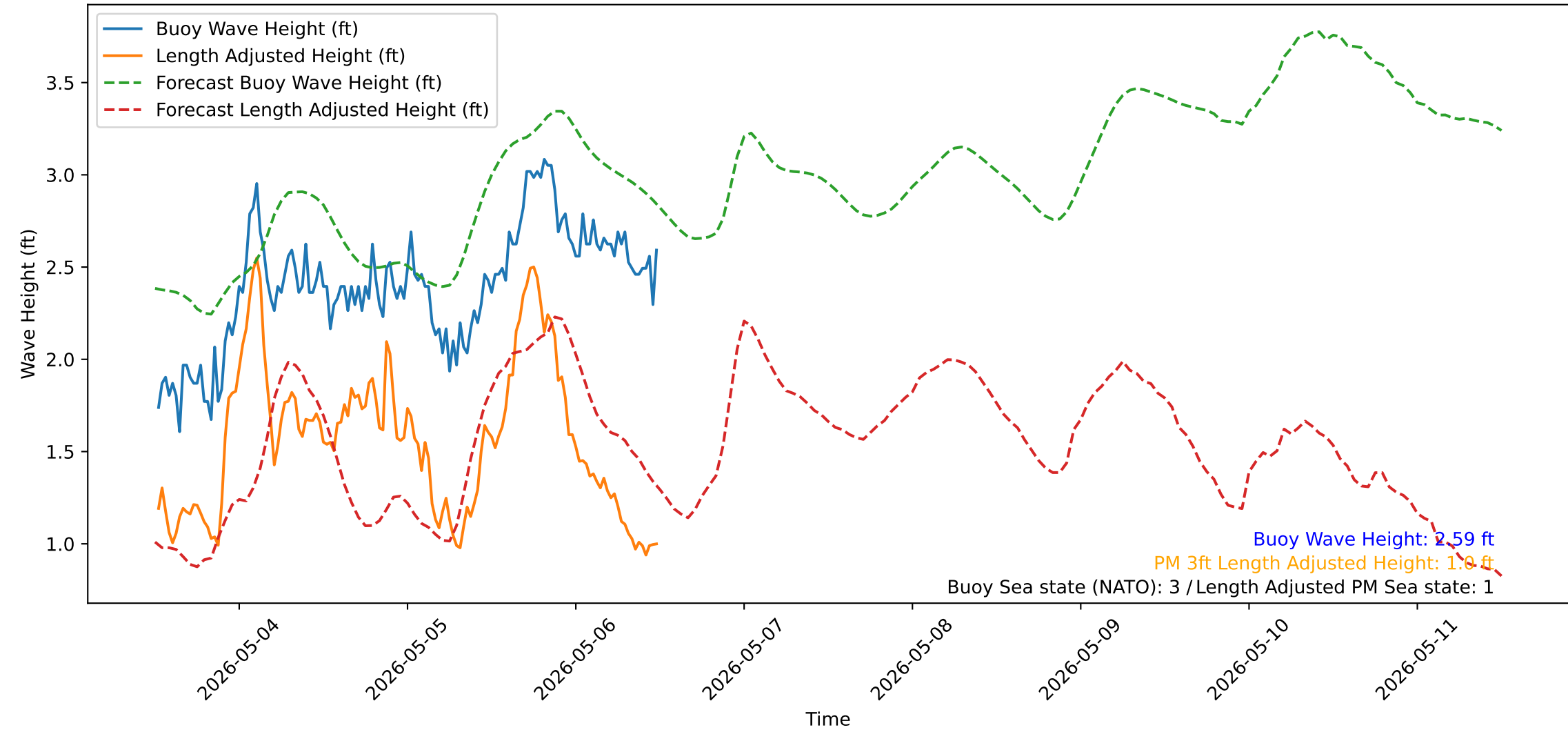
Wave Heights over Time for Red Beach at 2026-05-06 12:20:51
