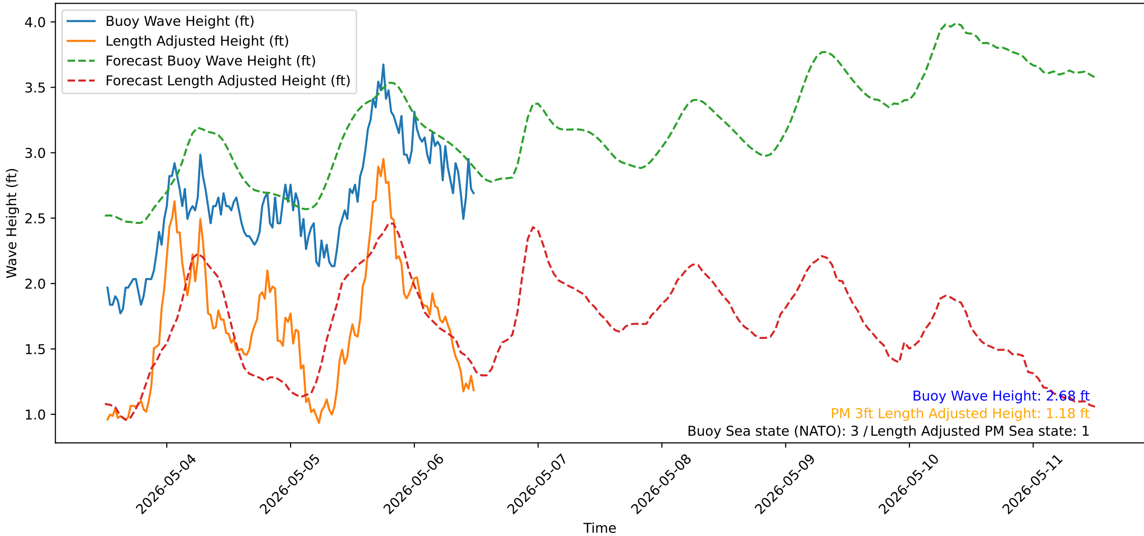
Wave Heights over Time for Green Beach at 2026-05-06 12:21:14
