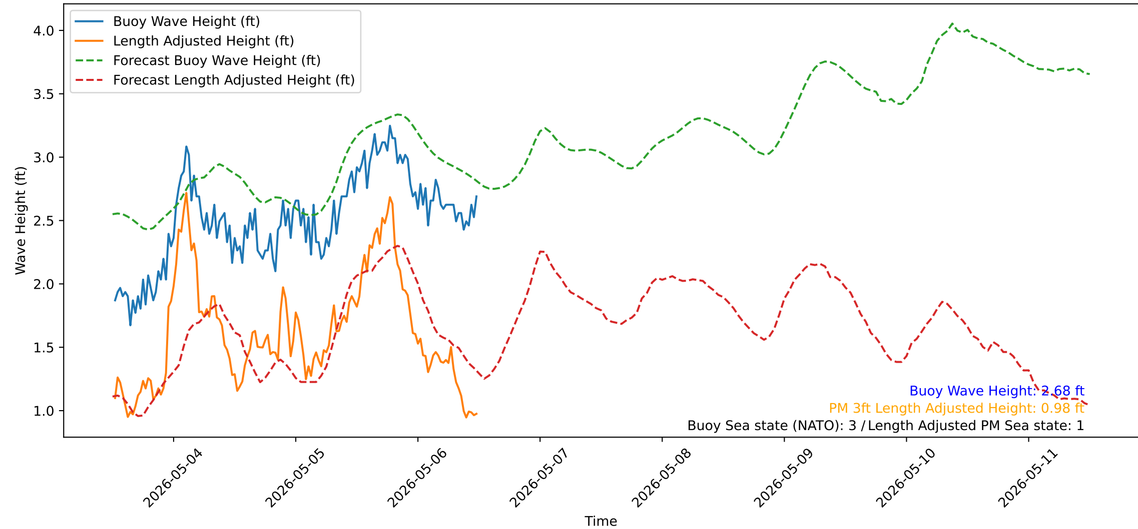
Wave Heights over Time for Oceanside Harbor at 2026-05-06 12:20:31
