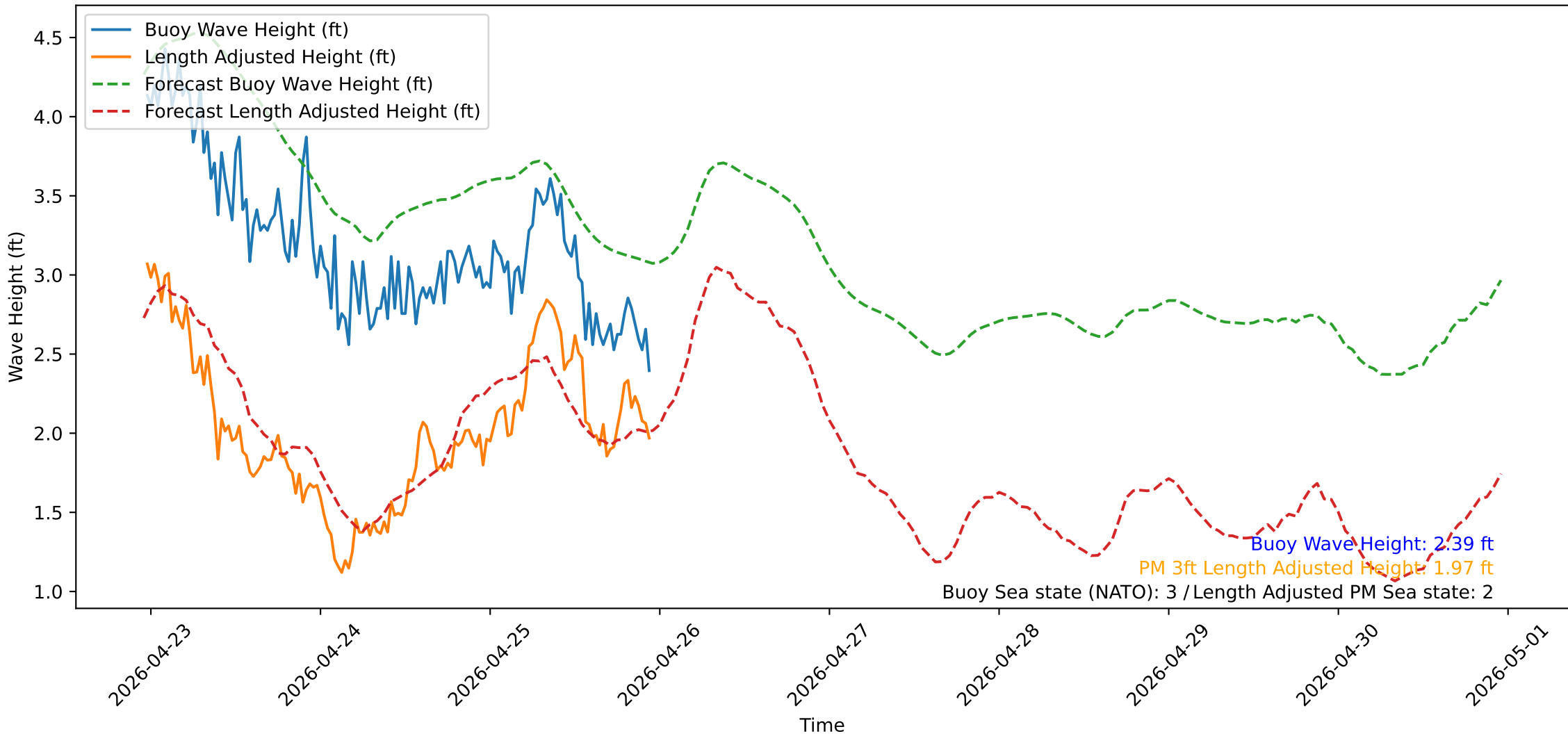
Wave Heights over Time for Oceanside Harbor at 2026-04-25 23:20:31
