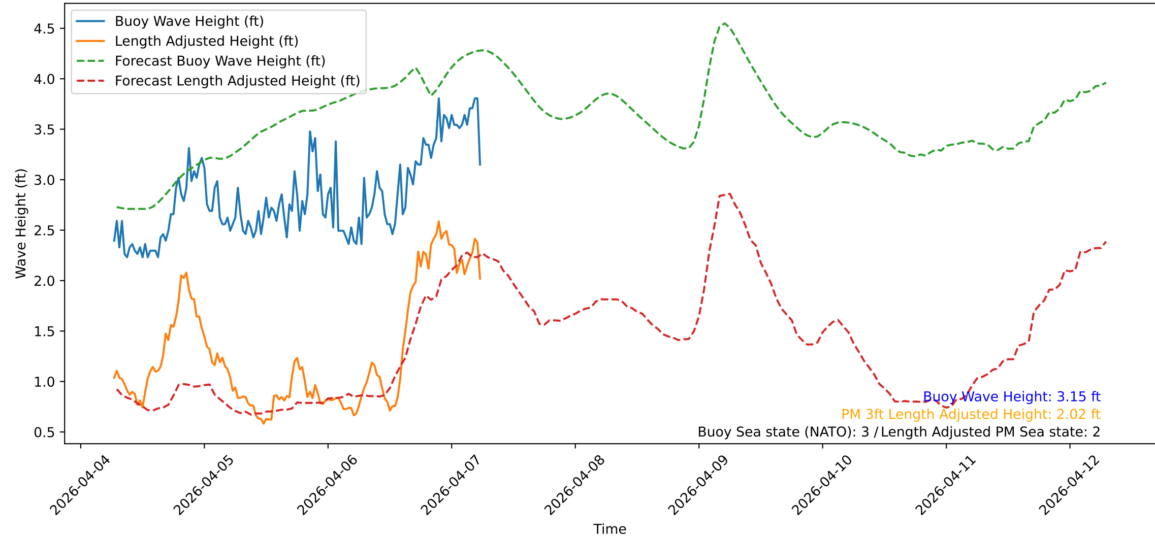
Wave Heights over Time for Green Beach at 2026-04-07 06:31:10
