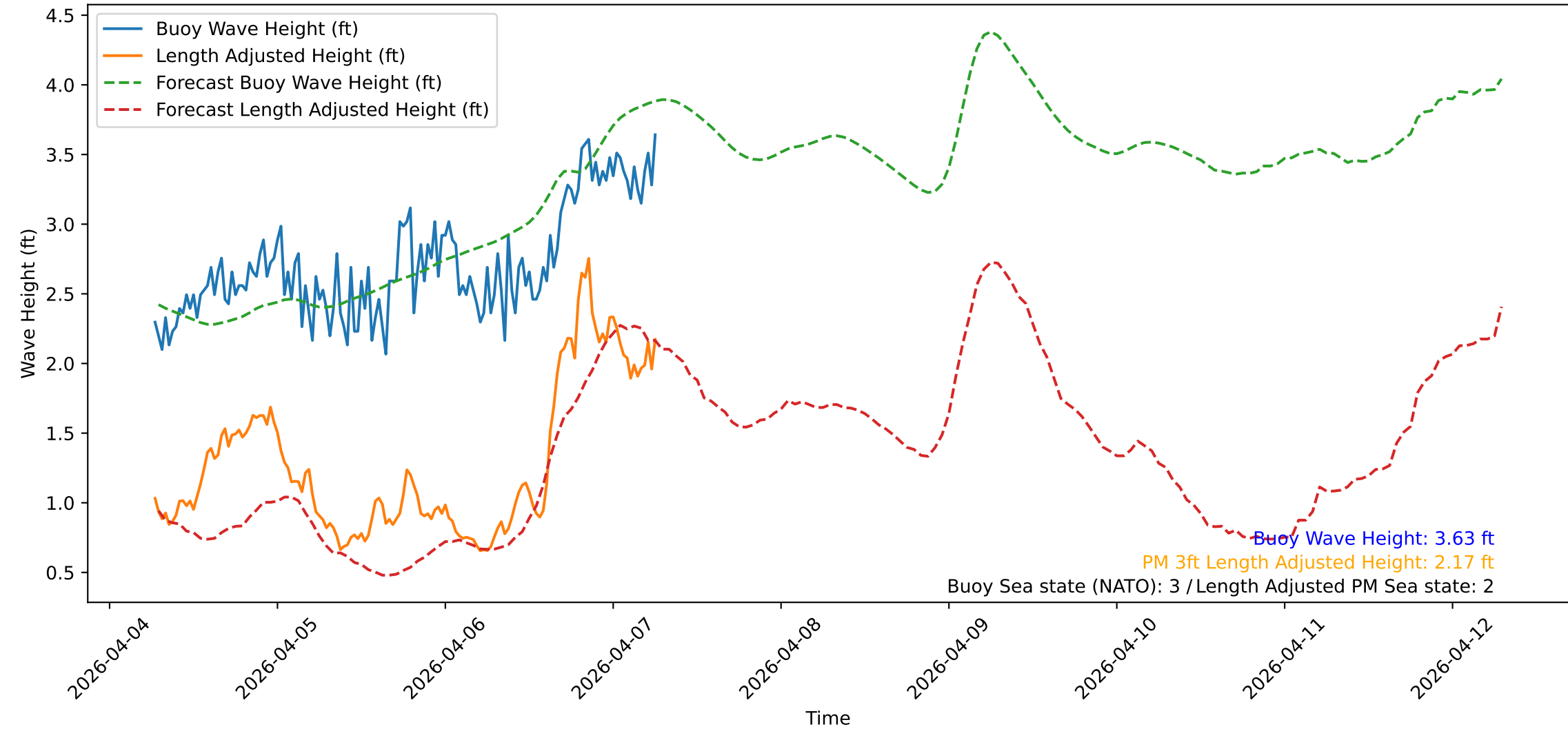
Wave Heights over Time for Oceanside Harbor at 2026-04-07 06:30:32
