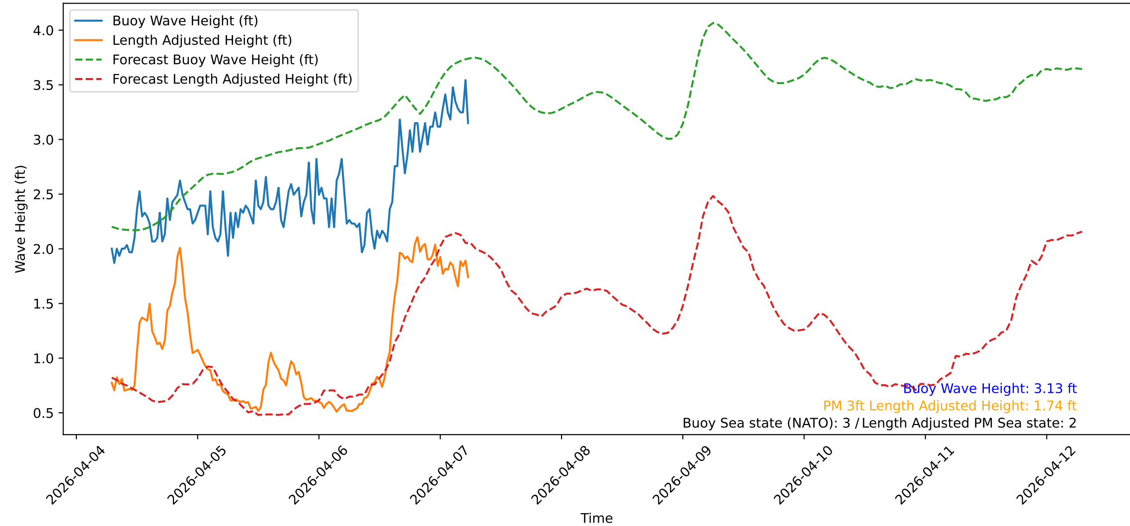
Wave Heights over Time for Red Beach at 2026-04-07 06:30:48
